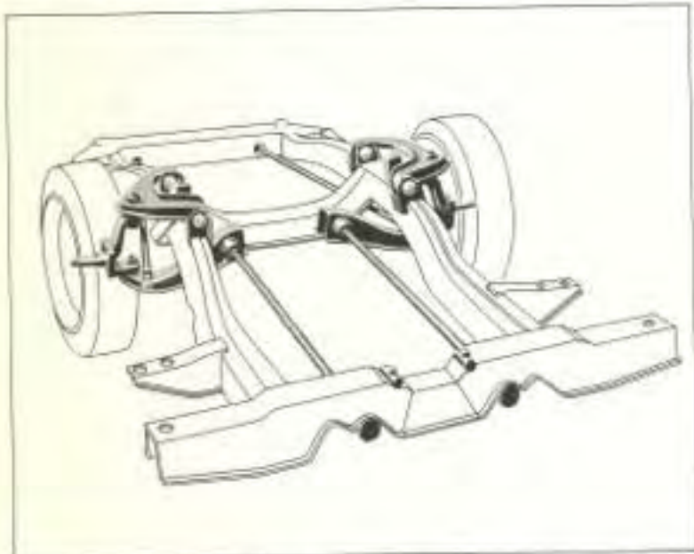
Torsion bars team up with 60-inch outrigger springs, heavy-duty shock absorbers and a low center of gravity to deliver level, balanced ride.
