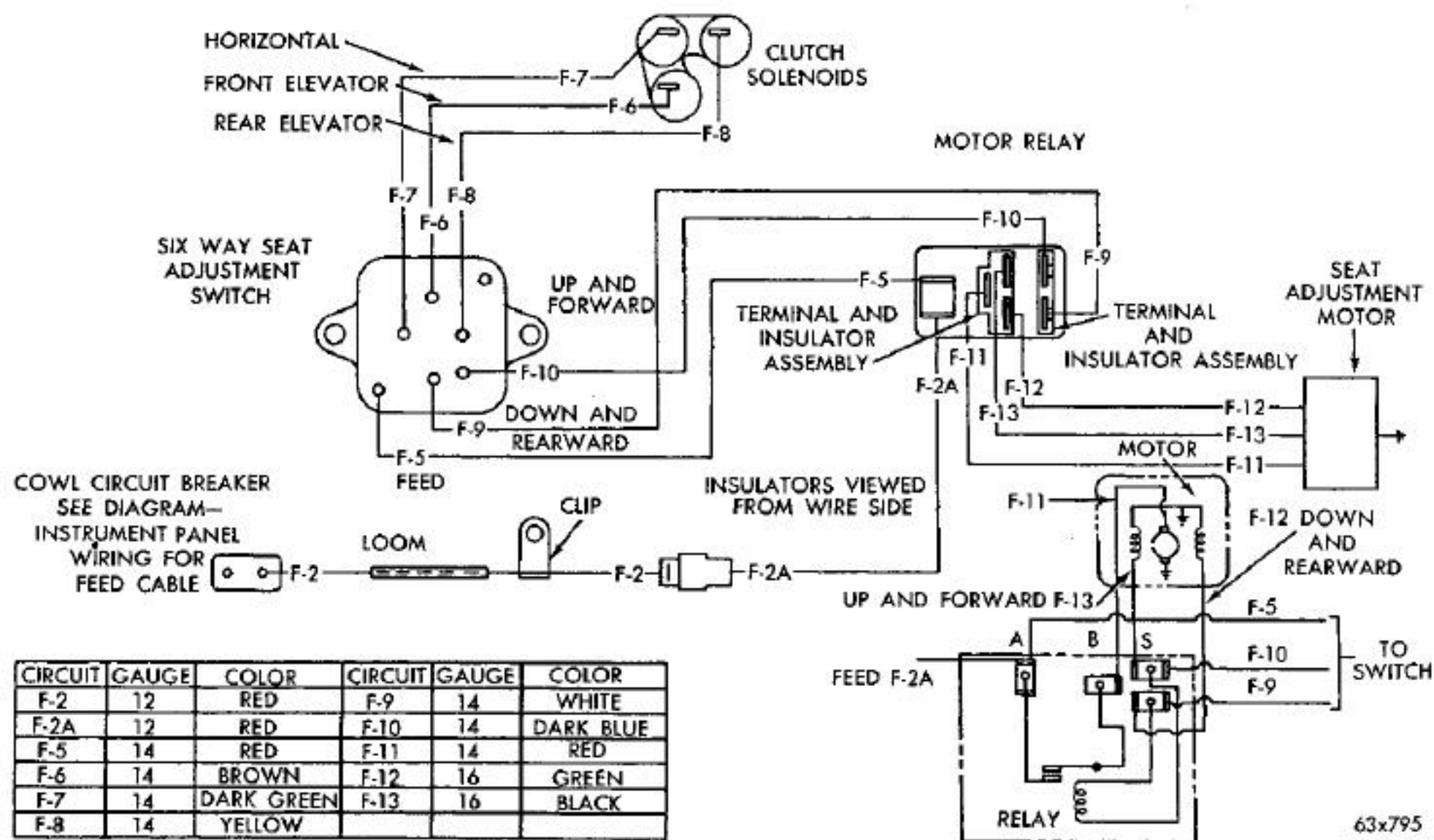
Fig. 138—Six Way Seat Adjusting
