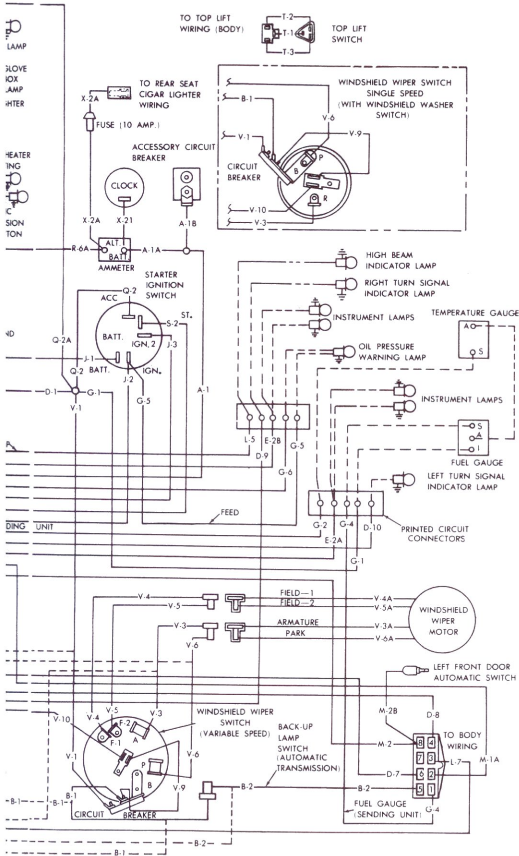
Instrument Panel Wiring—
