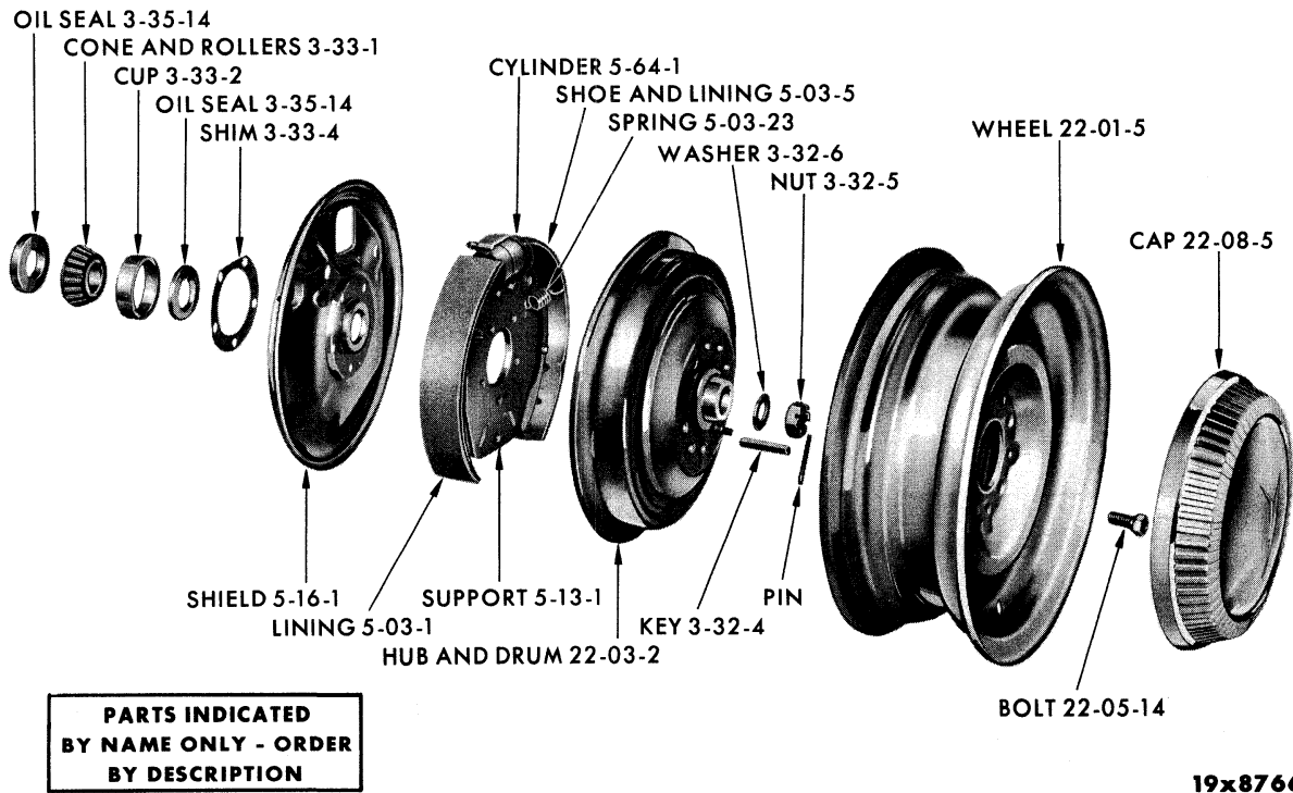
REAR WHEEL
