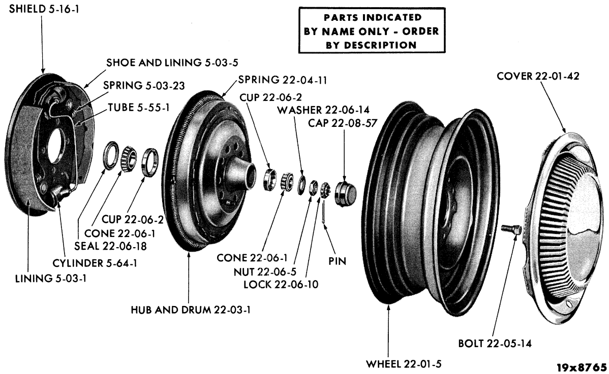
FRONT WHEEL
