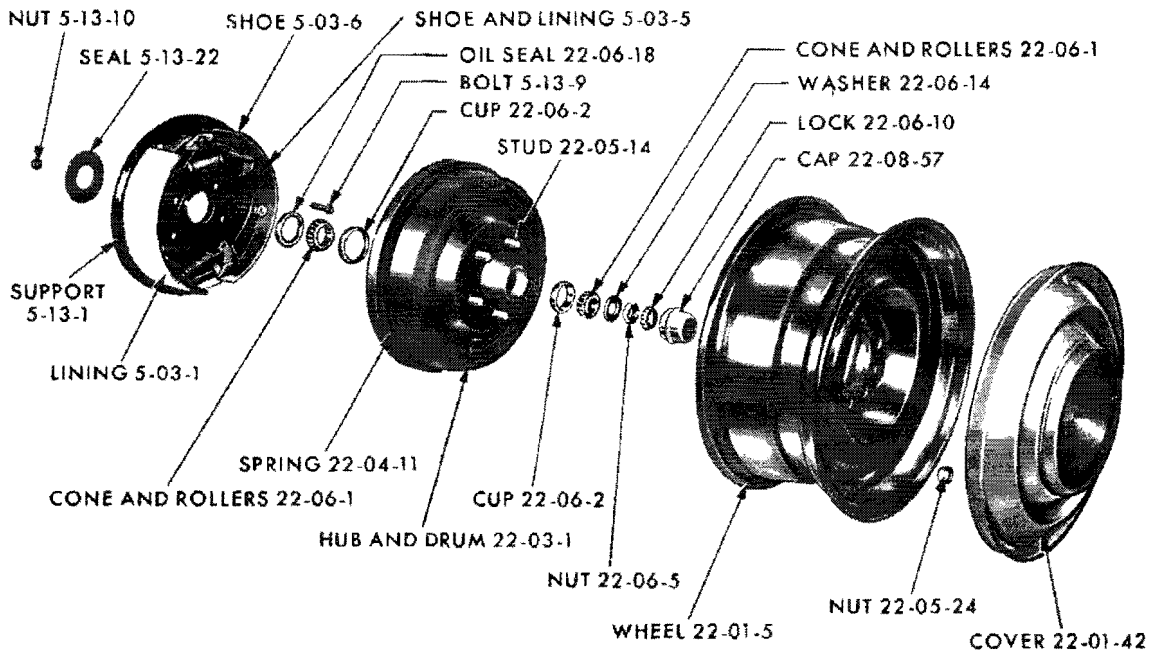
FRONT WHEEL
