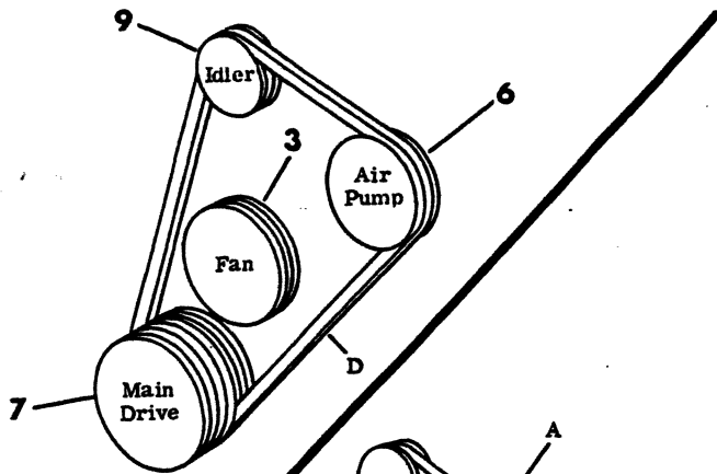
W/AIR PUMP 1979-80
