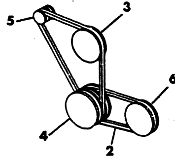
W/PWR STRG
