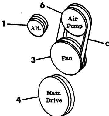
W/AIR PUMP 1978
