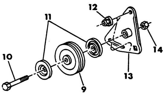
IDLER PULLEY
