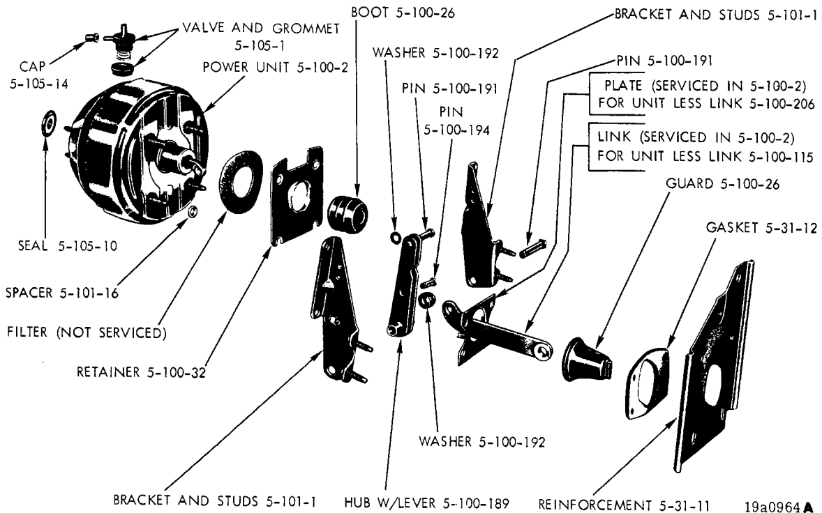
POWER BRAKE UNIT - BELVEDERE, CORONET, CHARGER, BARRACUDA AND CHALLENGER (WITH 480 ENGINE)
