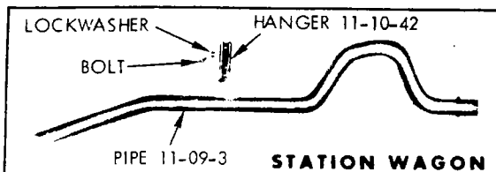
DUAL EXHAUST (383 AND 440 ENGINE) - PLYMOUTH FURY, DODGE (EXCEPT CORONET, CHARGER AND CHARGER R/T) AND CHRYSLER
