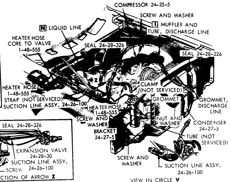
ROUTING FOR LEECE NEVILLE ALTERNATOR 19a3445
