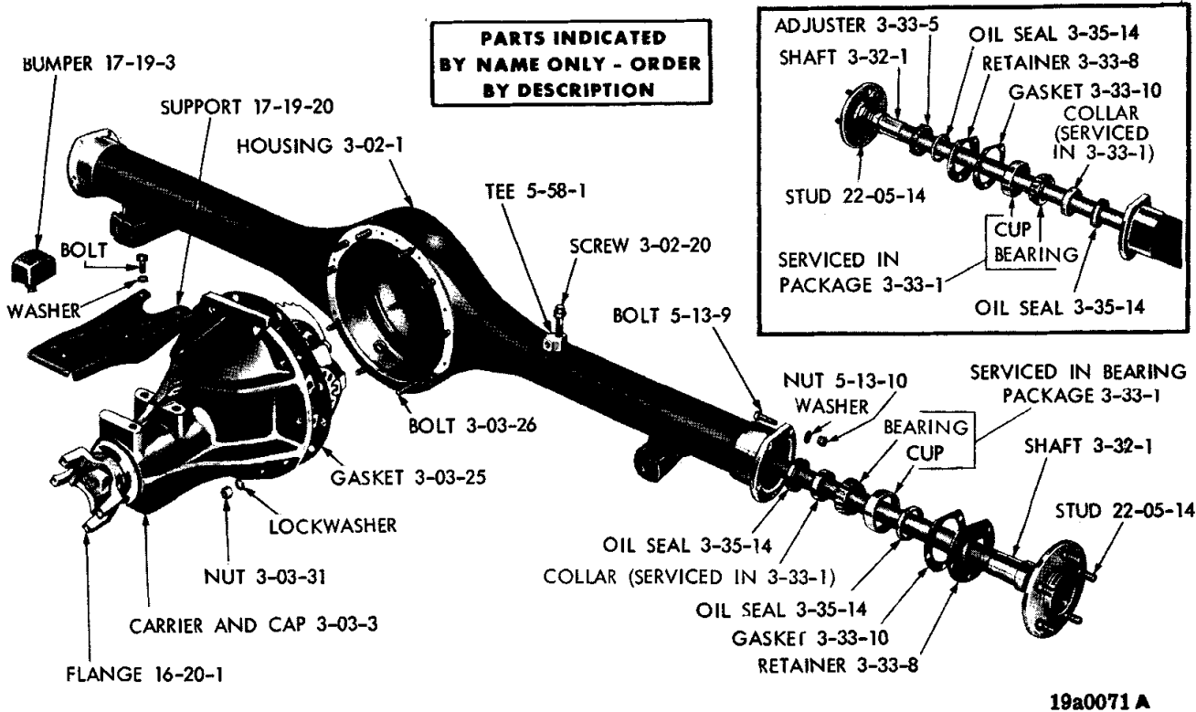
REAR AXLE HOUSING AND CARRIER - EXCEPT VALIANT AND DART
