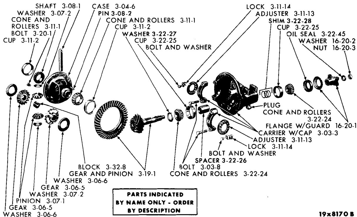
REAR AXLE DIFFERENTIAL - EXCEPT VALIANT AND DART
