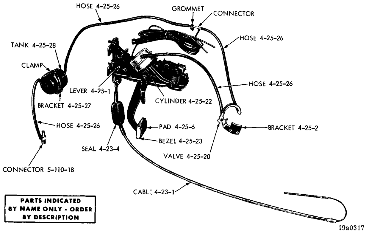
PARKING BRAKE SYSTEM (VACUUM RELEASE) - IMPERIAL
