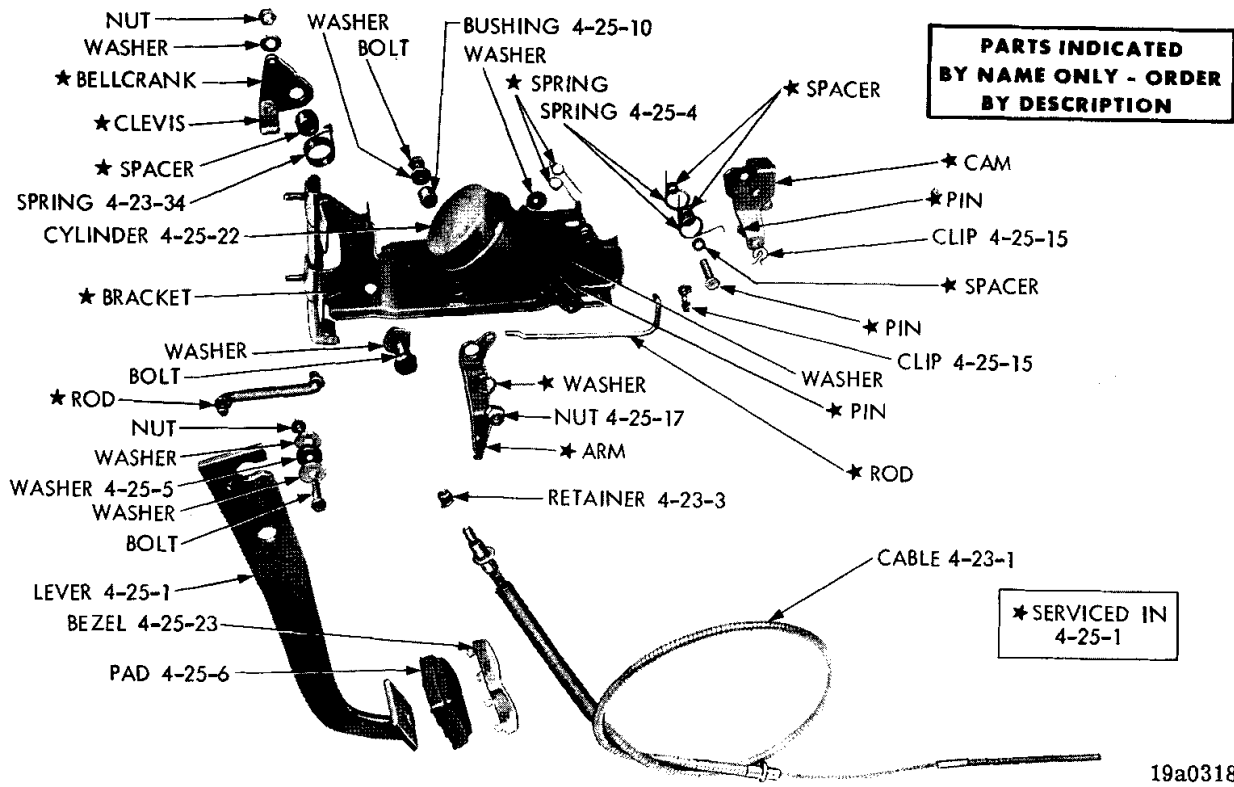
PARKING BRAKE (VACUUM RELEASE) - IMPERIAL
