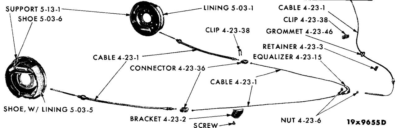
PARKING BRAKE SYSTEM - VALIANT, DART, BELVEDERE AND CORONET
