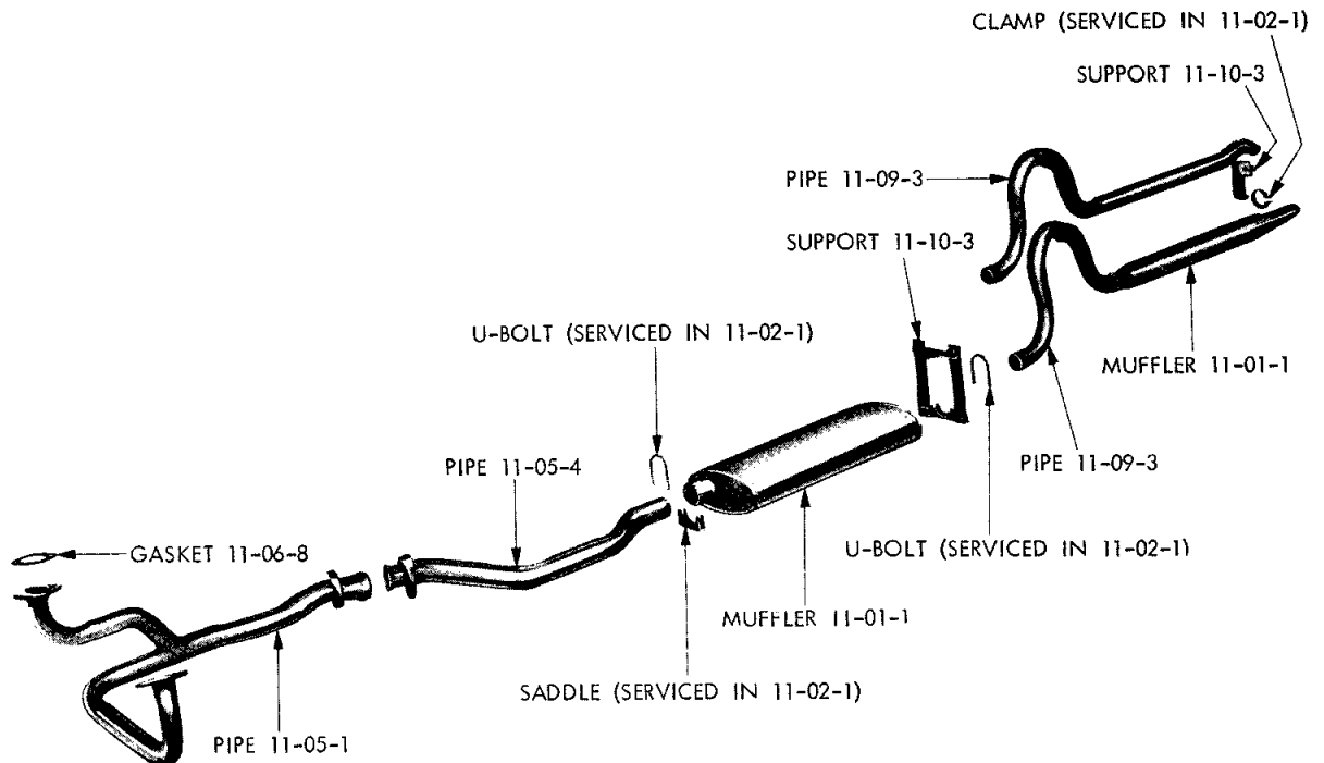
SINGLE EXHAUST SYSTEM (V8 CYLINDER - "B" ENGINE) - PLYMOUTH FURY, DODGE POLARA AND CHRYSLER
