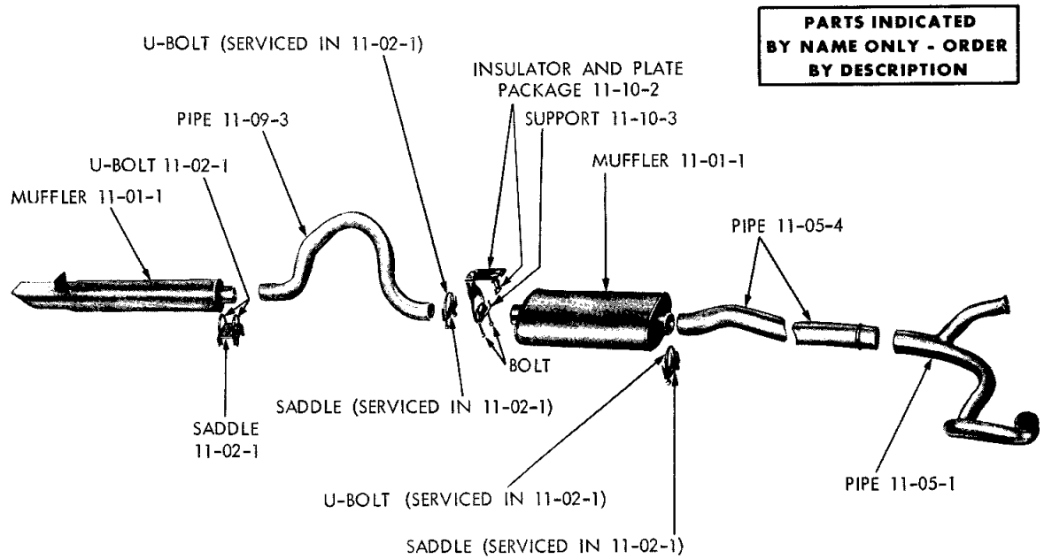
SINGLE EXHAUST SYSTEM (V8 CYLINDER) - VALIANT AND DART WITH POWER PACK, 1-4 BARREL CARBURETOR
