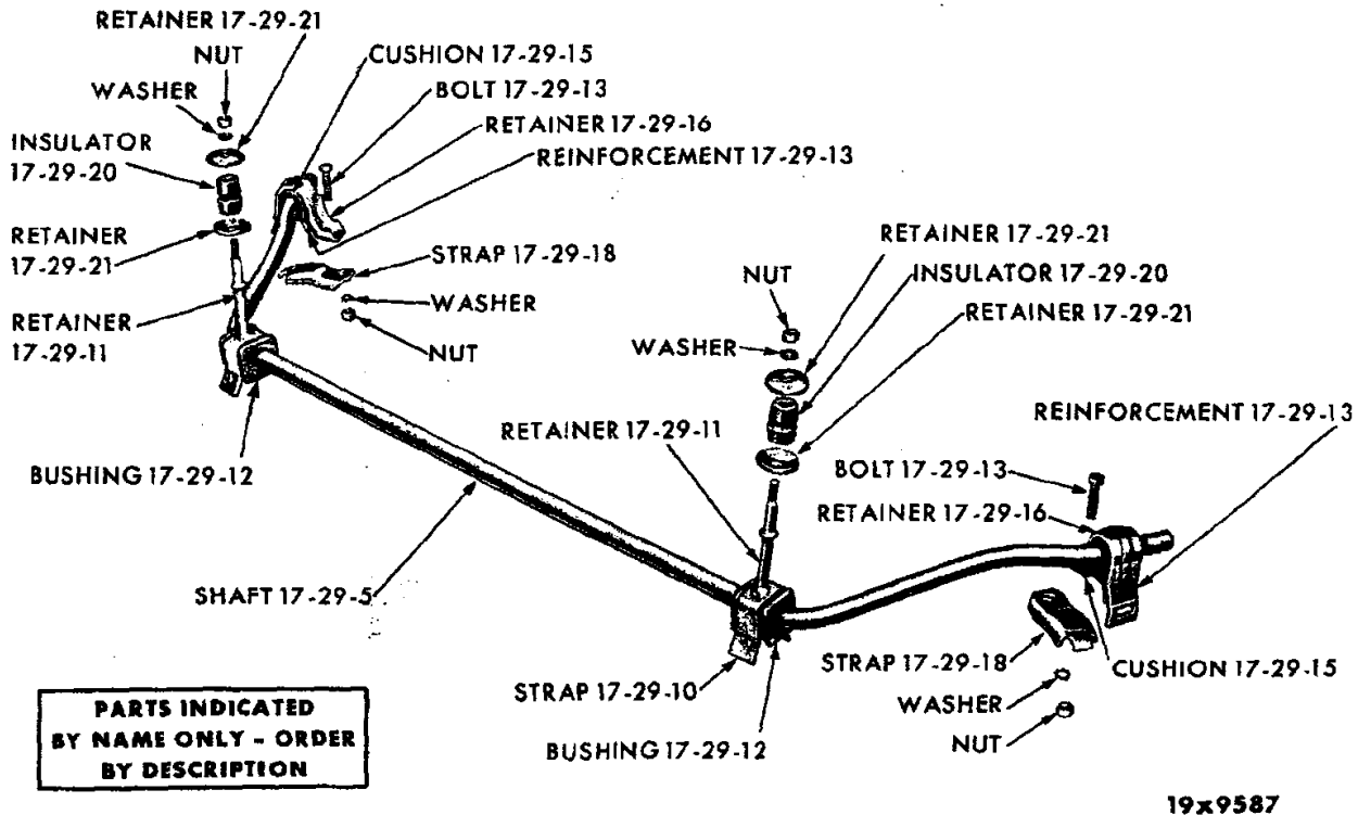
SWAY ELIMINATOR - DODGE VA3 AND CHRYSLER VC1-2-3
