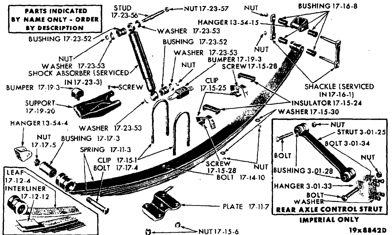
REAR SPRING - DODGE VA3, CHRYSLER VC1-2-3 AND IMPERIAL VY1
