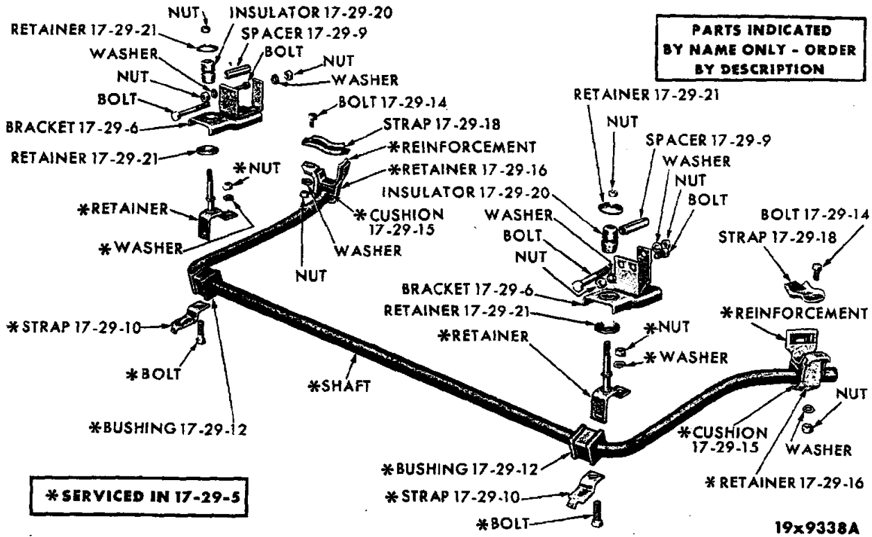
SWAY ELIMINATOR - PLYMOUTH VP1-2 AND DODGE VD1-2
