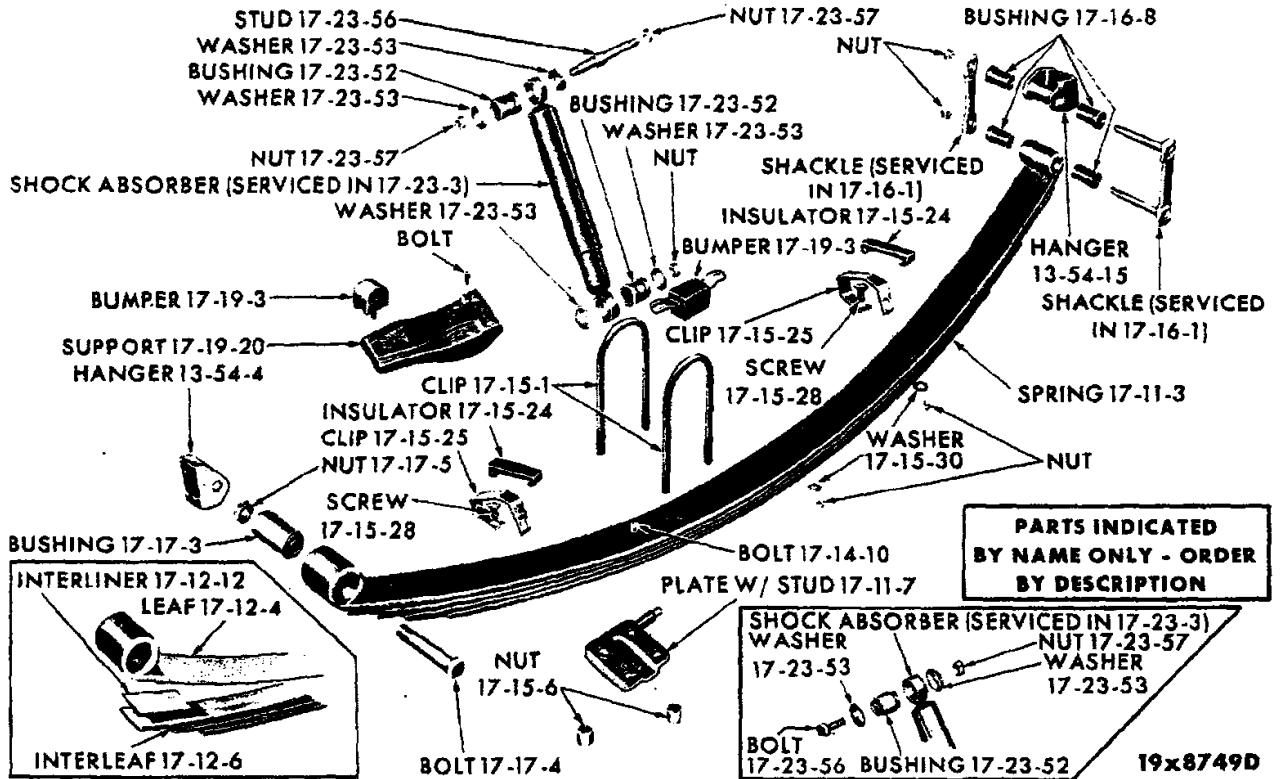
REAR SPRING - VALIANT VV1-2, DART VL1-2, PLYMOUTH VP1-2 AND DODGE VD1-2
