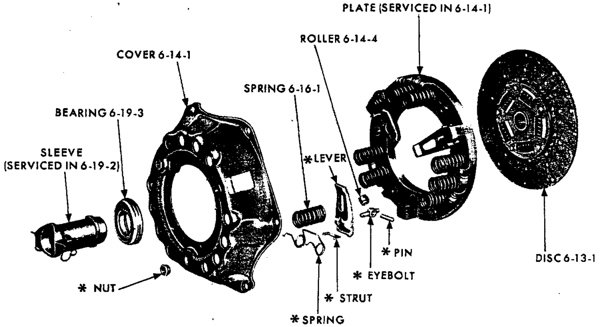
CLUTCH PRESSURE PLATE AND DISC
