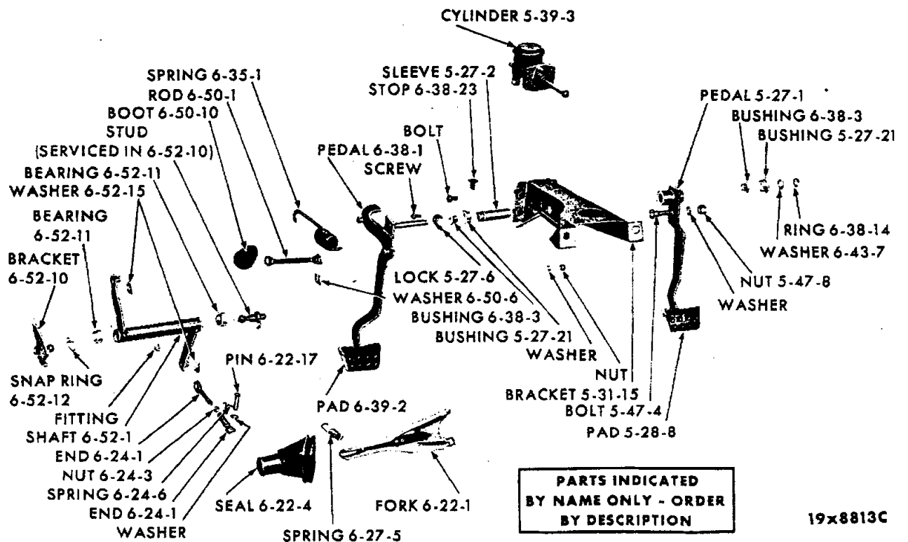
CLUTCH AND BRAKE PEDAL LINKAGE - VALIANT VV1-2 AND DART VL1-2 (WITH MANUAL TRANSMISSION)
