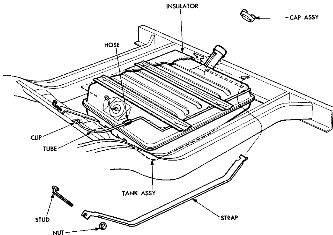
Fig. 81—Fuel Tank Mounting
