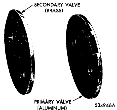
Fig. 44—Throttle Valve Identification
