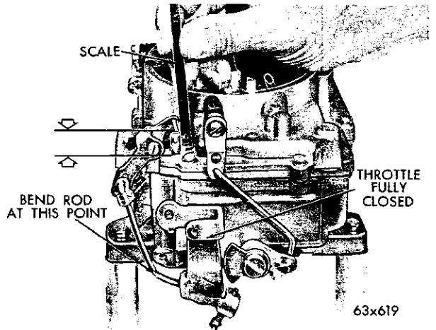
Fig. 75—Measuring the Accelerator Pump Travel
