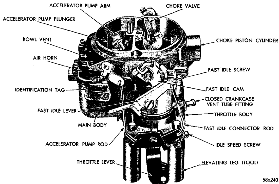
Fig. 22—Carburetor Assembly (BBD 3476S)
