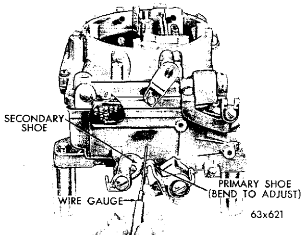
Fig. 77—Measuring the Clearance Between the Closing Shoes
