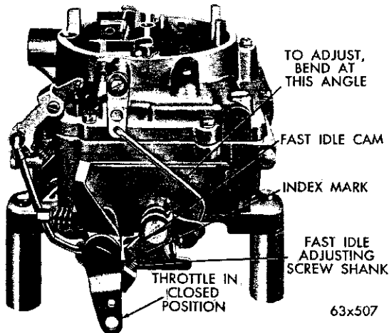
Fig. 55—Fast Idle Cam Indexing
