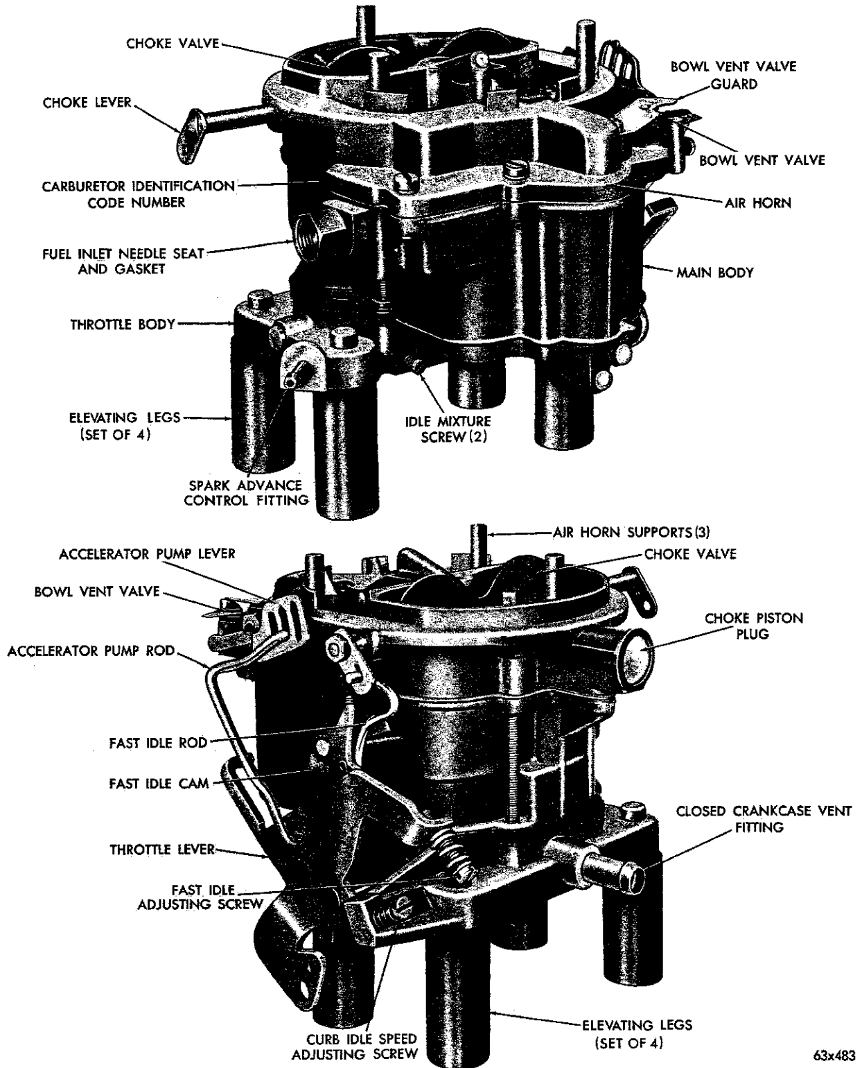
Fig. 1—Carburetor Assembly (WWC3)
