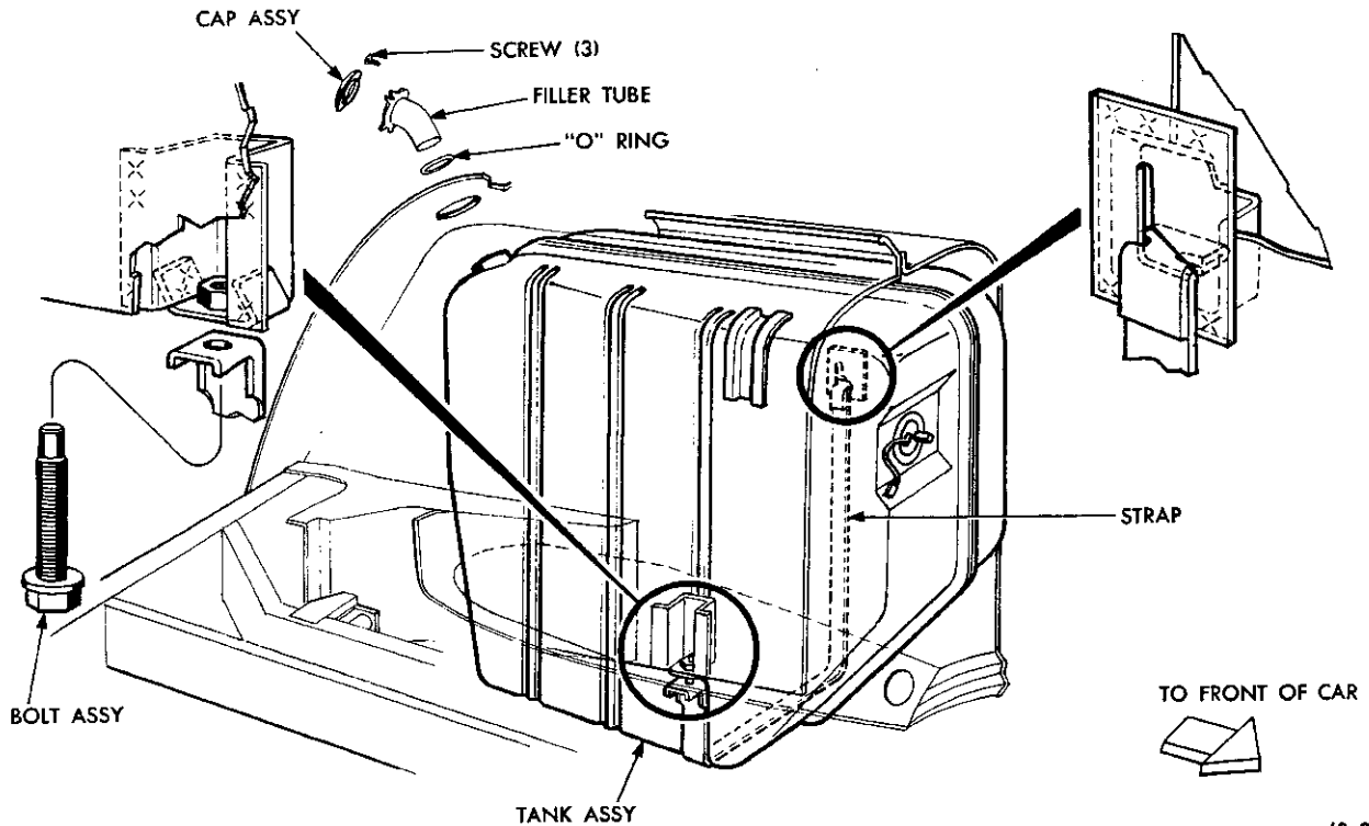
Fig. 82—Fuel Tank Mounting (Town and Country)
