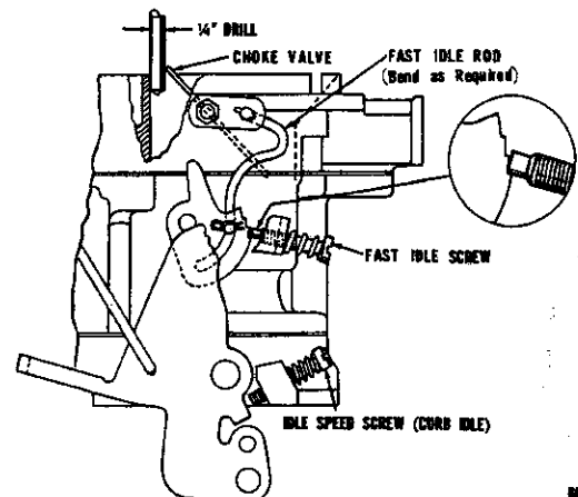
Fig. 18—Fast Idle Speed and Cam Position Setting
