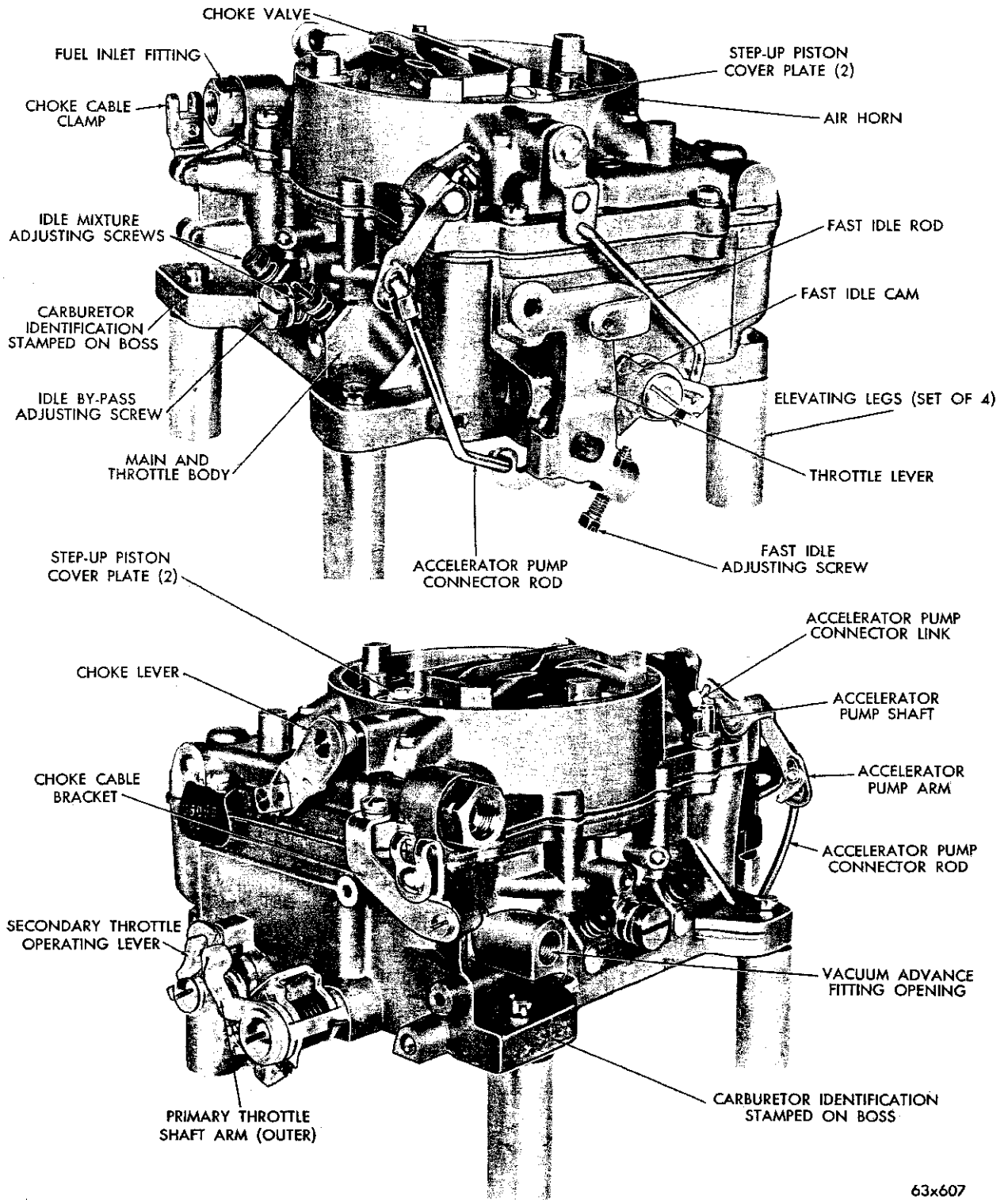
Fig. 61—Carburetor Assembly (AFB—3505S)
