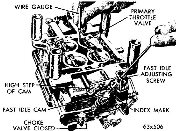
Fig. 49—Fast Idle Adjustment
