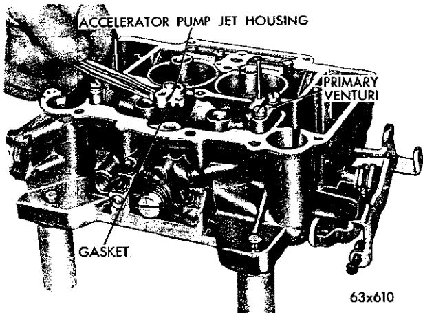
Fig. 63—Removing or Installing the Pump Jet Housing
