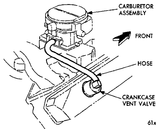
Fig. 35—Closed Crankcase Vent System
