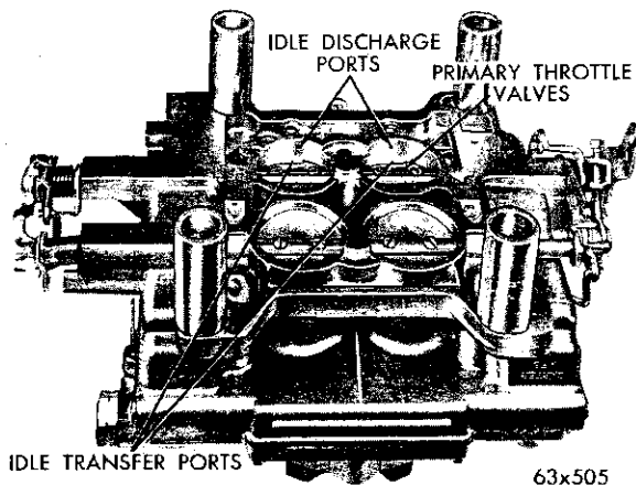
Fig. 43—Ports in Relation to Throttle Valves
