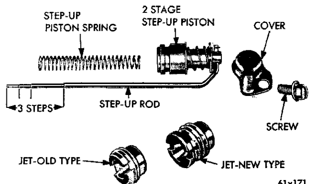
Fig. 48—Step-Up Piston, Rod and Jet
