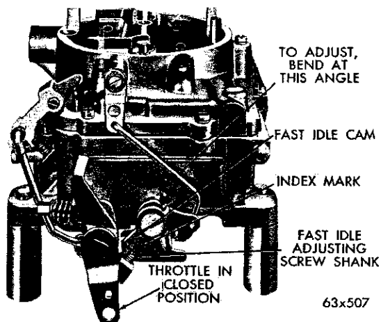
Fig. 50—Fast Idle Cam Indexing
