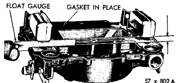
Fig. 73—Measuring the Float Height
