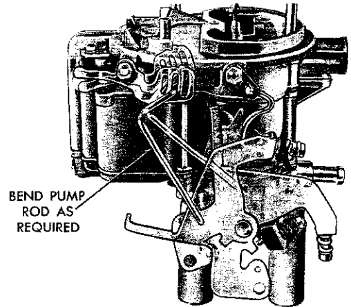
Fig. 20—Accelerator Pump Travel
