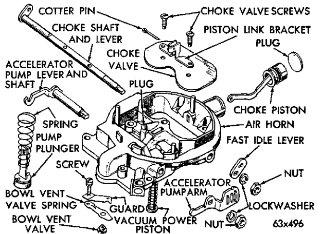
Fig. 16—Air Horn (Disassembled View)
