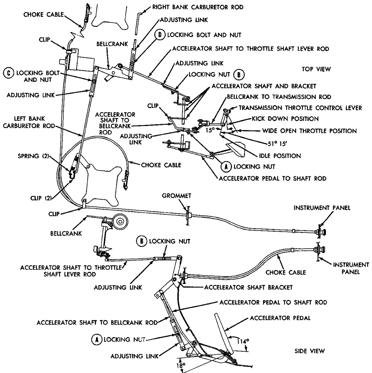
Fig. 60—Throttle Linkage C-300J (Schematic)
