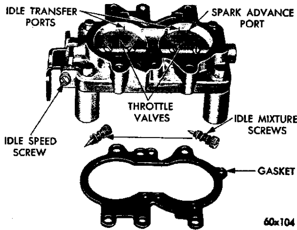
Fig. 26—Ports in Relation to Throttle Valves
