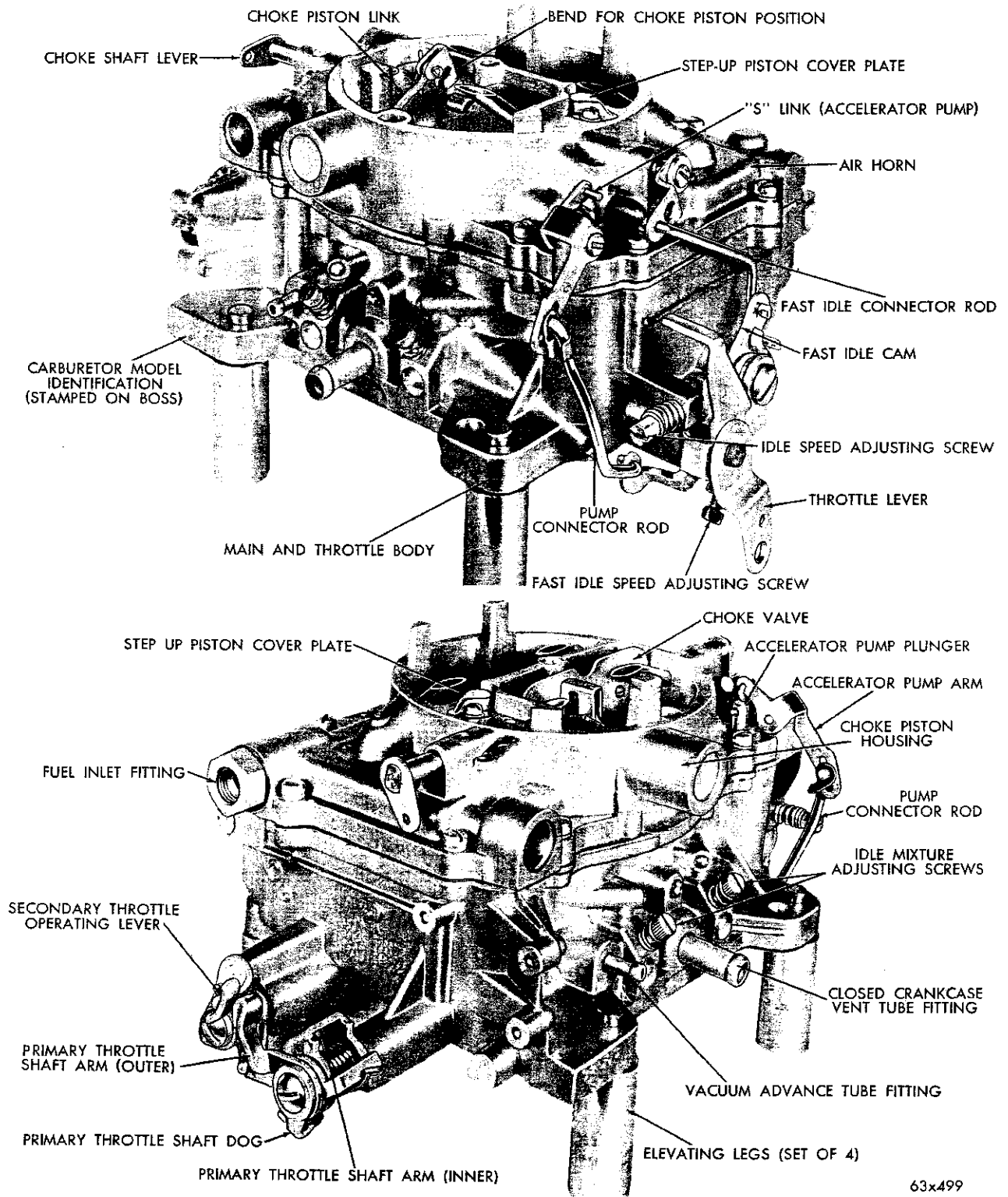
Fig. 37—Carburetor Assembly (AFB Series 32565 and 34785)
