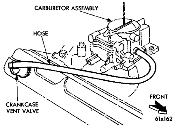
Fig. 56—Closed Crankcase Vent System
