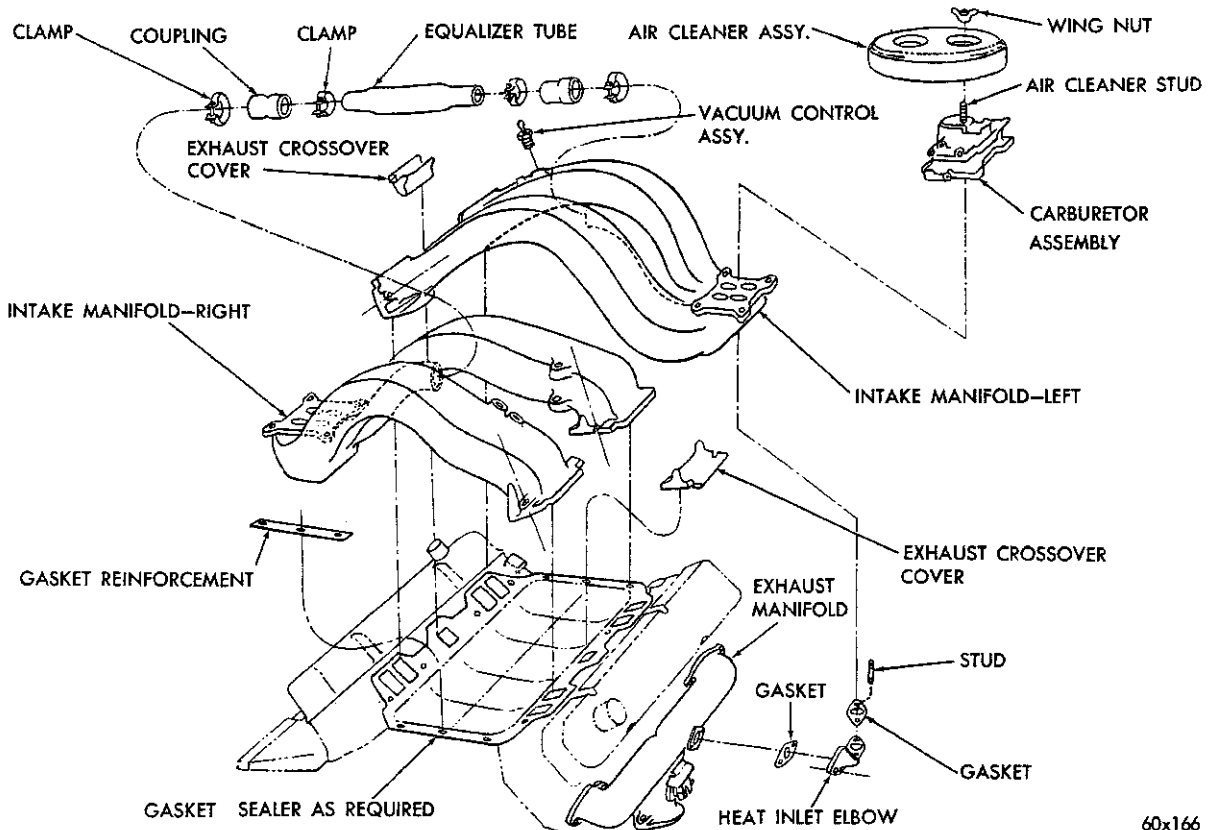
Fig. 59—C-300J Manifold (Disassembled)
