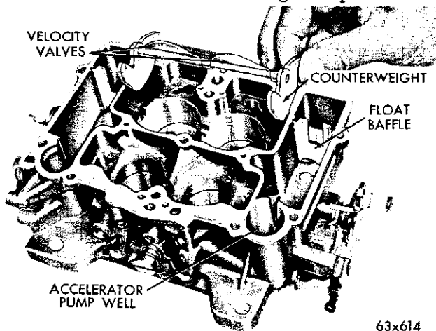
Fig. 67—Removing or Installing the Velocity Valves
