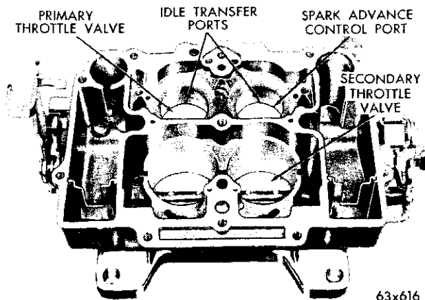
Fig. 69—Ports in Relation to Throttle Valves
