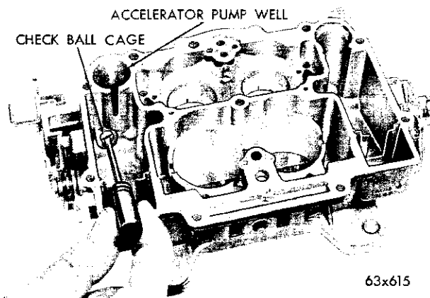
Fig. 68—Removing or Installing the Pump Inlet Check Ball Cage
