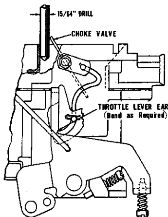
Fig. 19—Unloader Adjustment (Wide Open Kick)
