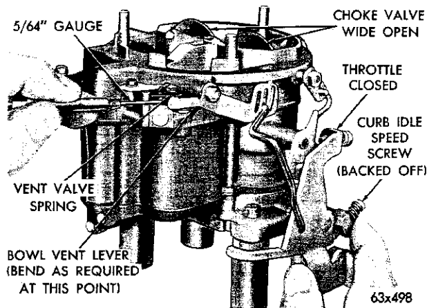
Fig. 21—Bowl Vent Valve Setting
