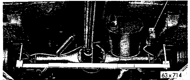
Fig. 14—Rear Alignment Gauge Installed
