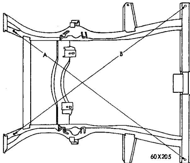
Fig. 4—Frame Diagonal Measurements
