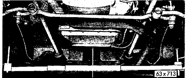
Fig. 13—Center Alignment Gauge Installed
