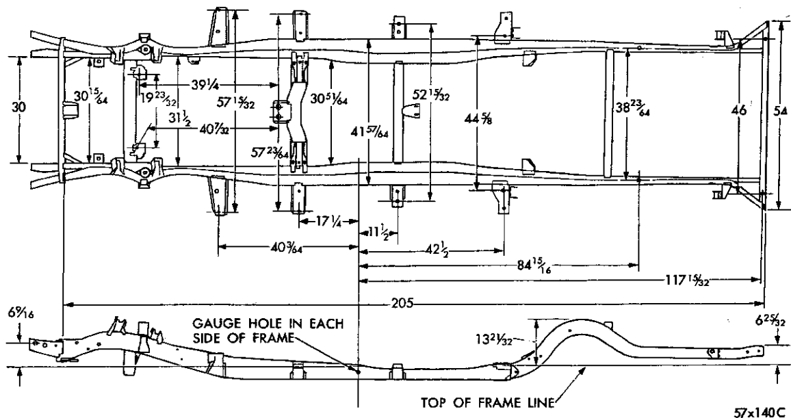
Fig. 1—Frame Dimensions (Imperial)
