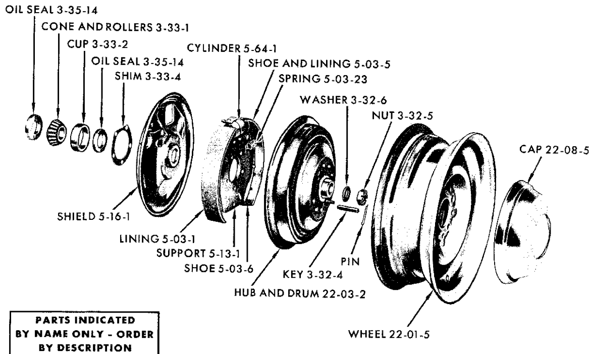
FRONT WHEEL - CHRYSLER SC1-2-3
