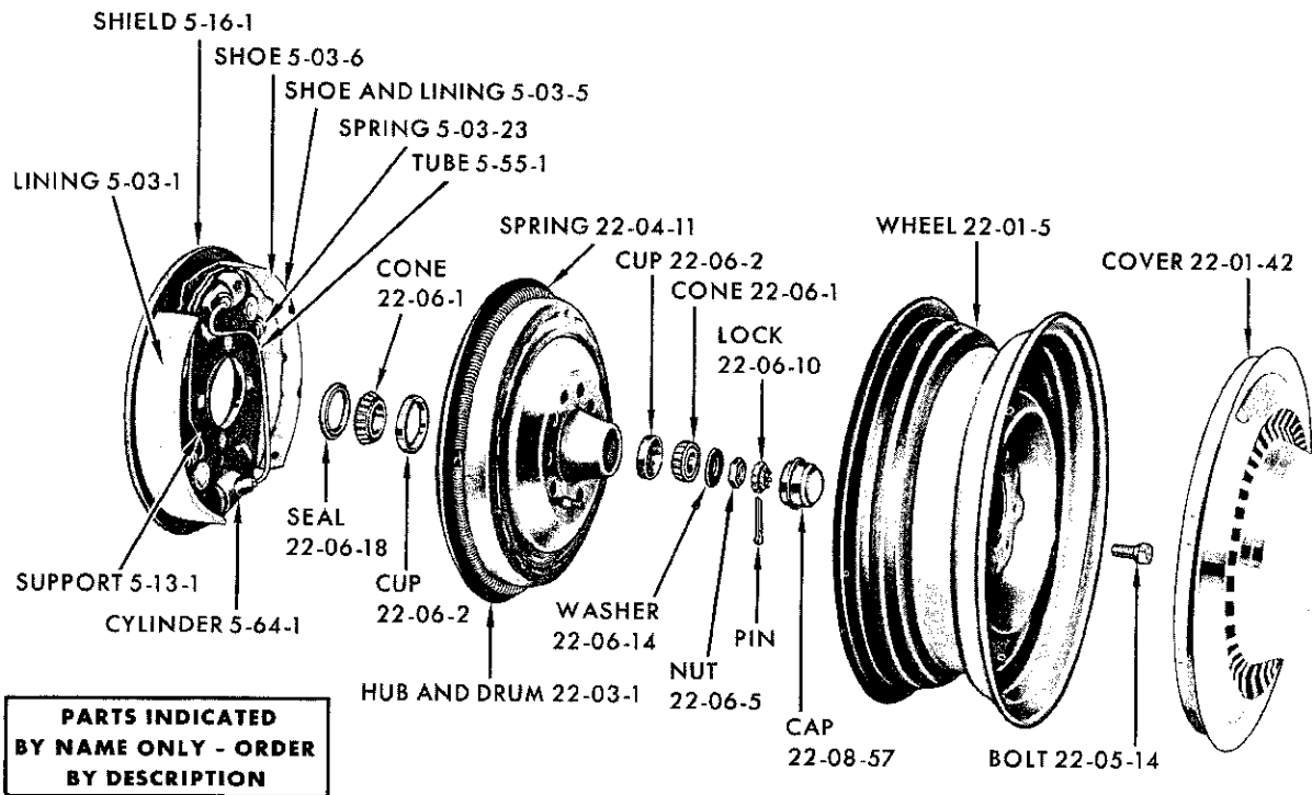
FRONT WHEEL - CHRYSLER SC1-2-3
