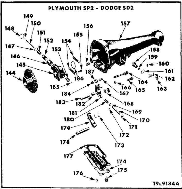
AUTOMATIC 3-SPEED TRANSMISSION - V8 CYLINDER
