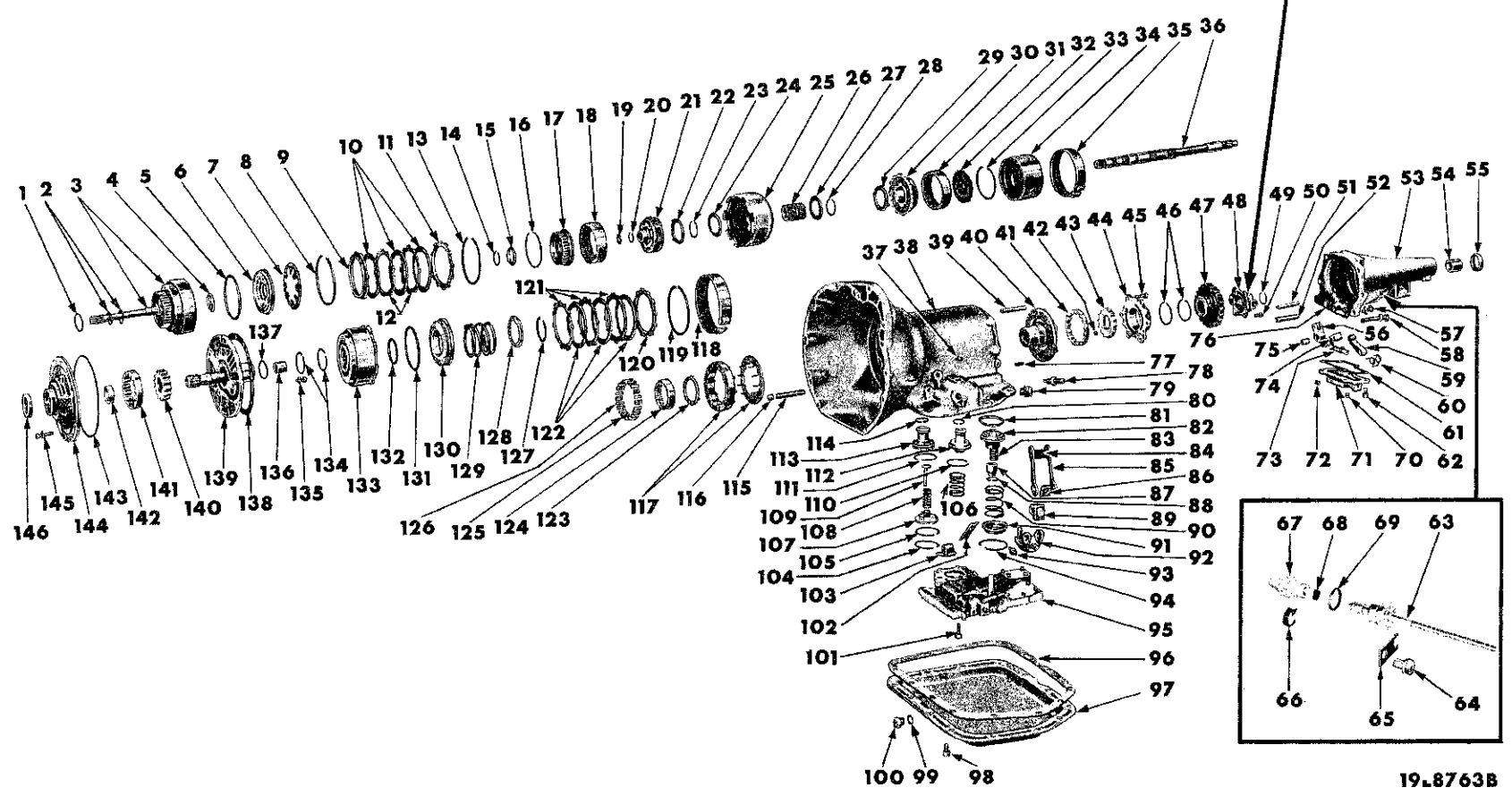
AUTOMATIC 3-SPEED TRANSMISSION - 6 CYLINDER
