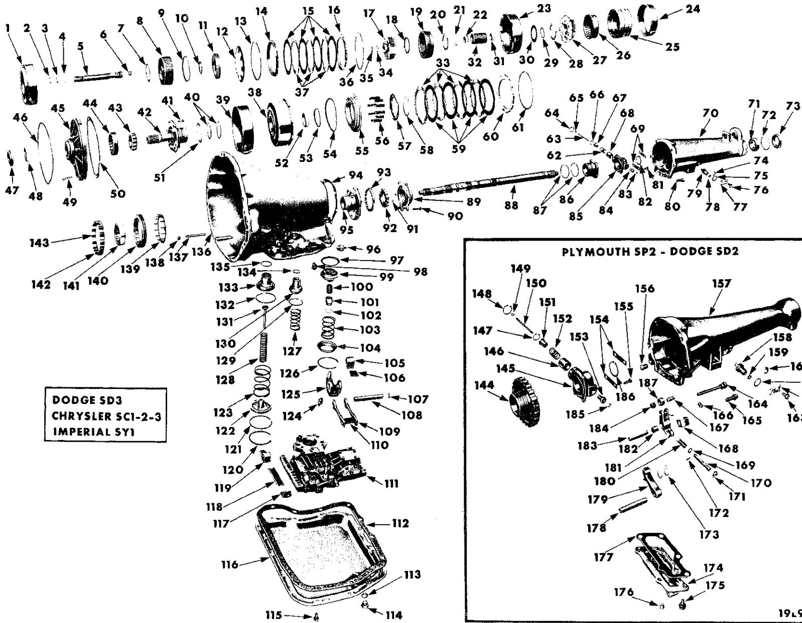
AUTOMATIC 3-SPEED TRANSMISSION - V8 CYLINDER
