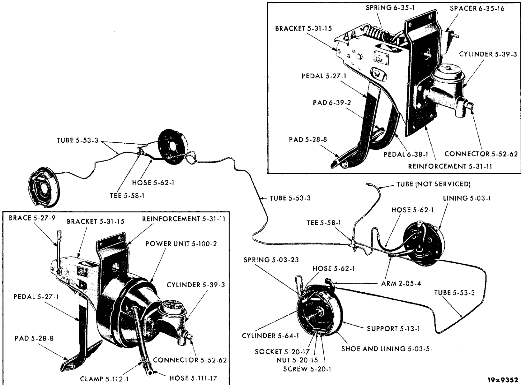
HYDRAULIC BRAKE SYSTEM - PLYMOUTH SP1-2 AND DART SD1-2
