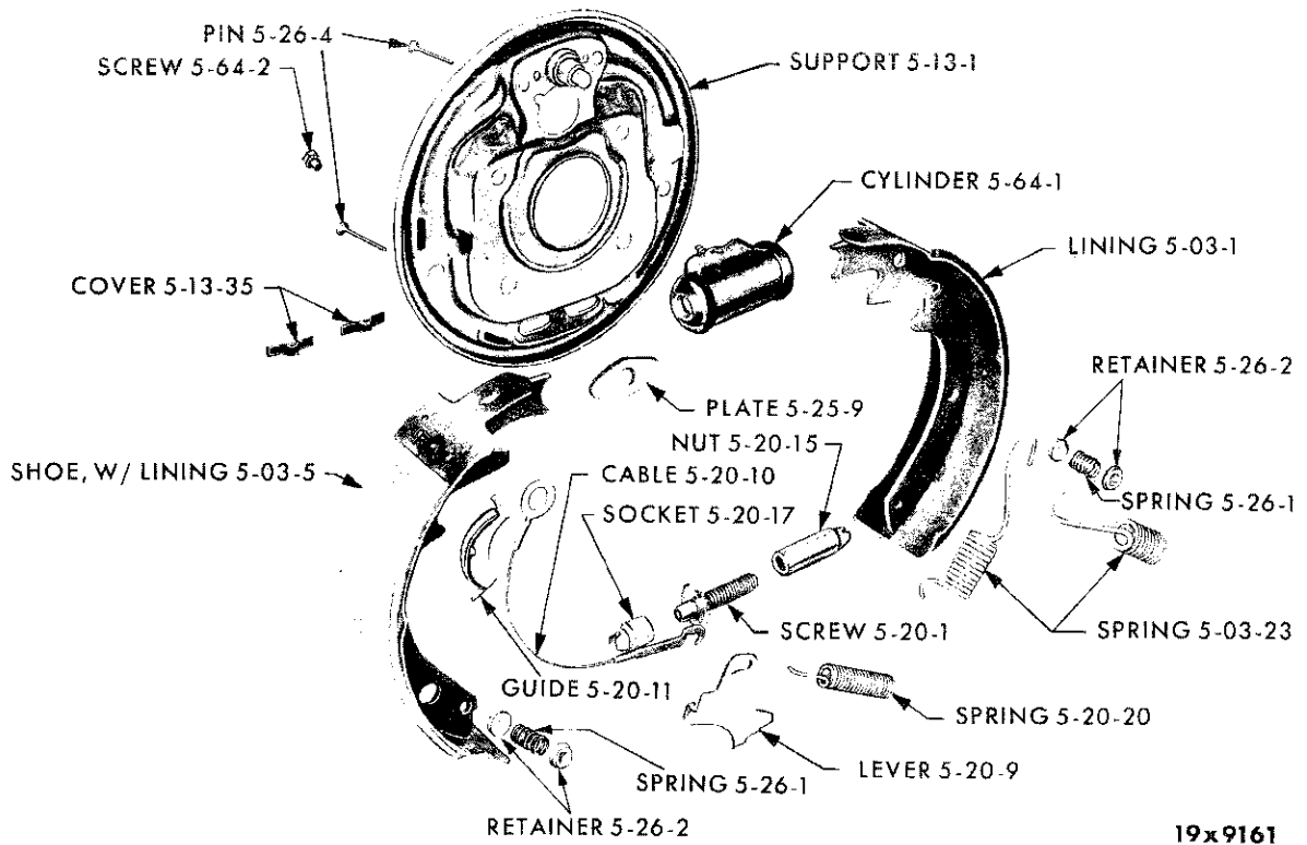
FRONT WHEEL BRAKE - PLYMOUTH SP1-2 AND DODGE SD1-2
