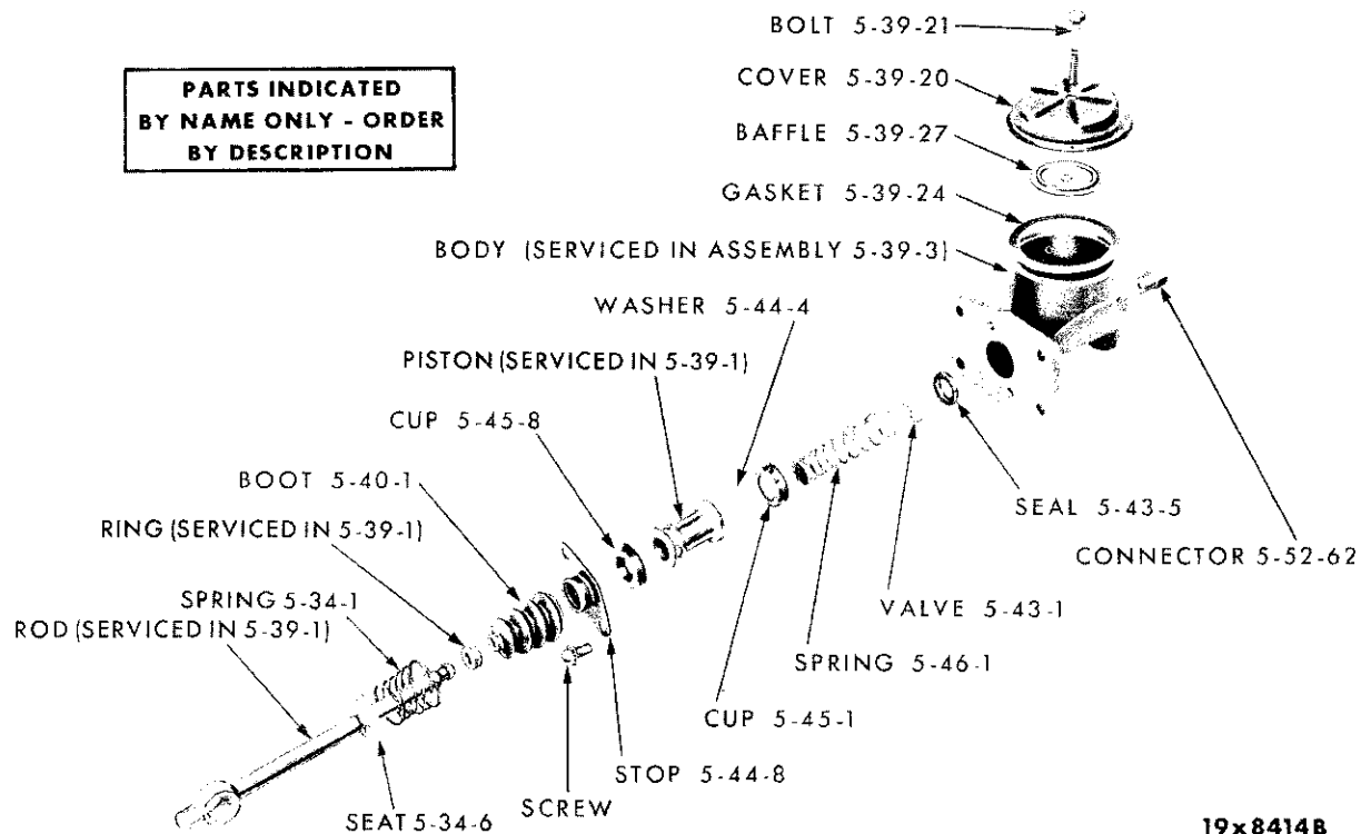
MASTER CYLINDER (WITHOUT POWER BRAKES) - EXCEPT IMPERIAL SY1
