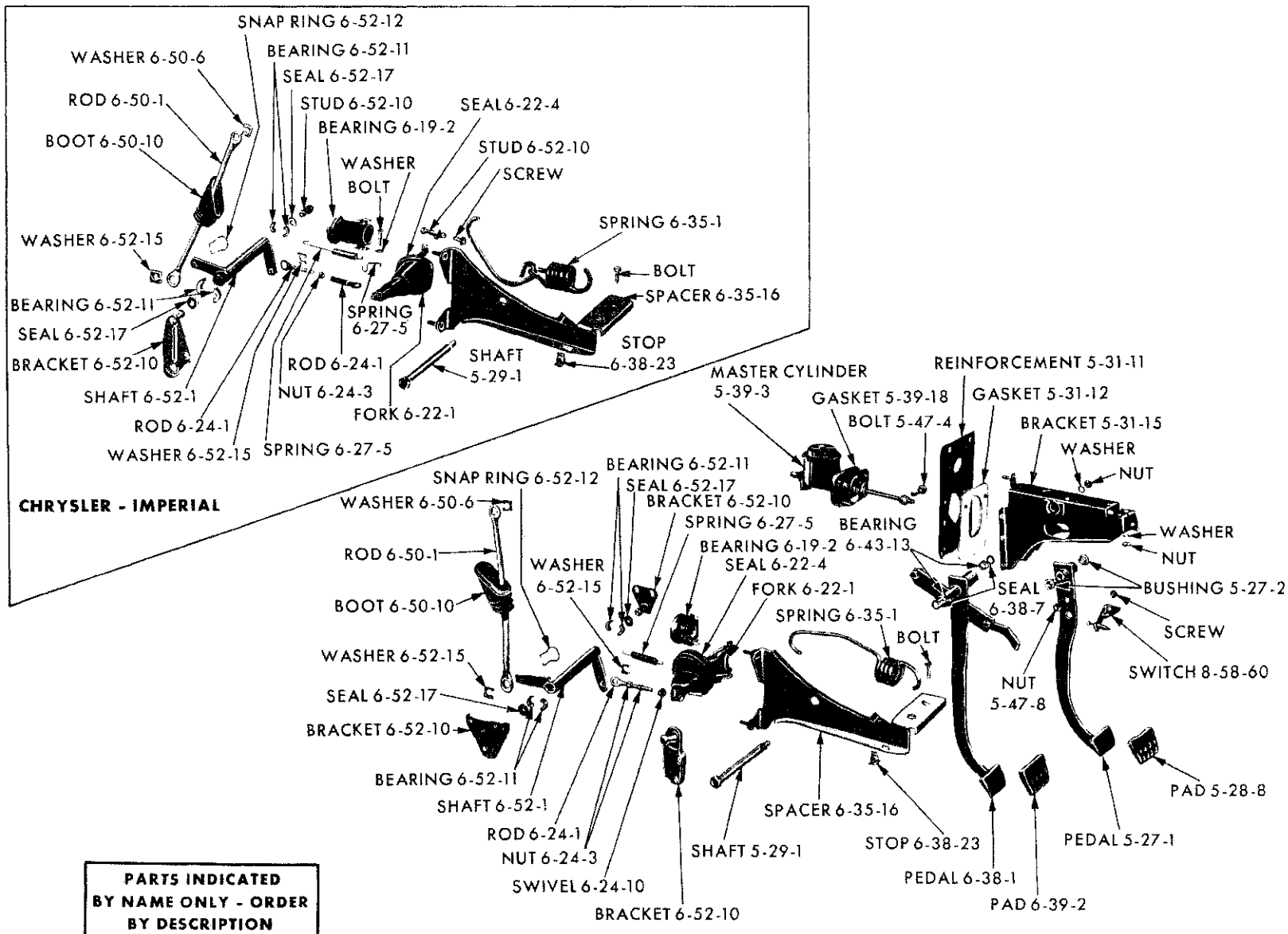
BRAKE AND CLUTCH PEDAL LINKAGE - PLYMOUTH SP1-2, DODGE SD1-2-3, CHRYSLER SC1-2-3 AND IMPERIAL SY1
