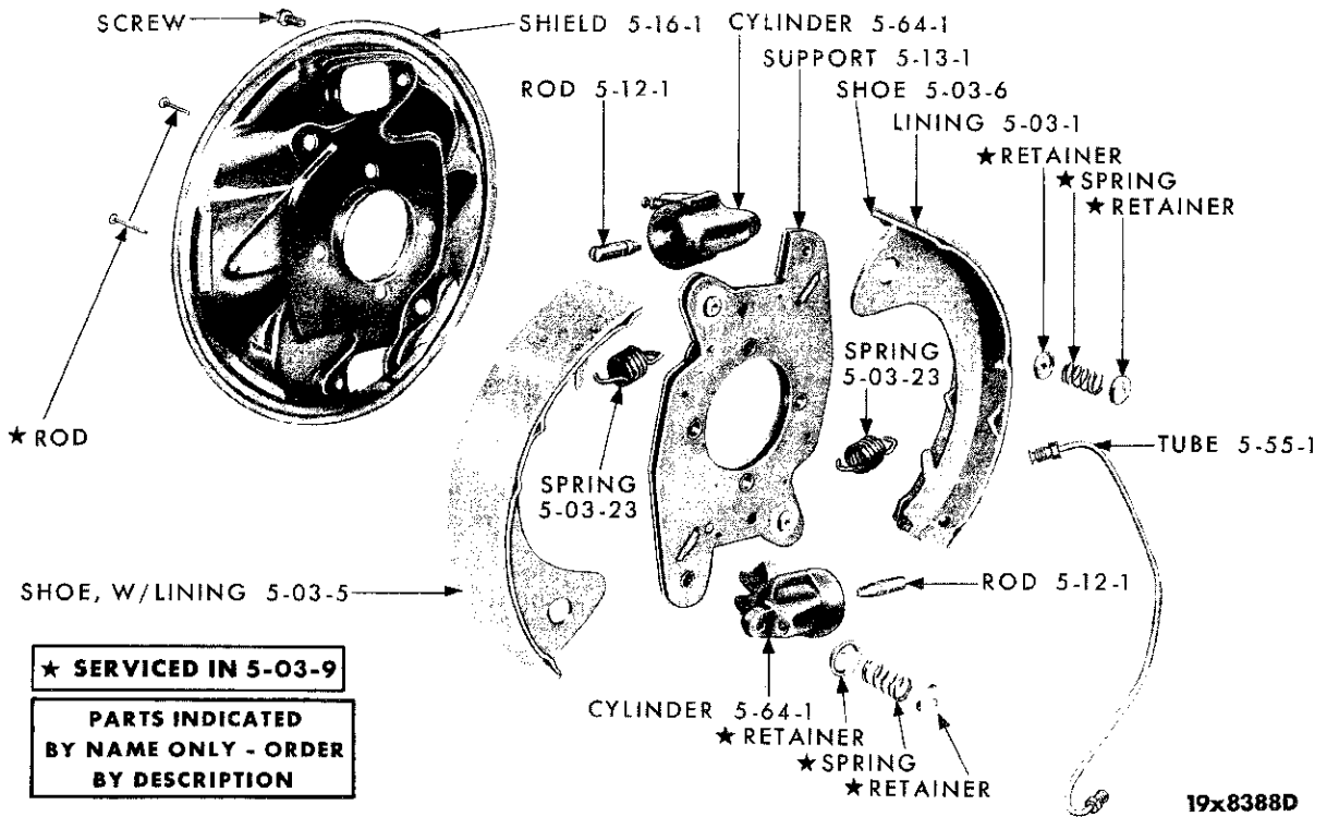
FRONT WHEEL BRAKE - DODGE SD3, CHRYSLER SC1-2-3 AND IMPERIAL SY1
