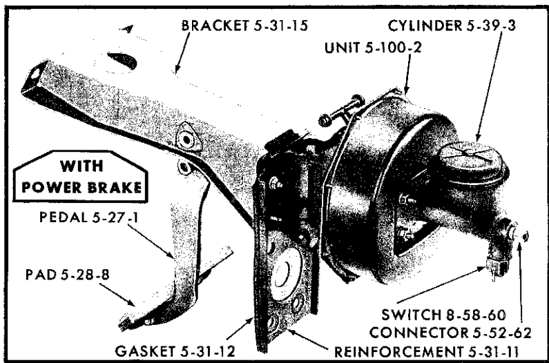
HYDRAULIC BRAKE SYSTEM - VALIANT SV1 AND LANCER SL1
