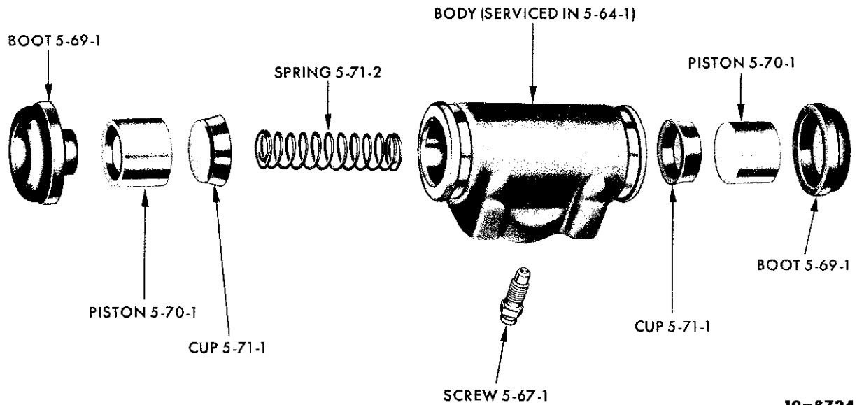
FRONT AND REAR WHEEL CYLINDER - EXCEPT CHRYSLER SC1-2-3 AND IMPERIAL SY1
