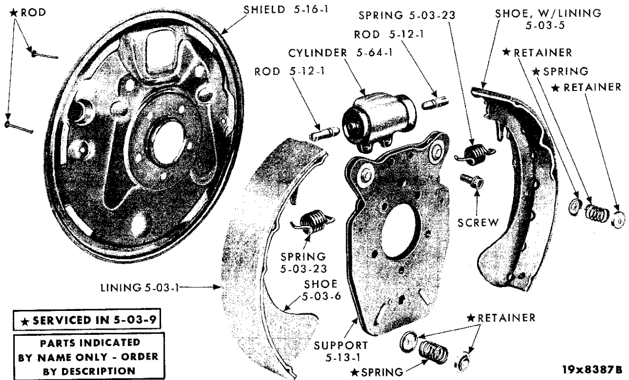
REAR WHEEL BRAKE - DODGE SD3, CHRYSLER SC1-2-3 AND IMPERIAL SY1
