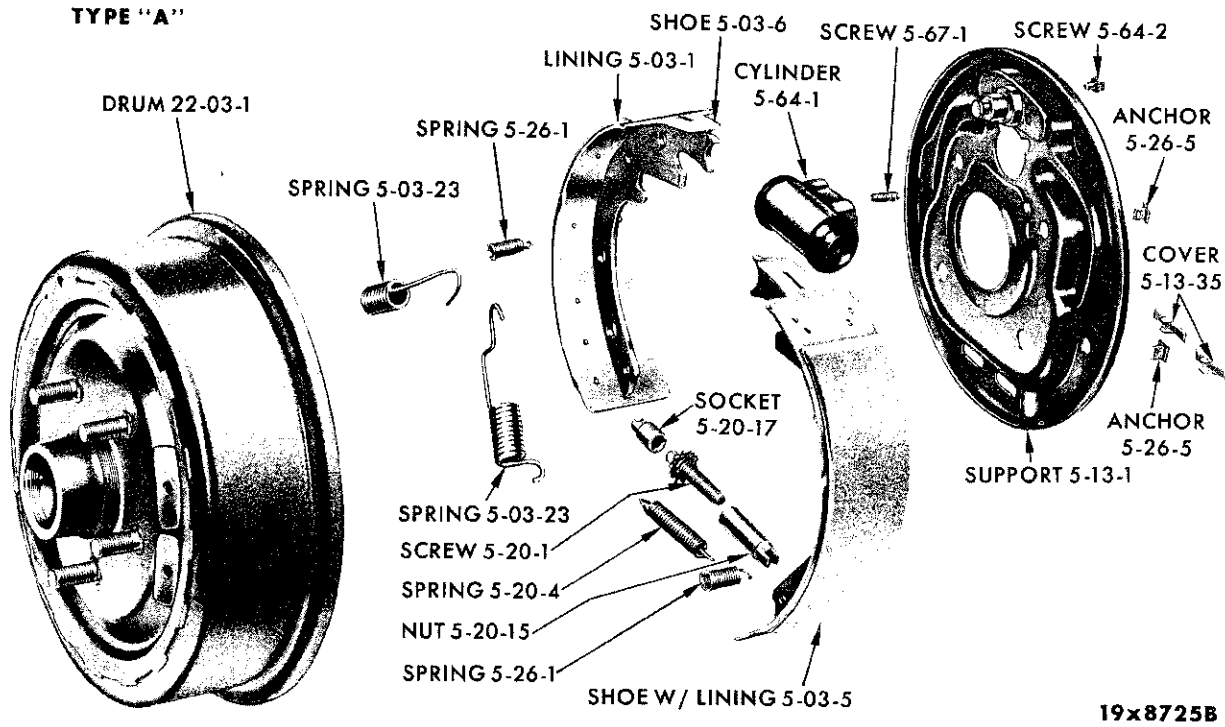
FRONT WHEEL BRAKE - VALIANT SV1 AND LANCER SL1
