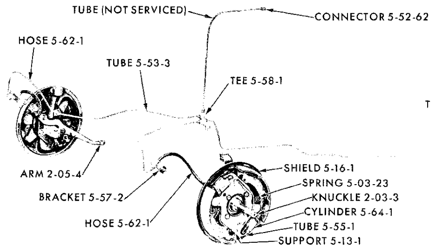
HYDRAULIC BRAKE SYSTEM - DODGE SD3, CHRYSLER SC1-2-3 AND IMPERIAL SY1
