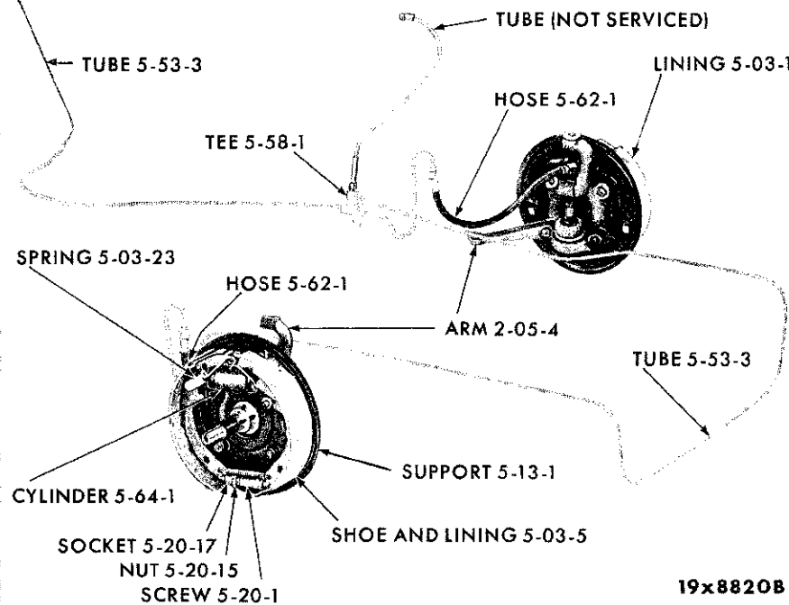
HYDRAULIC BRAKE SYSTEM - VALIANT SV1 AND LANCER SL1
