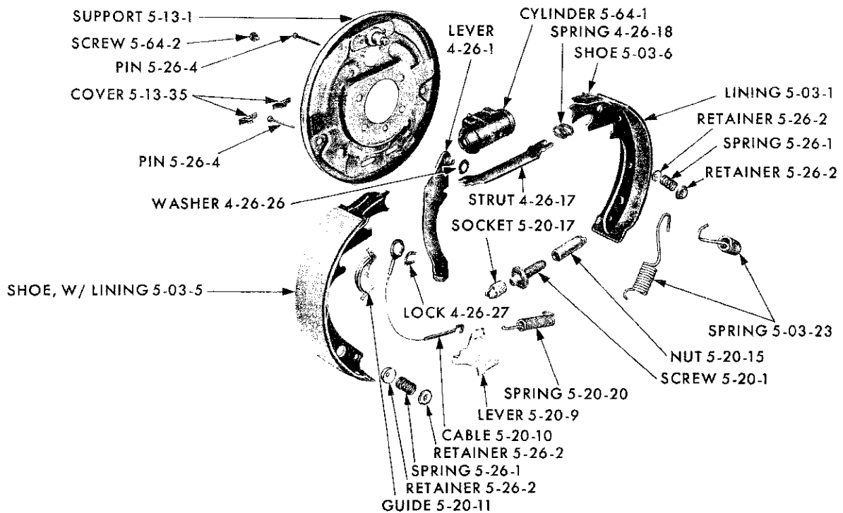
REAR WHEEL BRAKE - PLYMOUTH SP1-2 AND DODGE SD1-2
