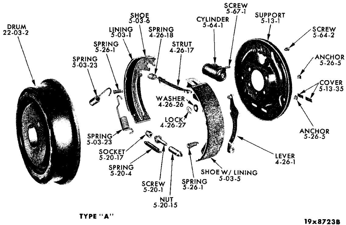
REAR WHEEL BRAKE - VALIANT SV1 AND LANCER SL1
