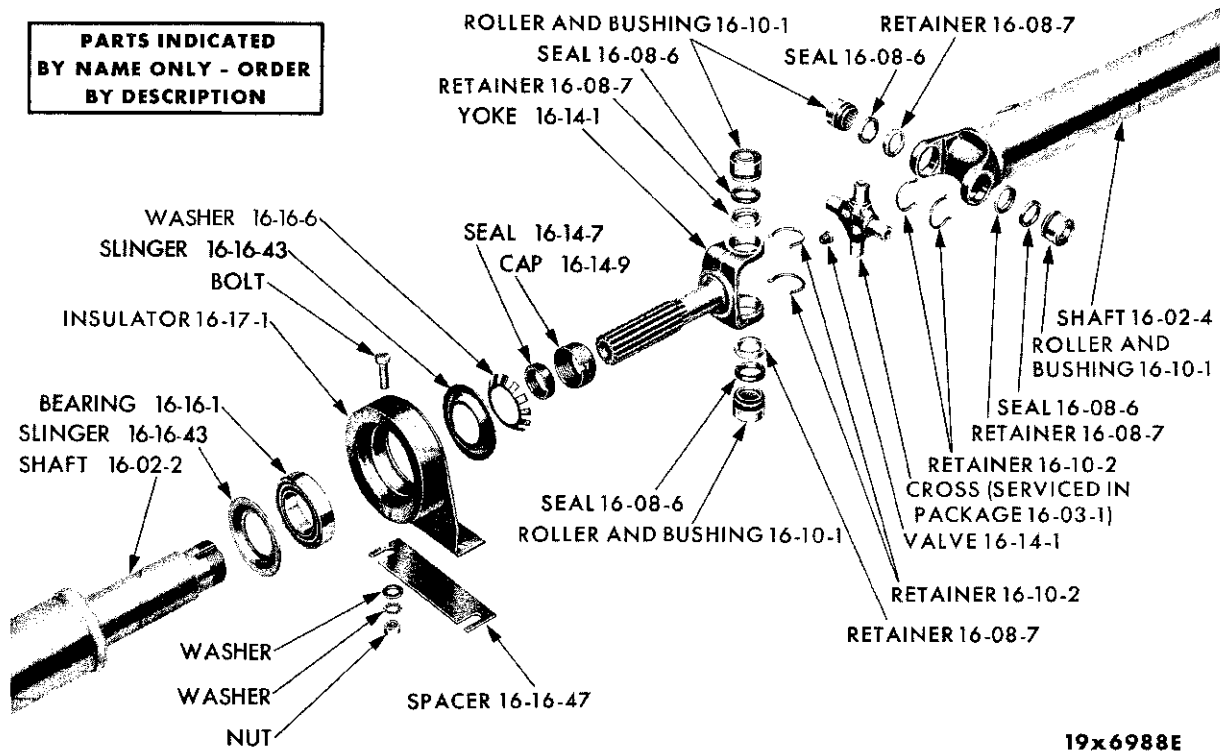
PROPELLER SHAFT CENTER BEARING - IMPERIAL SY1
