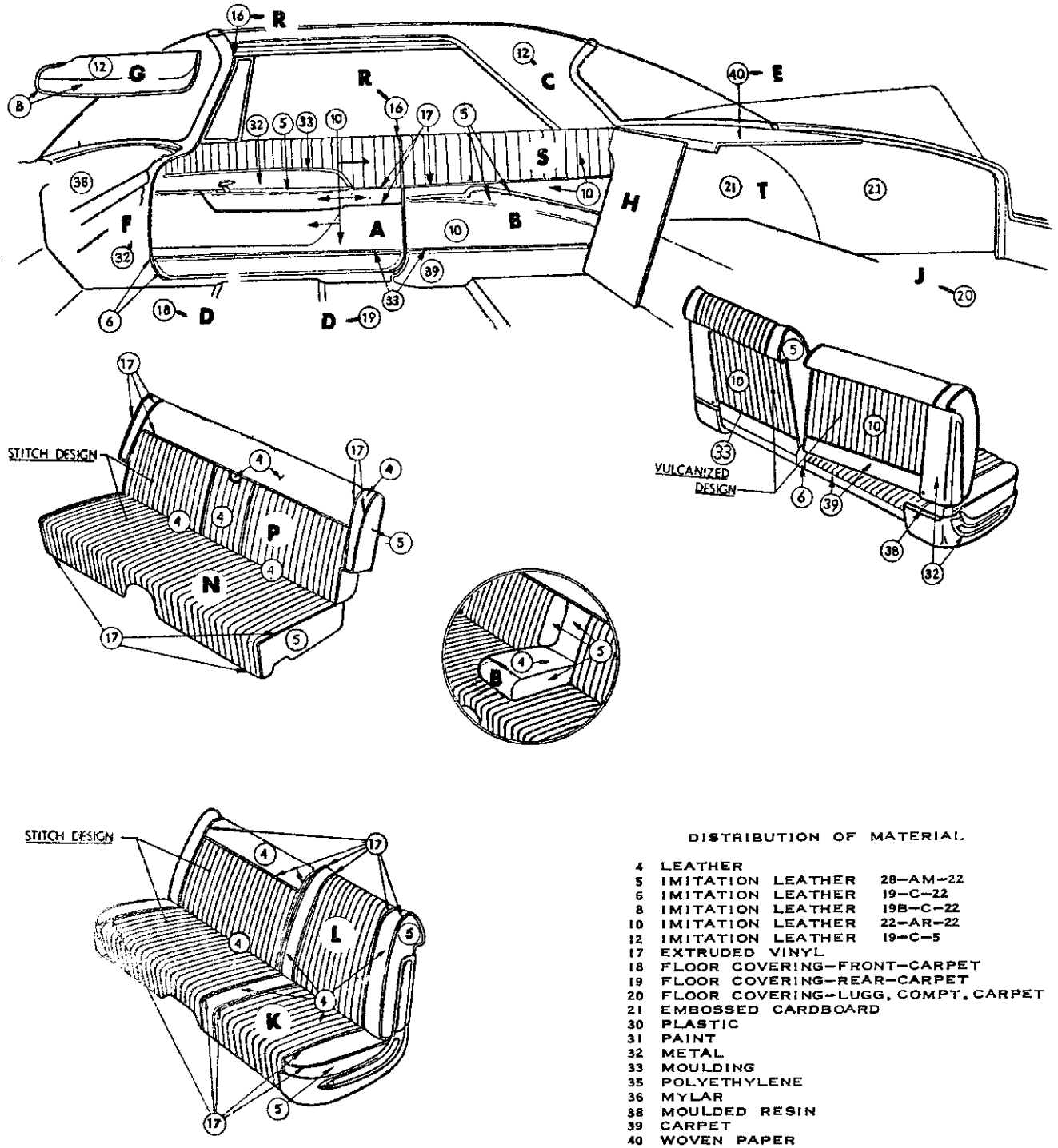
Distribution Drawing Legend Page Appears Following Illustration Section
