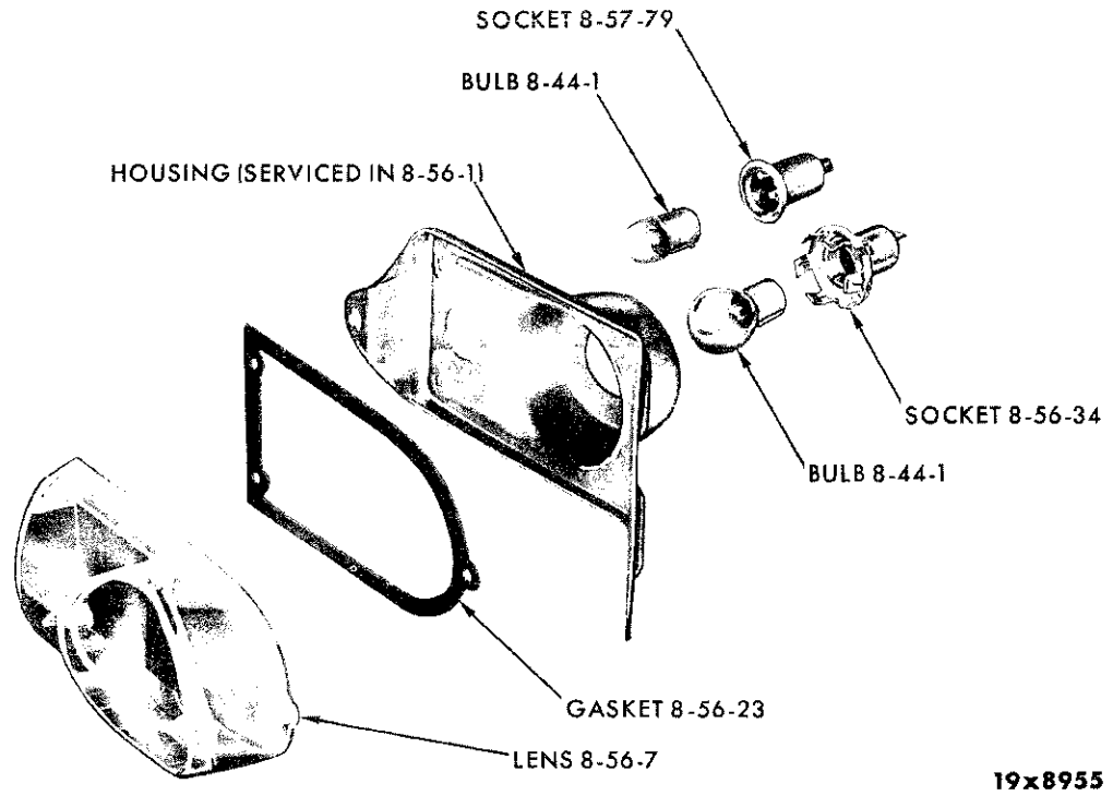
BACK-UP AND LICENSE LAMP - CHRYSLER SC1-2-3 (SUBURBAN)
