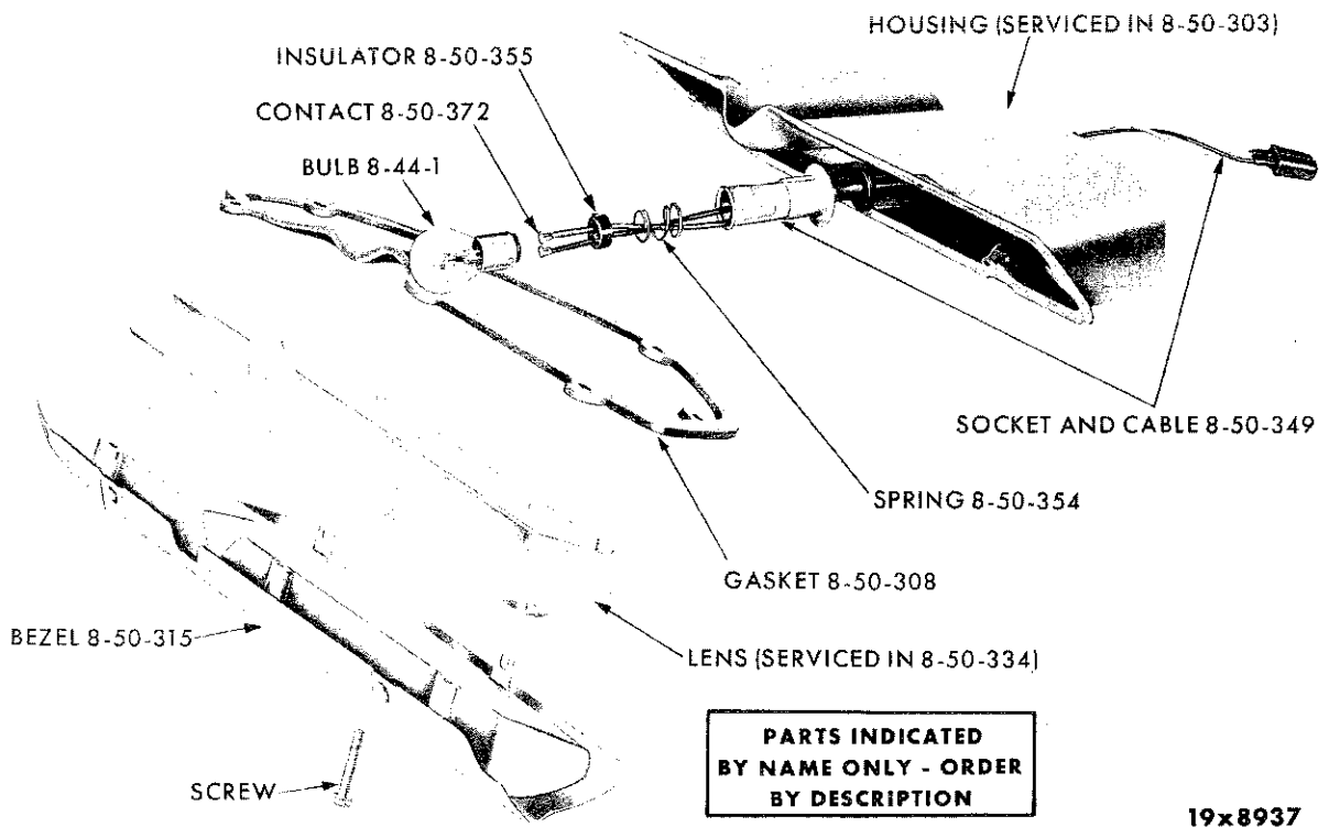
PARKING LAMP - IMPERIAL SY1
