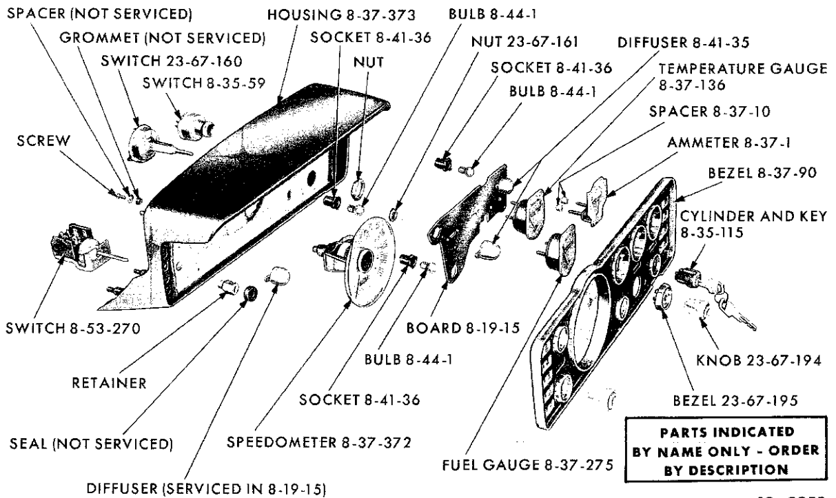
INSTRUMENT CLUSTER - VALIANT SV1
