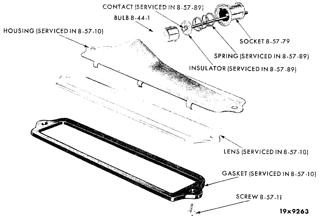
LICENSE LAMP - DODGE SD1-2 (EXCEPT SUBURBAN)
