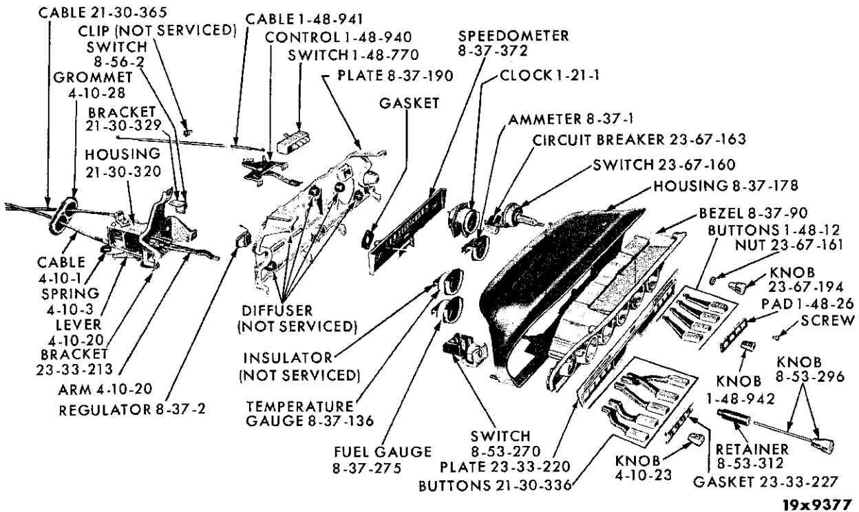
INSTRUMENT CLUSTER - DART SD1-2
