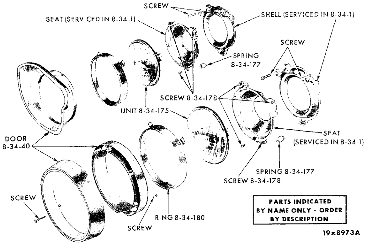
HEADLAMP - DODGE SD1-2
