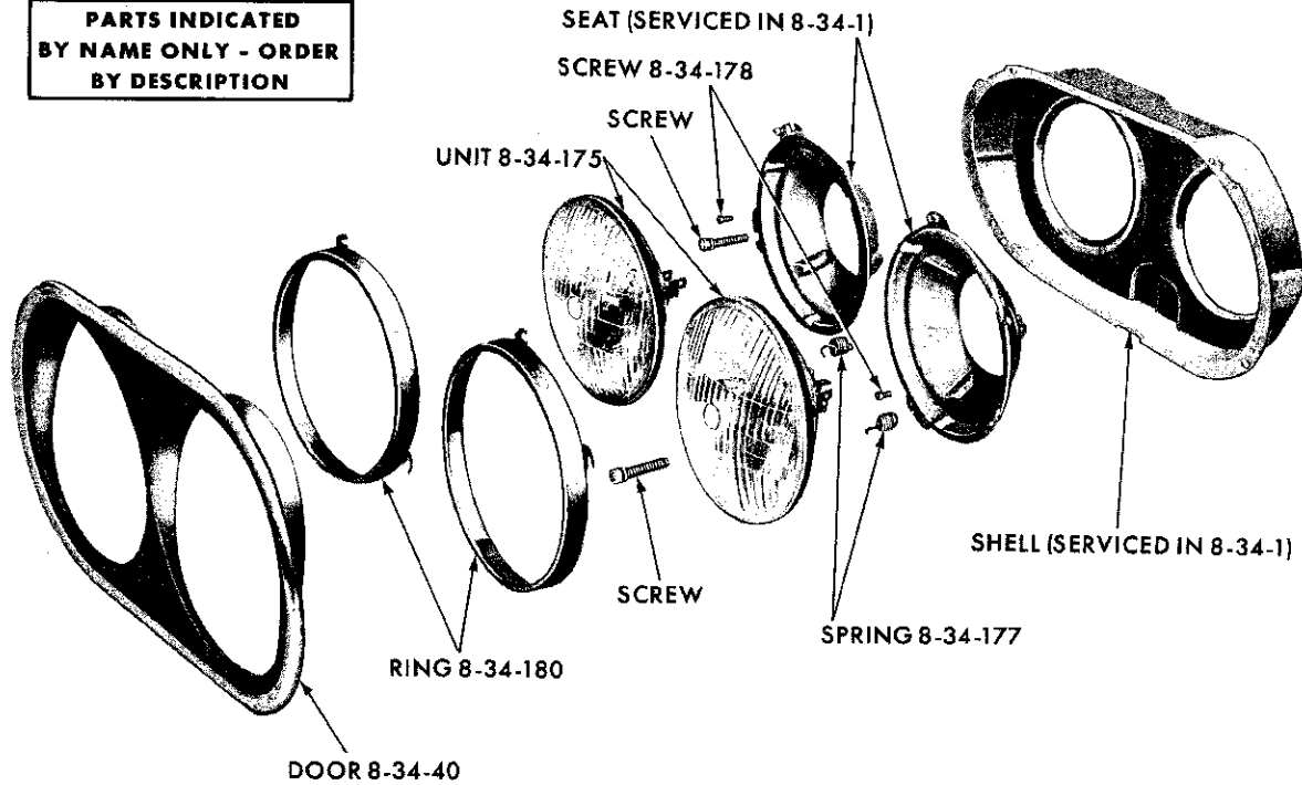
HEADLAMP - VALIANT SV1
