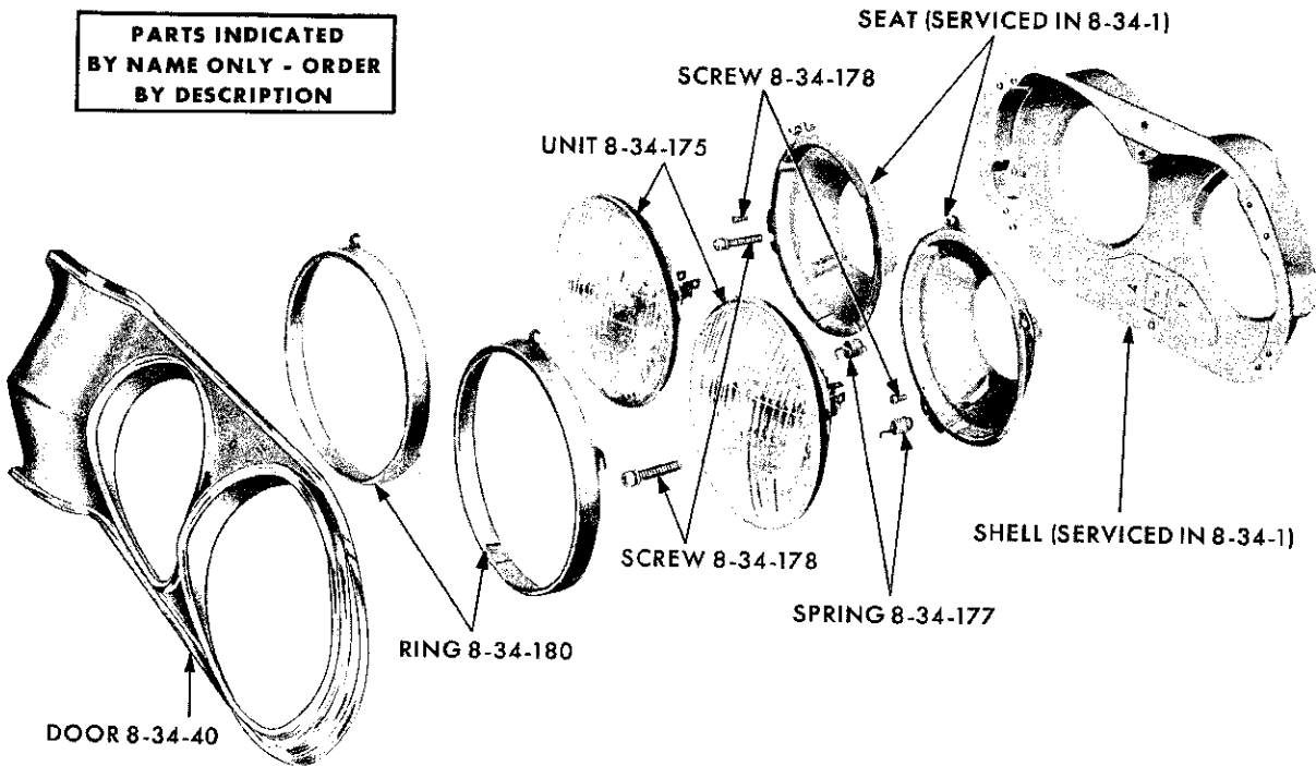
HEADLAMP - LANCER SL1
