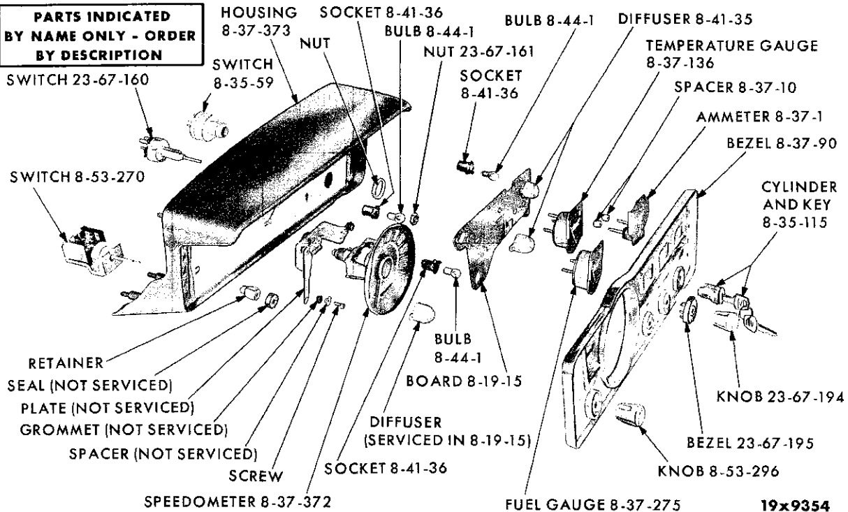
INSTRUMENT CLUSTER - LANCER SL1
