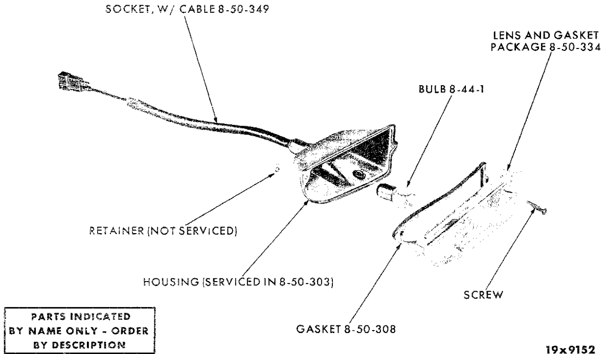
PARKING LAMP - PLYMOUTH SP1-2
