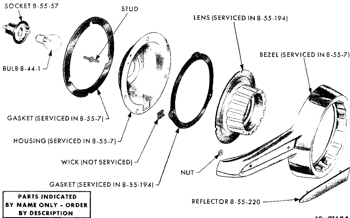
TAIL AND STOP LAMP - LANCER SL1
