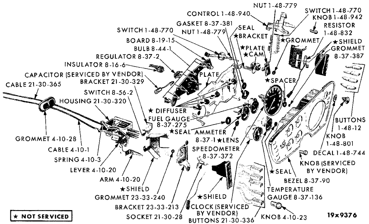
INSTRUMENT CLUSTER - PLYMOUTH SP1-2
