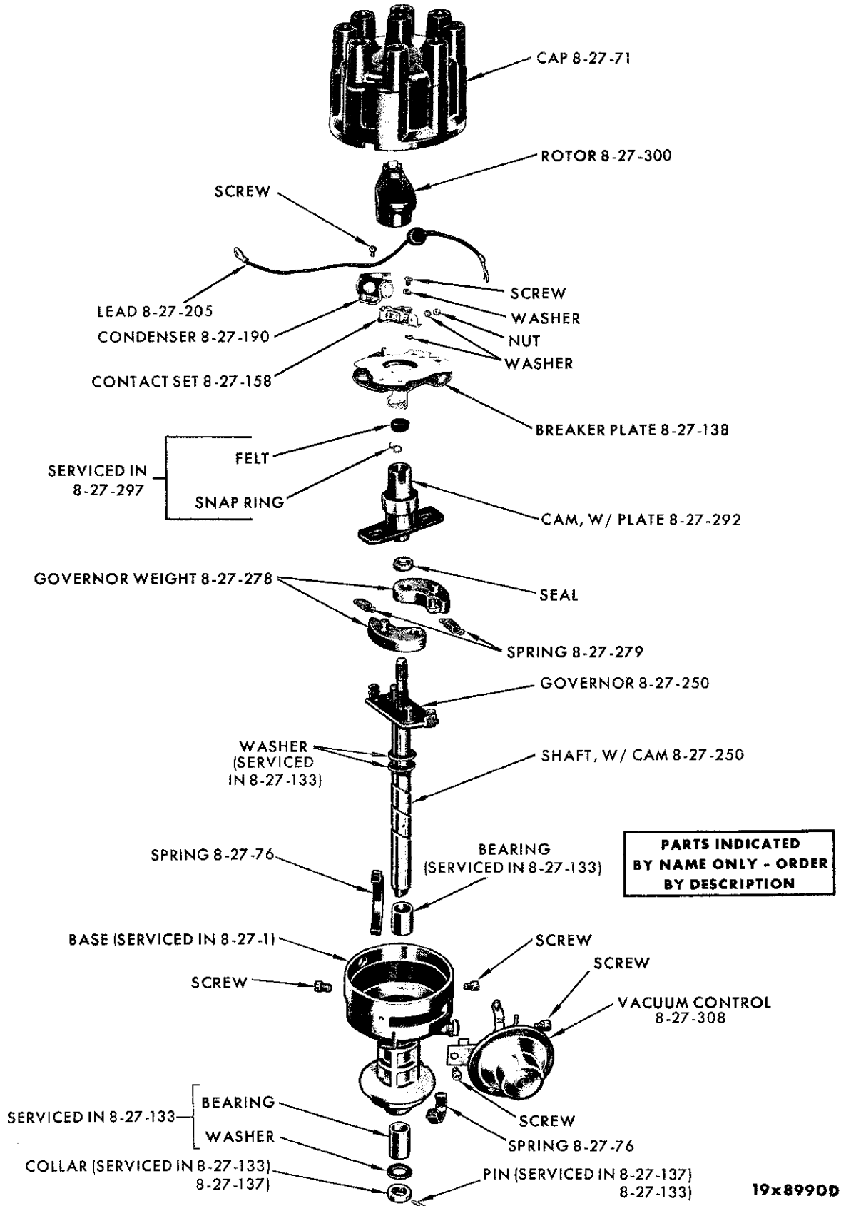
DISTRIBUTOR - V8 CYLINDER
