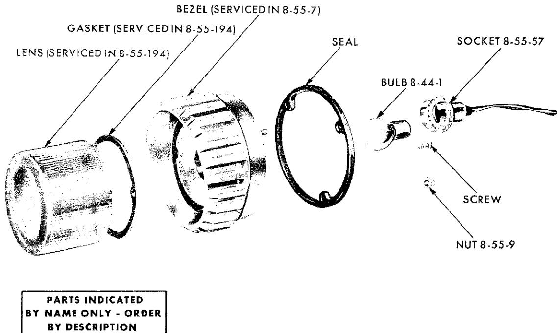
TAIL AND STOP LAMP - PLYMOUTH SP1-2
