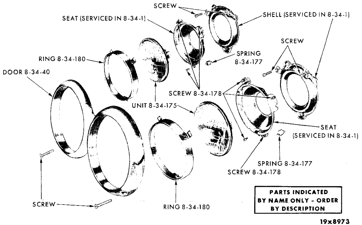
HEADLAMP - DODGE SD3
