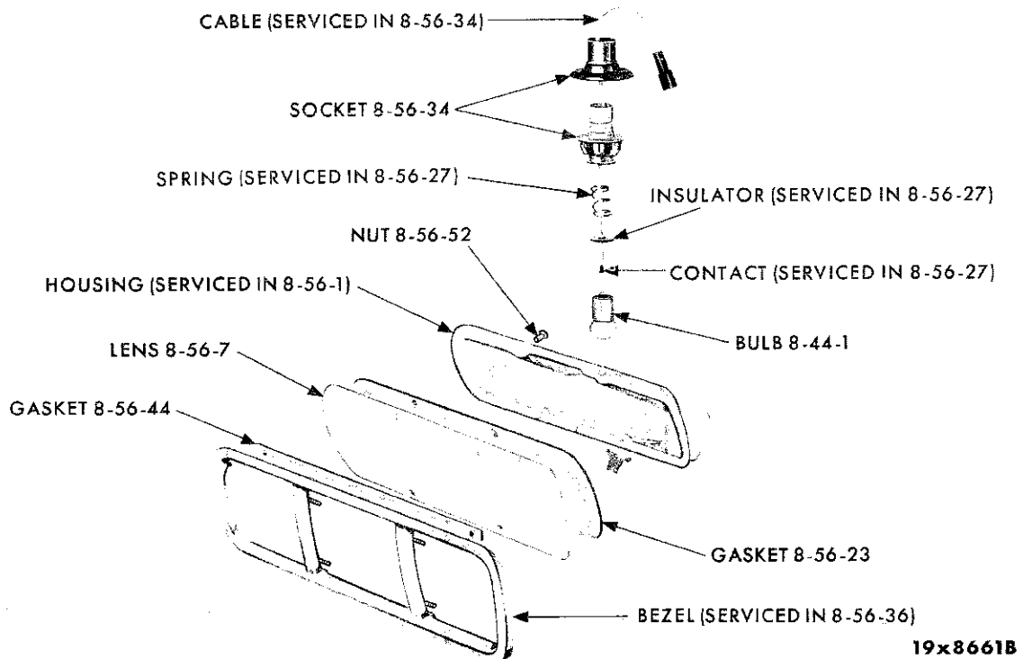
BACK-UP LAMP - IMPERIAL SY1
