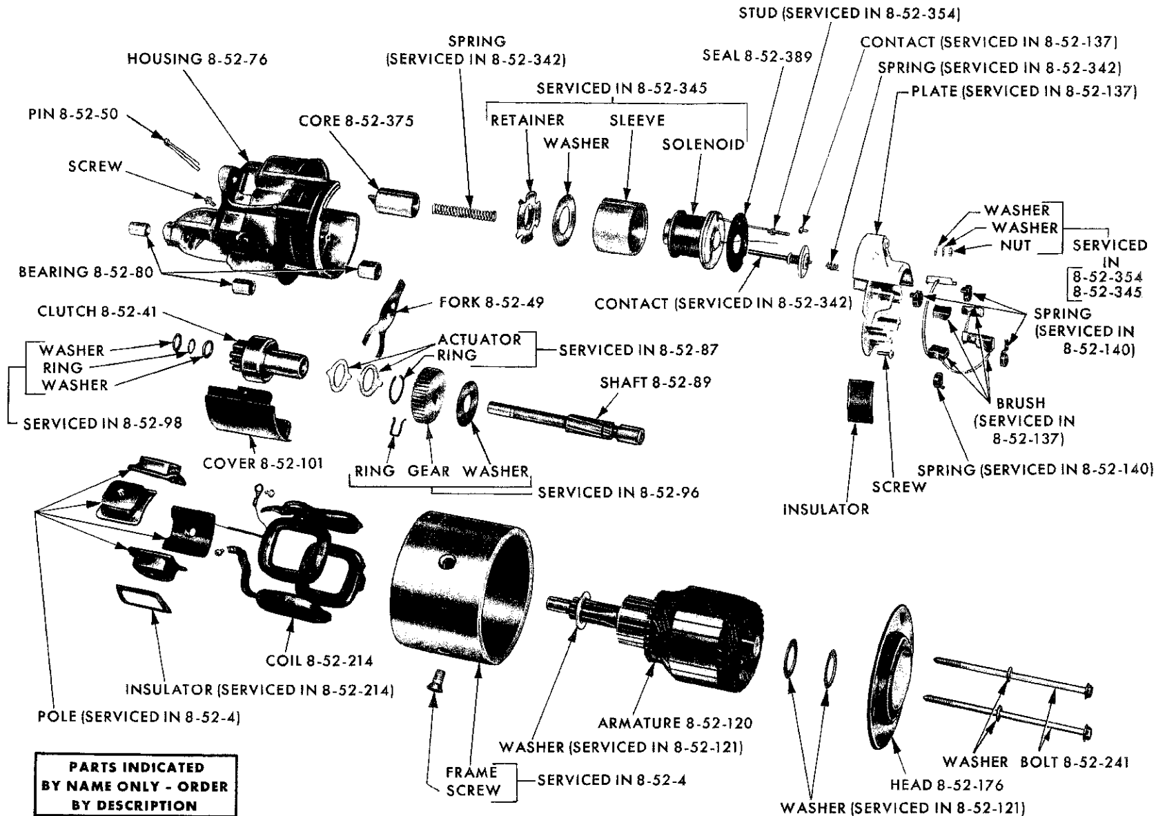
STARTER
