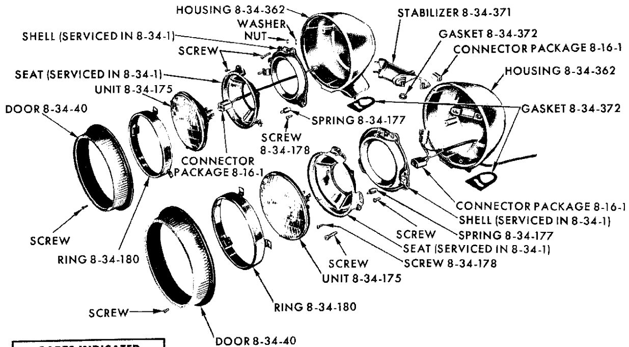
HEADLAMP - CHRYSLER SC1-2-3
