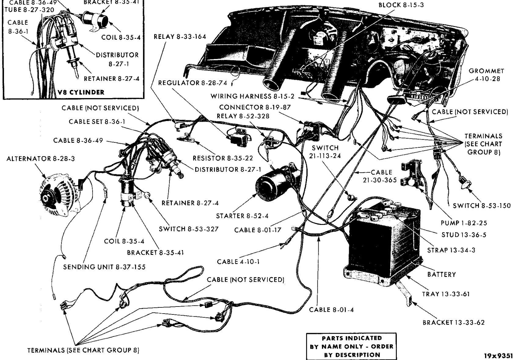
ELECTRICAL SYSTEM
