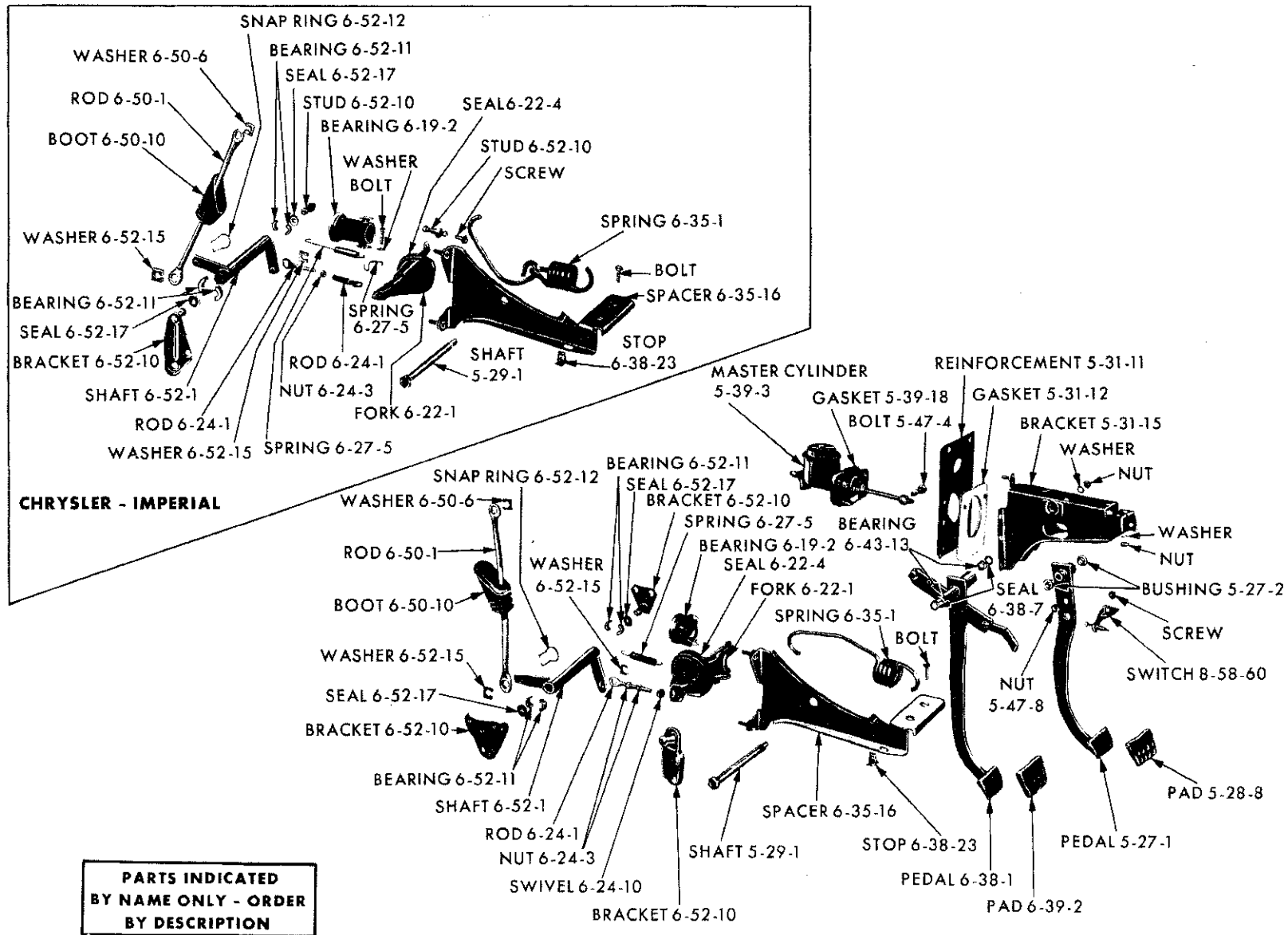
CLUTCH AND BRAKE PEDAL LINKAGE - PLYMOUTH SP1-2, DODGE SD1-2-3, CHRYSLER SC1-2-3 AND IMPERIAL SY1
