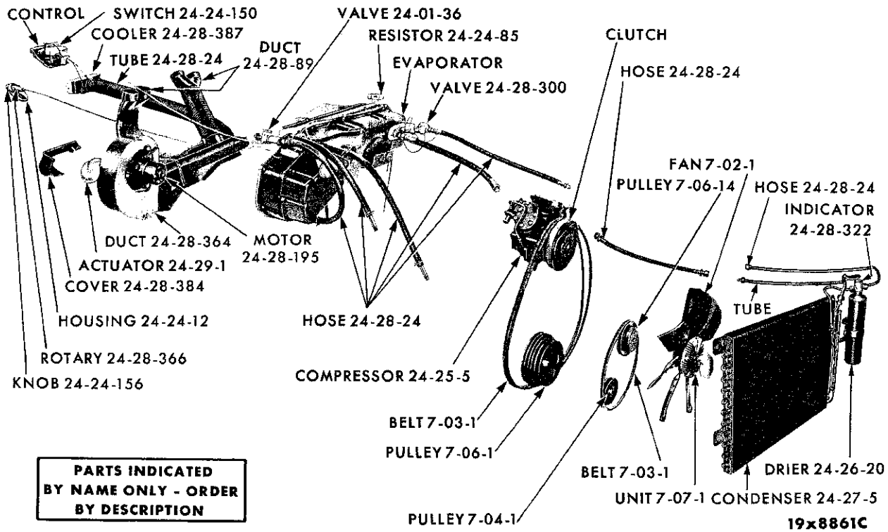
AIR CONDITIONING SYSTEM - CHRYSLER SC1-2-3 AND IMPERIAL SY1
