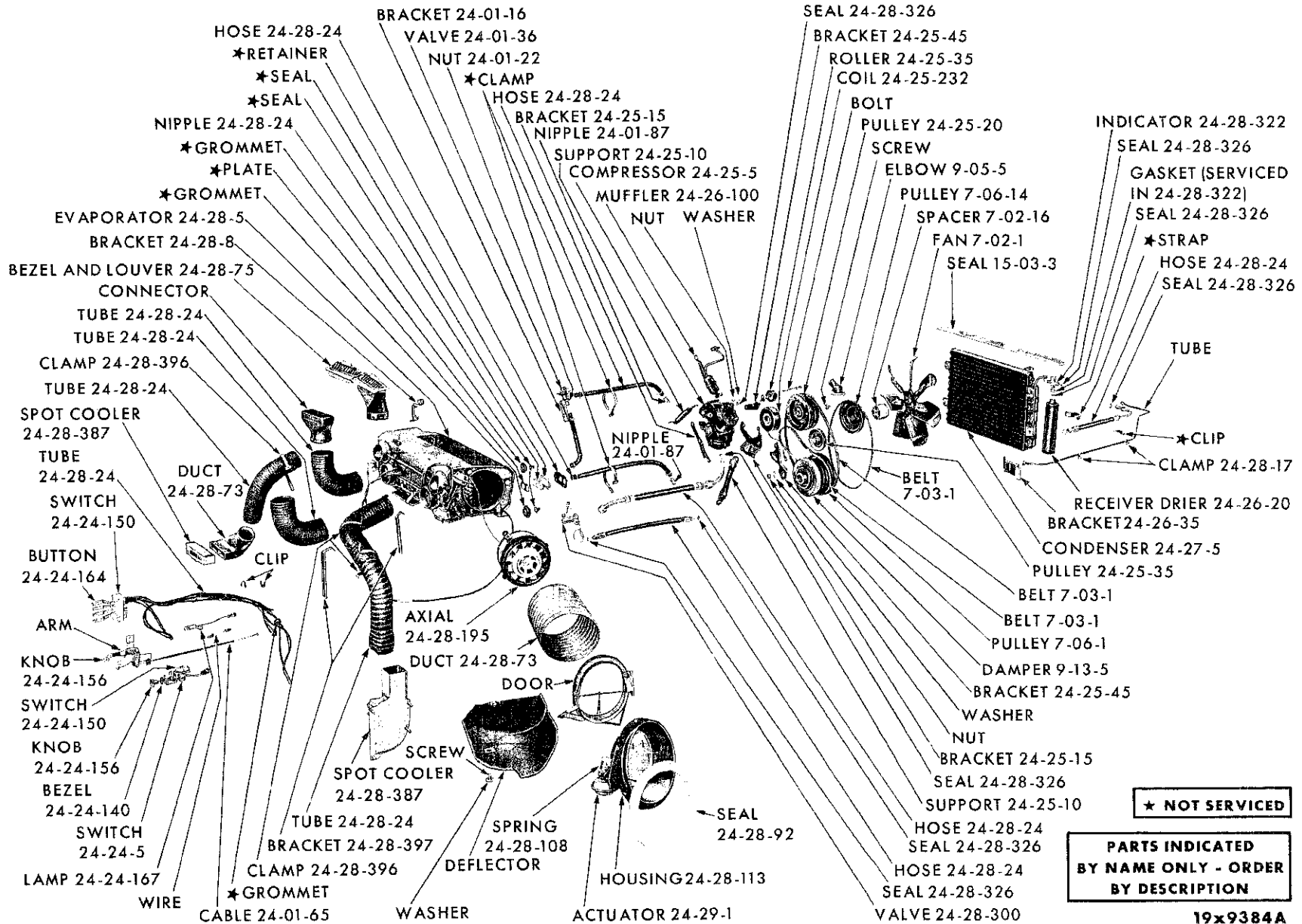
AIR CONDITIONING SYSTEM - PLYMOUTH SP1-2 AND DART SD1-2
