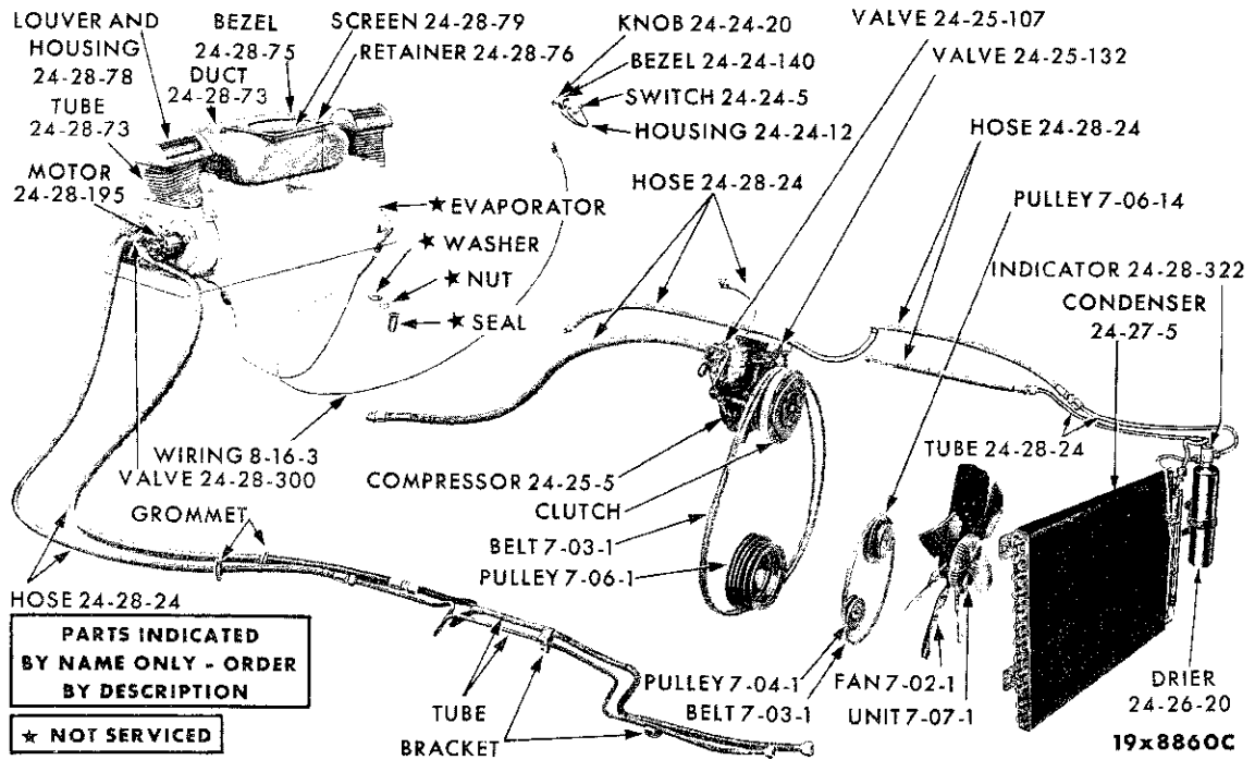
AIR CONDITIONING SYSTEM - TRUNK TYPE
