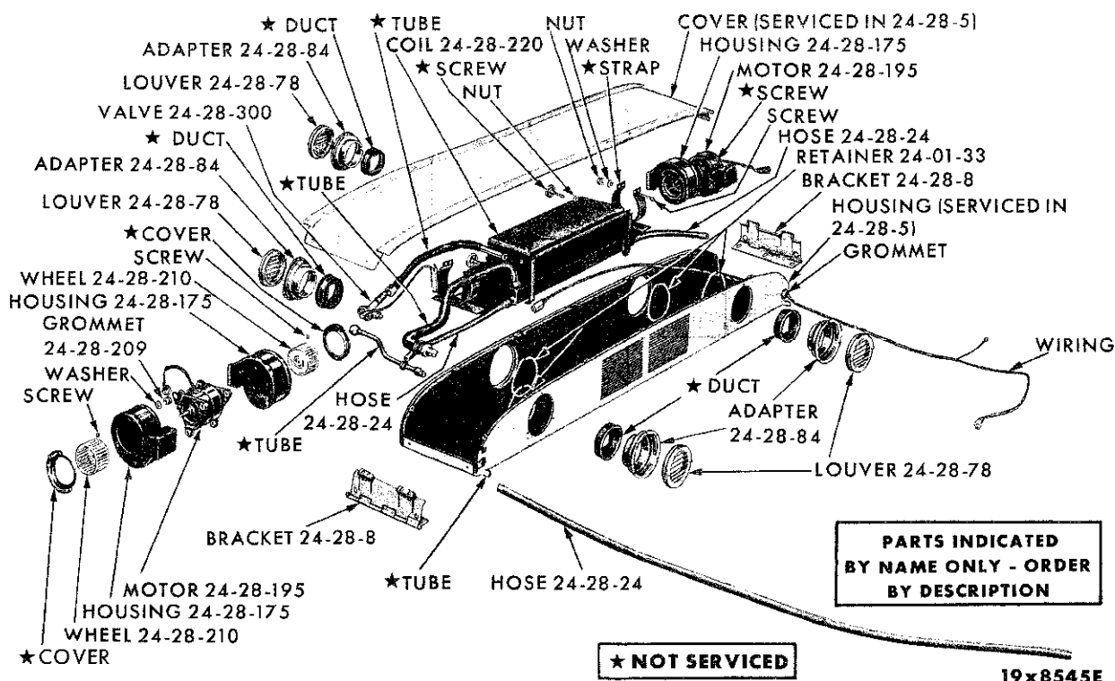
AIR CONDITIONING EVAPORATOR - SUBURBAN
