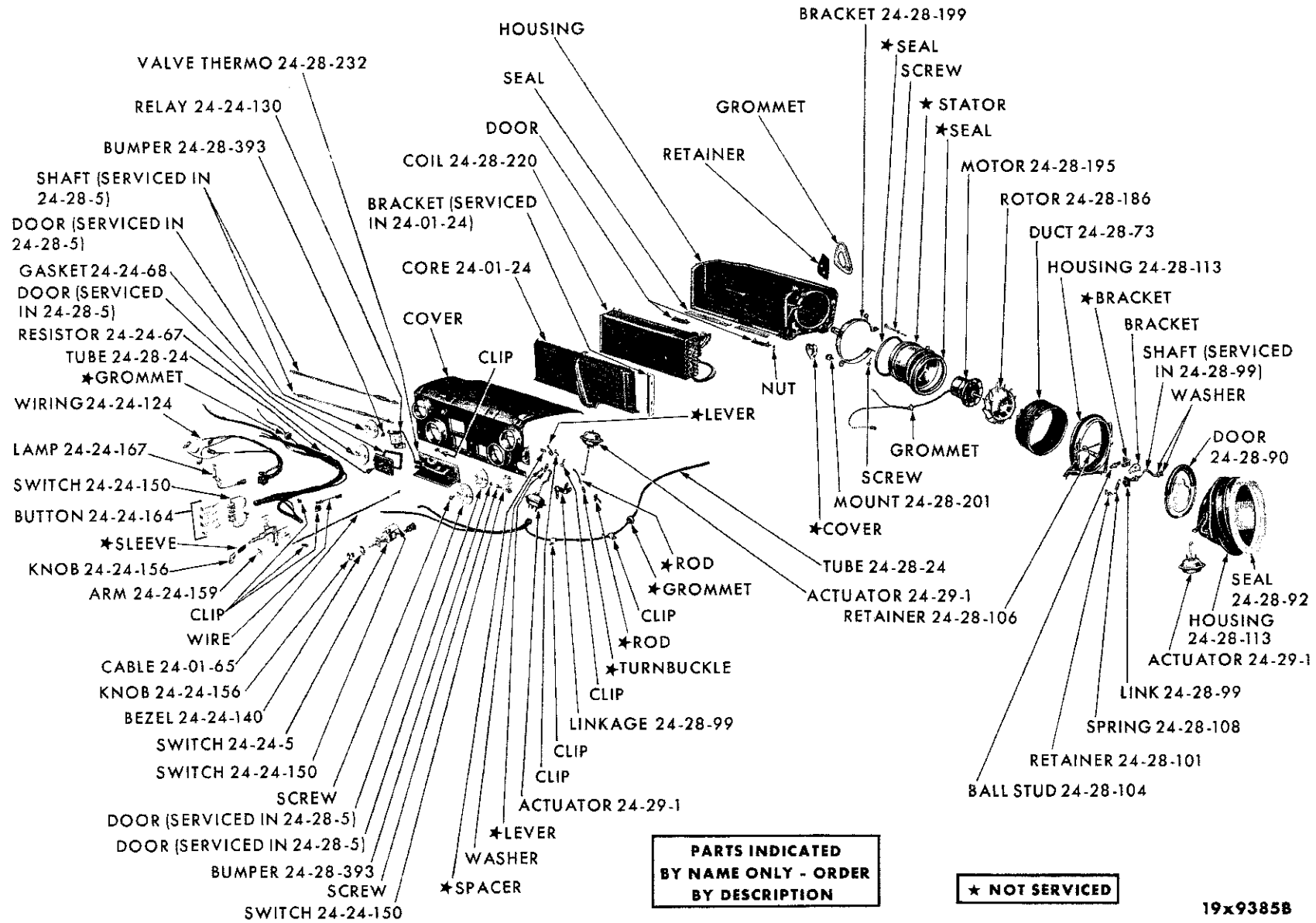
AIR CONDITIONING SYSTEM (COWL TYPE) - PLYMOUTH SP1-2 AND DART SD1-2
