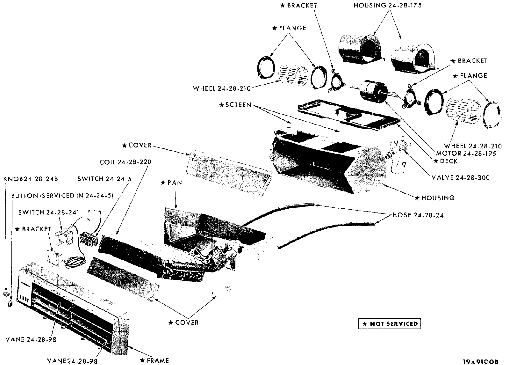
AIR CONDITIONING EVAPORATOR - MOPAR MODEL "G"
