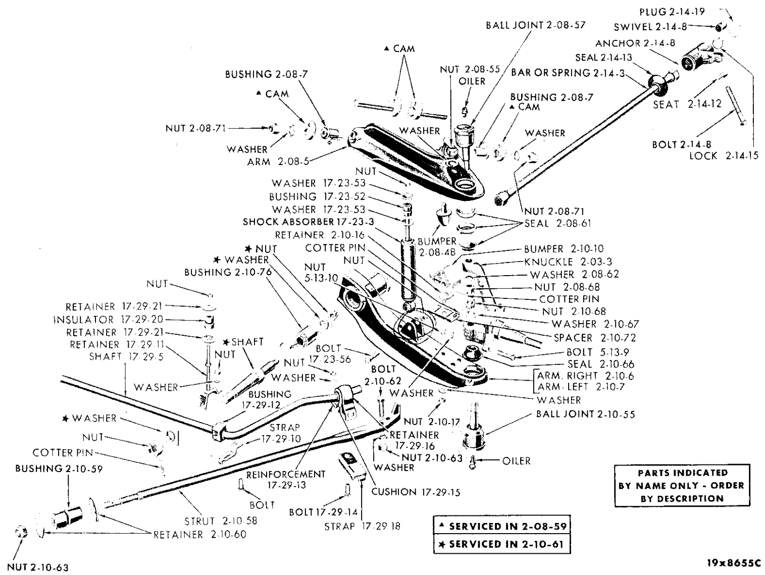
FRONT SUSPENSION - EXCEPT VALIANT RV1
