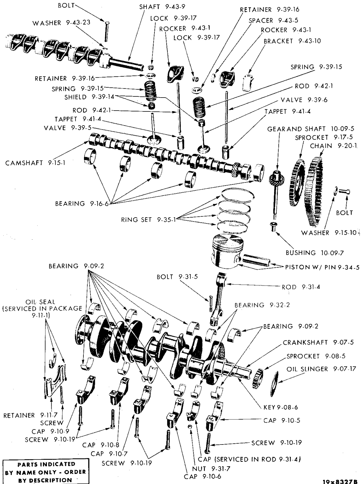
ENGINE INTERNAL PARTS - V8 CYLINDER ("B" ENGINE)
