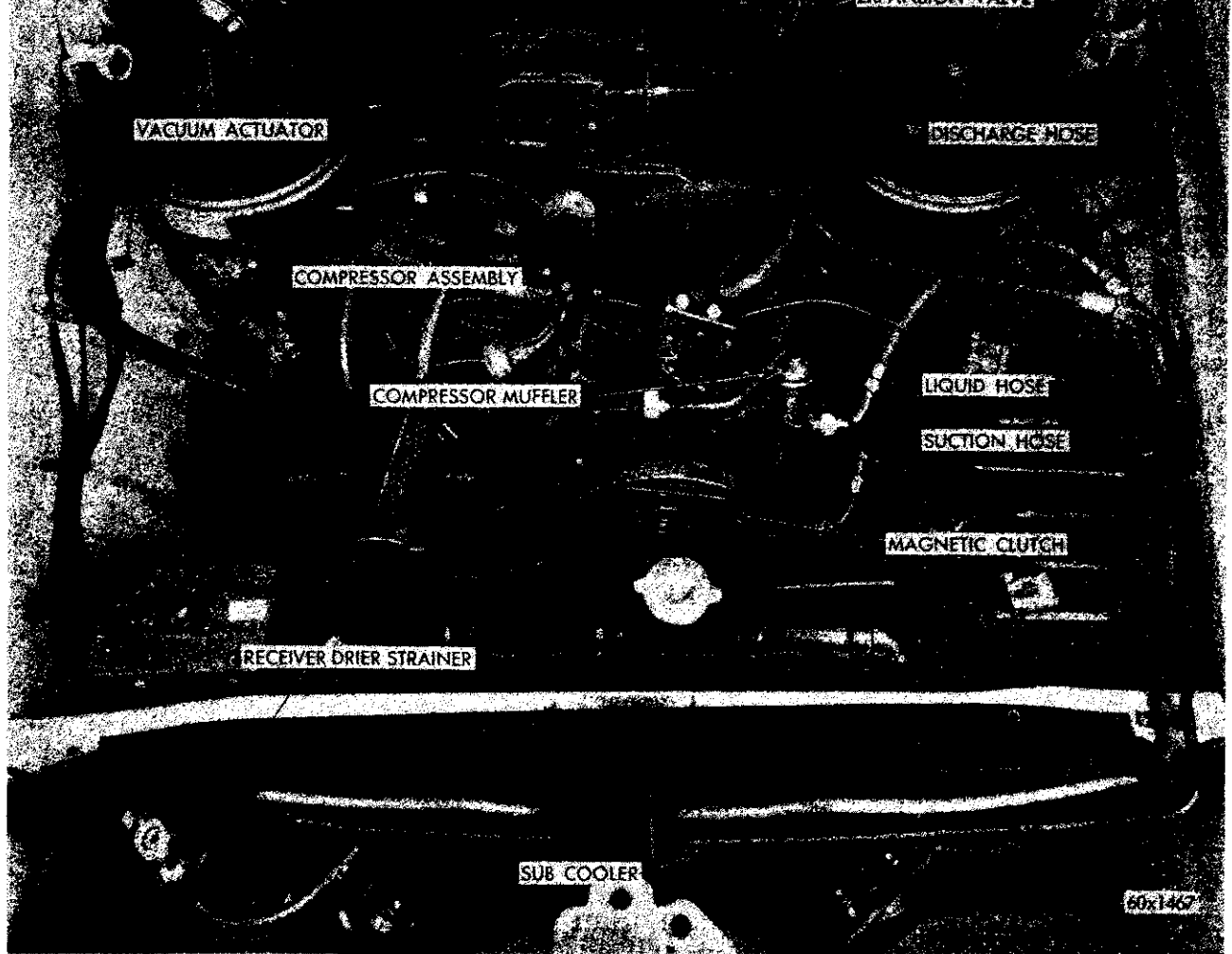
Fig. 19 Air Conditioning System Installed
