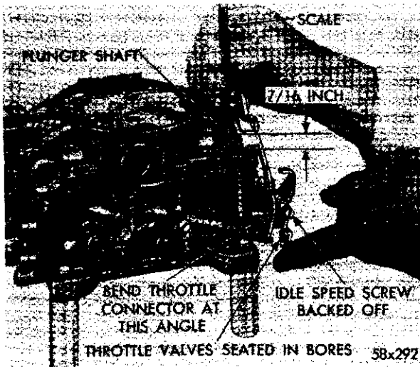
Fig. 9 Checking Accelerator Pump Travel
