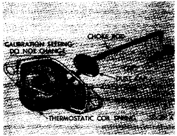
Fig. 12 Choke Control Unit (Cross-over)
