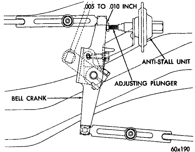
Fig. 16 Anti-Stall Adjustment
