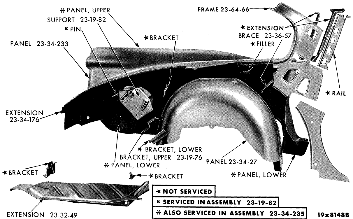
REAR QUARTER PANEL - IMPERIAL PY1 4 DOOR SEDAN
