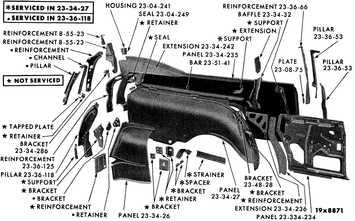
REAR QUARTER PANEL - PLYMOUTH PP1-2 2 DOOR SUBURBAN
