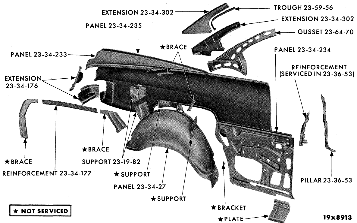
REAR QUARTER PANEL - DODGE PD3-4 SPECIAL CLUB COUPE
