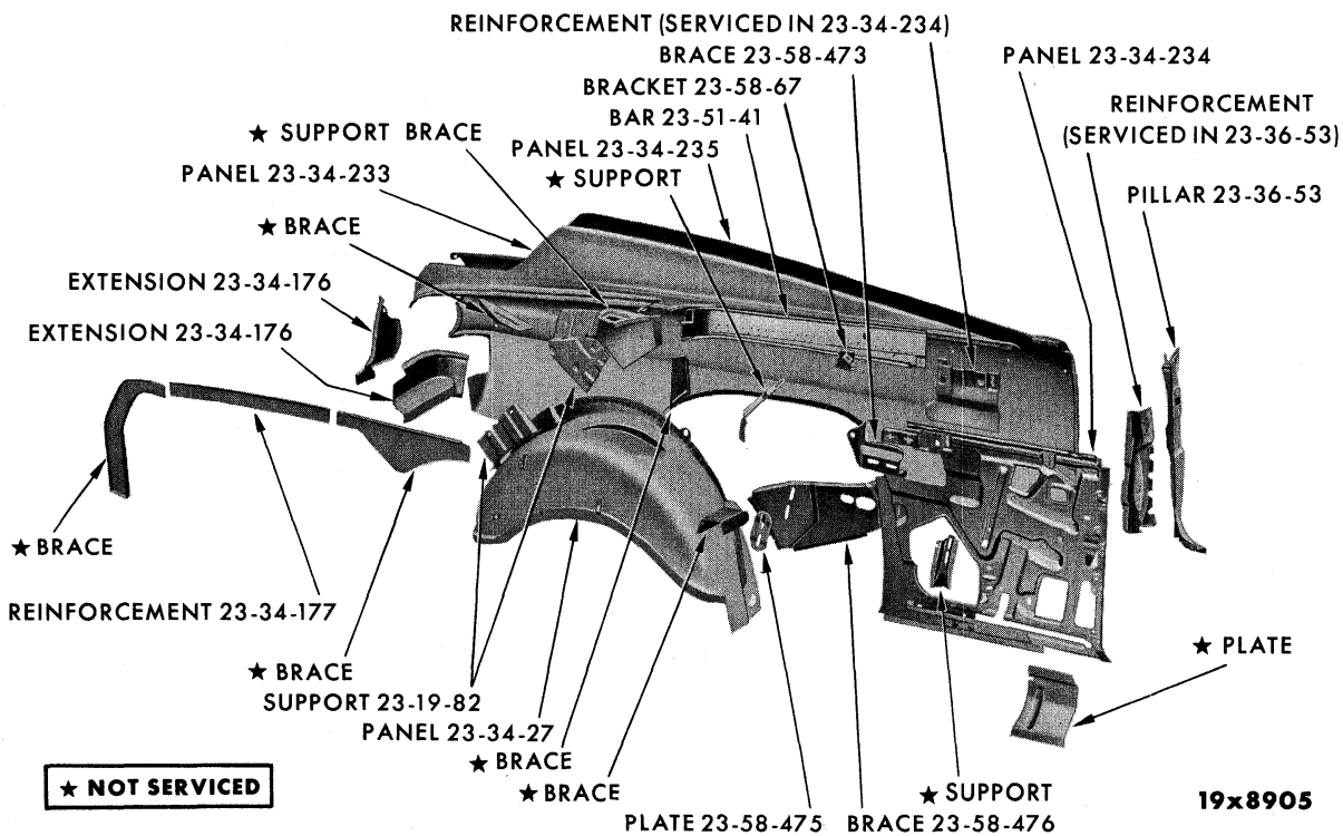
REAR QUARTER PANEL - DODGE PD1-2 CONVERTIBLE COUPE
