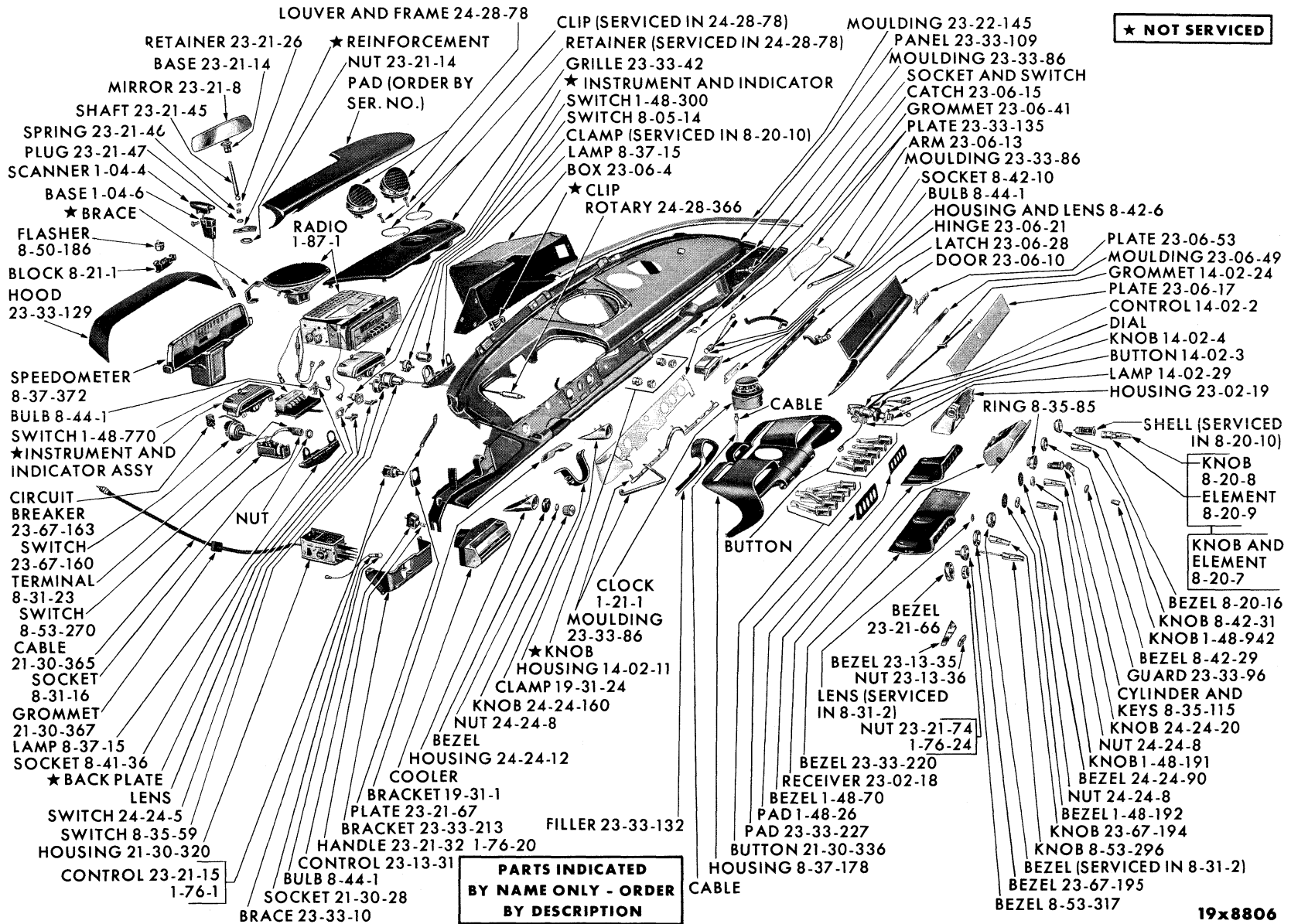
INSTRUMENT PANEL - DODGE PD1-2-3-4
