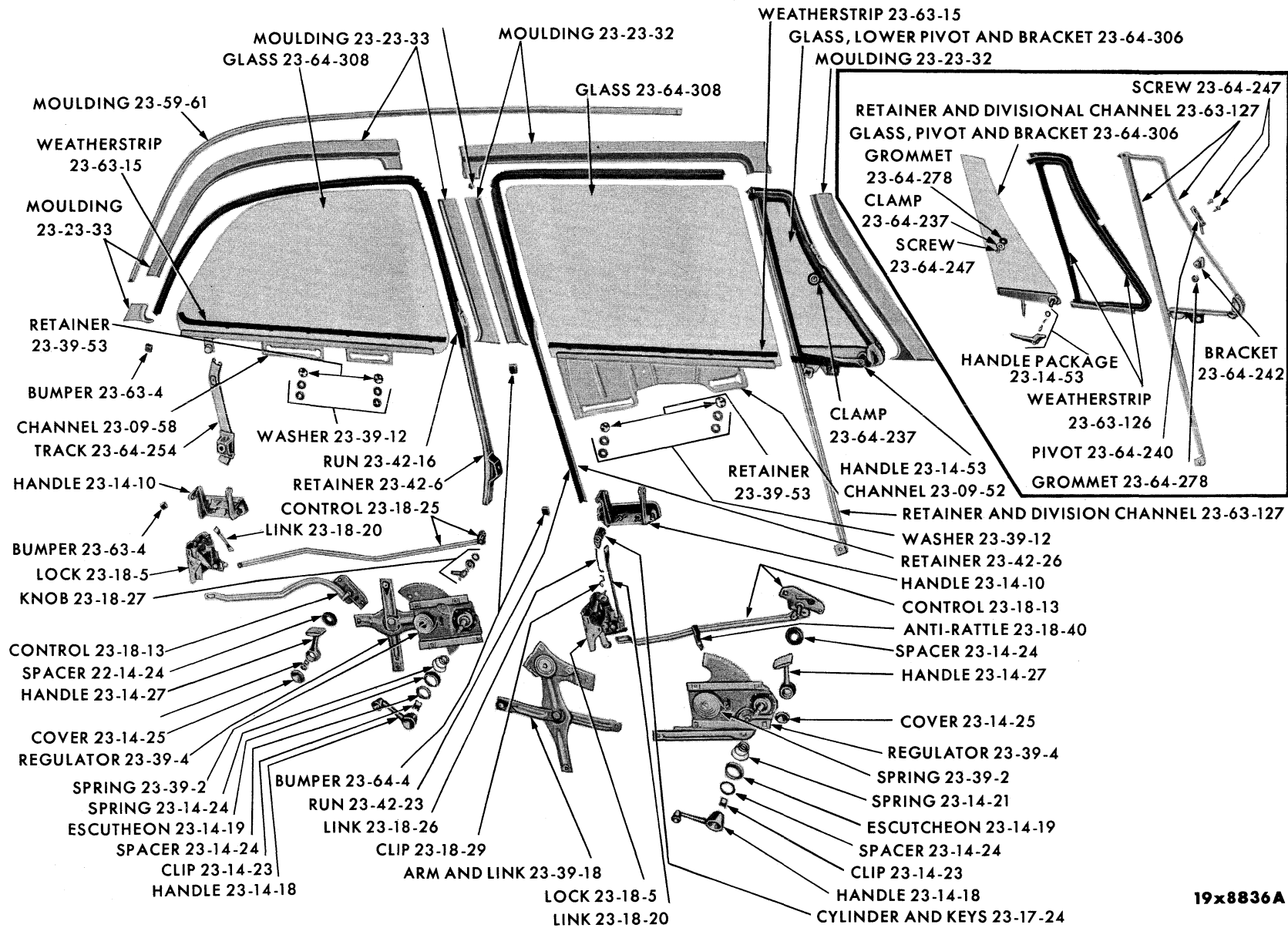
WINDOWS, REGULATORS AND RUNS - PLYMOUTH PP1-2 4 DOOR SEDAN
