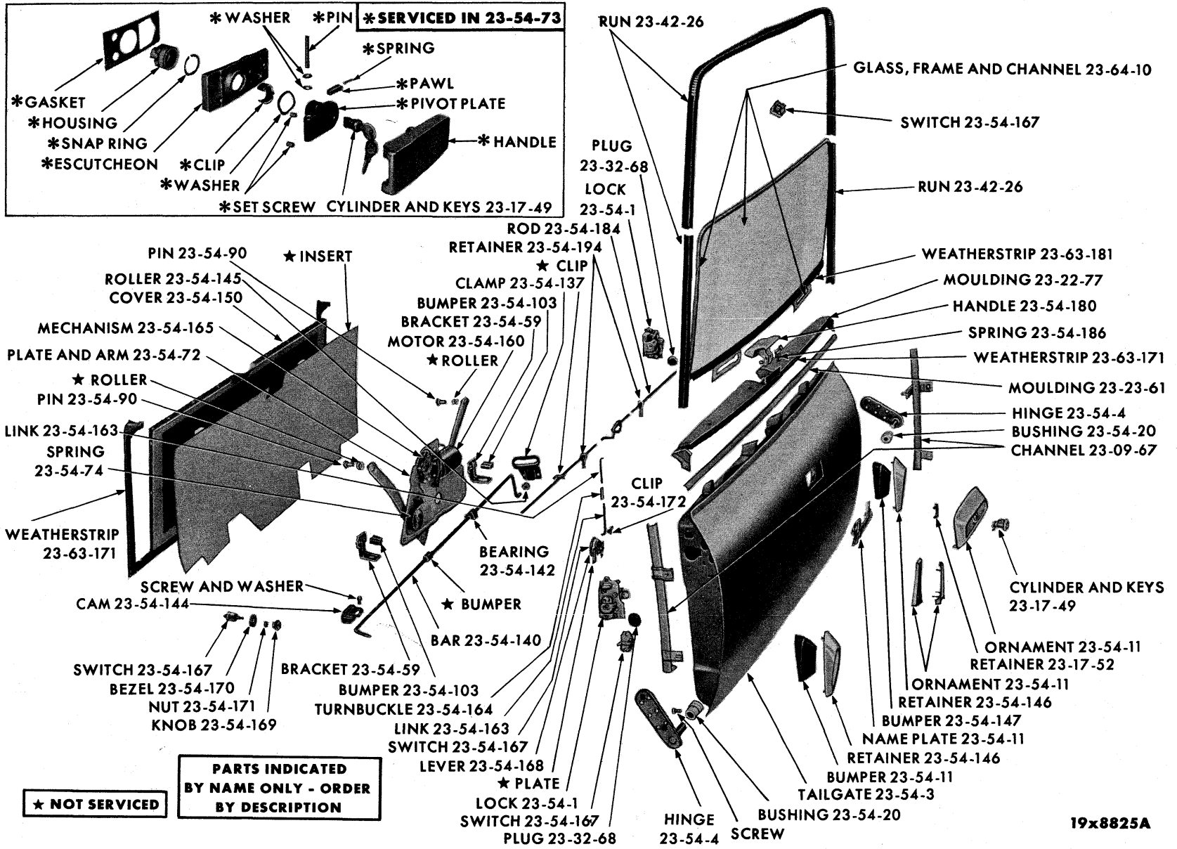
TAILGATE - SUBURBANS
