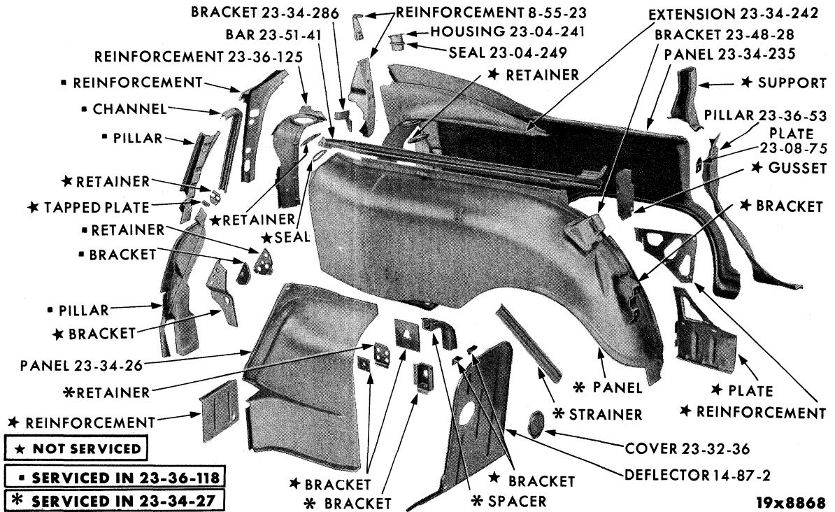
REAR QUARTER PANEL - PLYMOUTH PP1-2 4 DOOR SUBURBAN (LEFT-GAS TANK SIDE)
