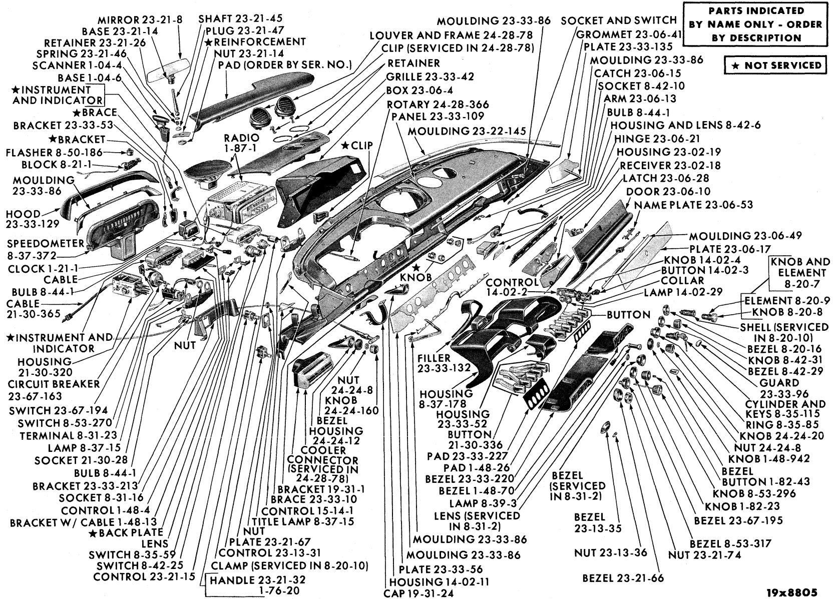
INSTRUMENT PANEL - DESOTO PS1-3
