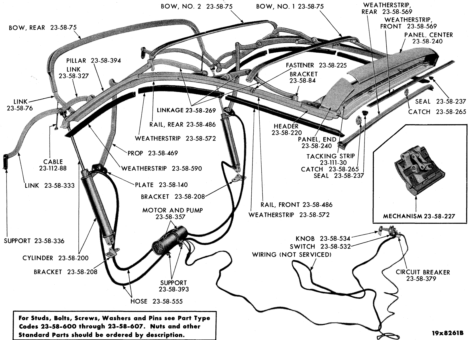
CONVERTIBLE COUPE FOLDING TOP - EXCEPT IMPERIAL PY1
