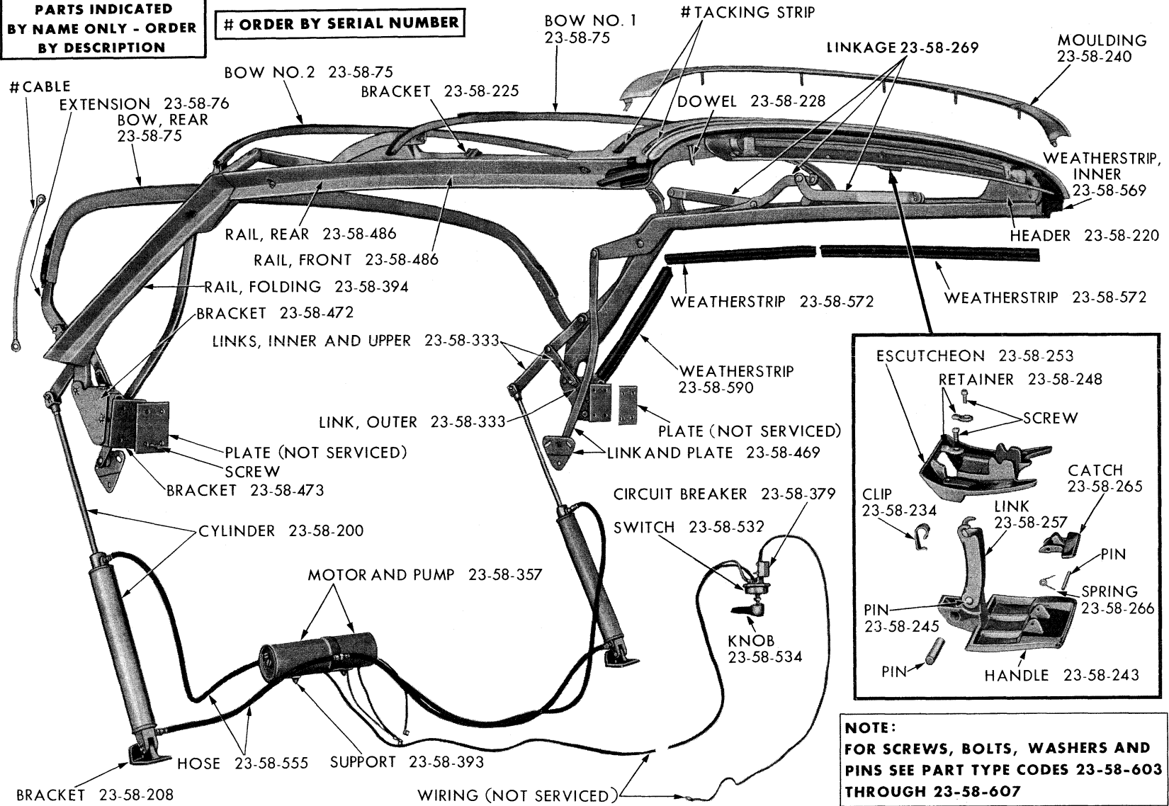
CONVERTIBLE COUPE FOLDING TOP - IMPERIAL PY1
