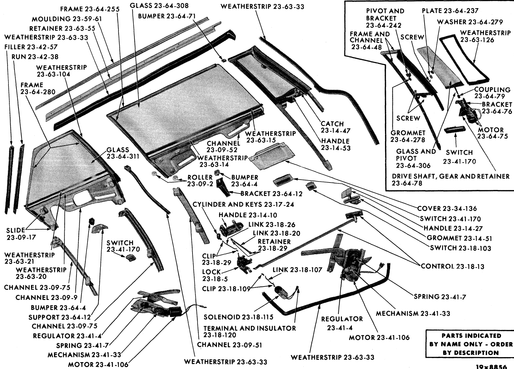
WINDOWS, REGULATORS AND RUNS - IMPERIAL PY1 SPECIAL CLUB COUPE
