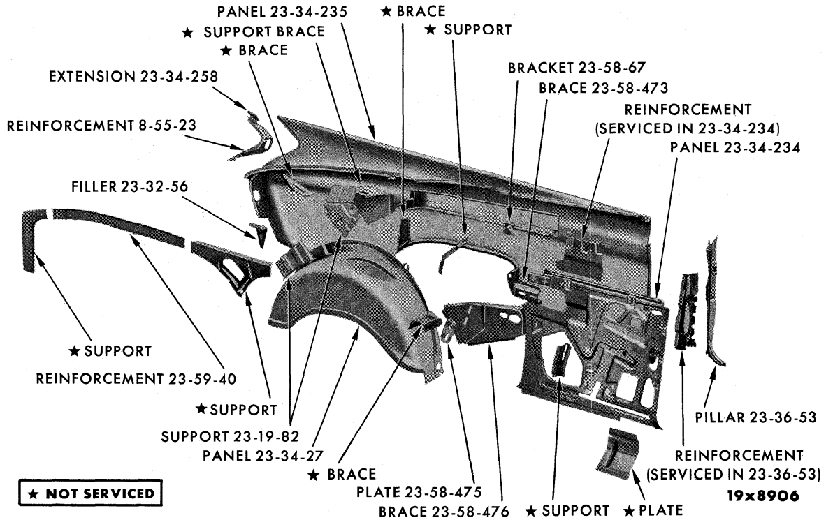
REAR QUARTER PANEL - CHRYSLER PC1-3-4 CONVERTIBLE COUPE
