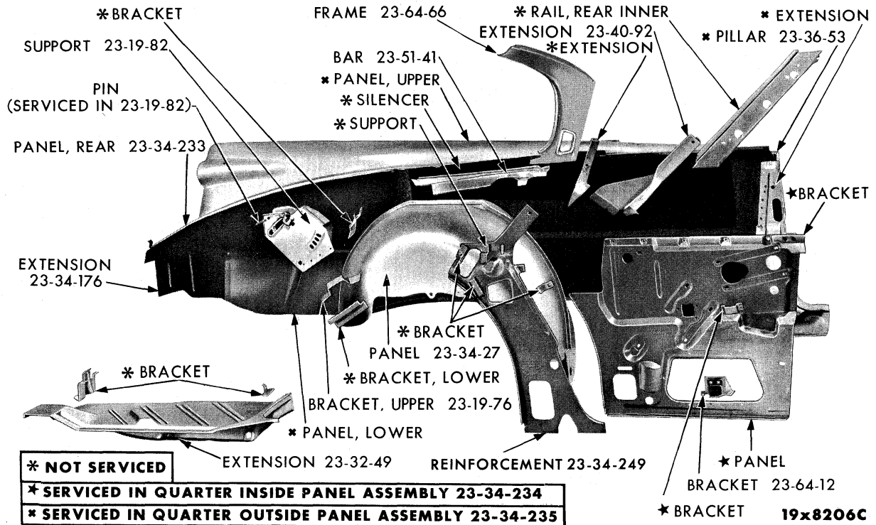
REAR QUARTER PANEL - IMPERIAL PY1 SPECIAL CLUB COUPE
