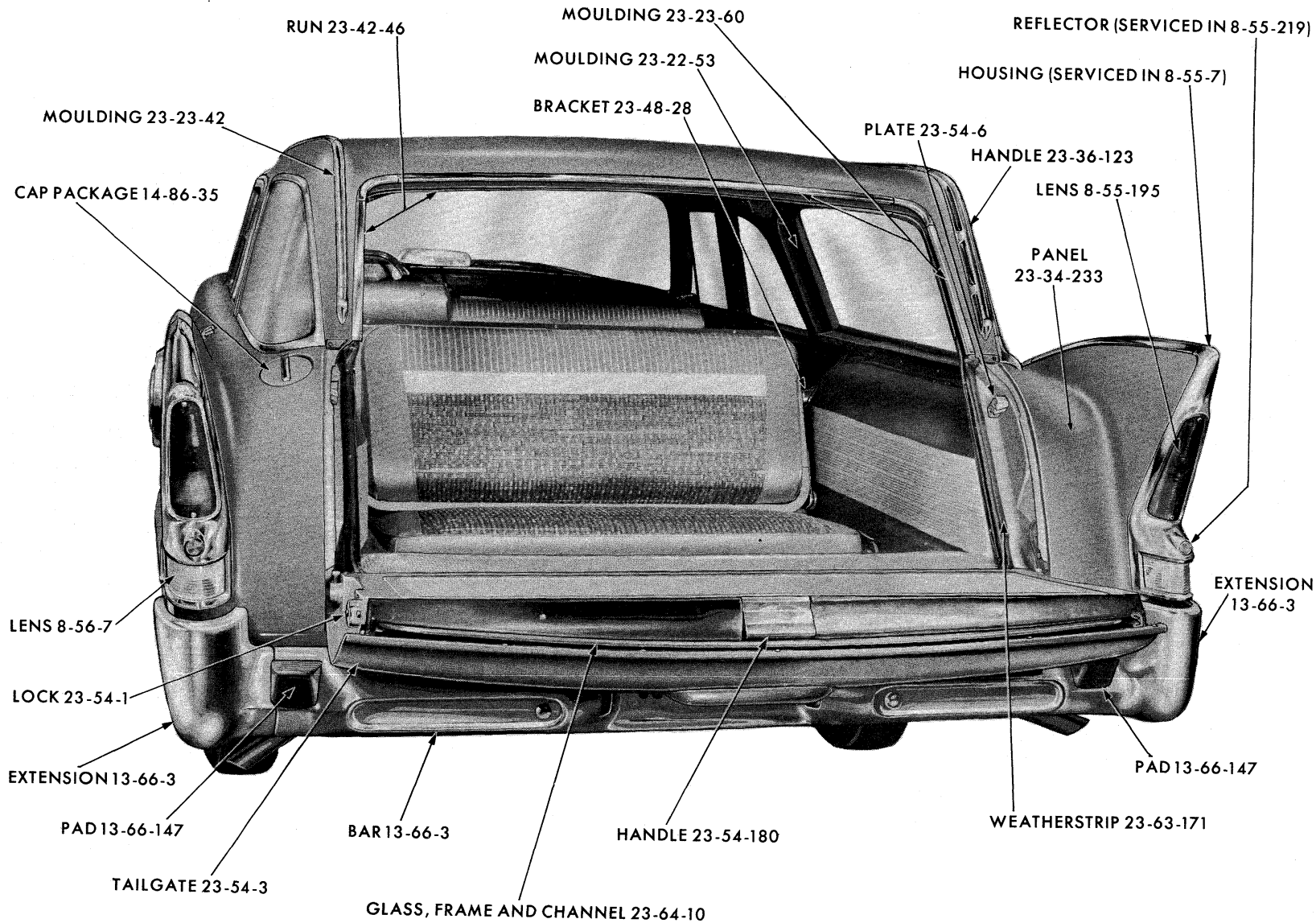
REAR VIEW - PLYMOUTH PP1-2 SUBURBAN
