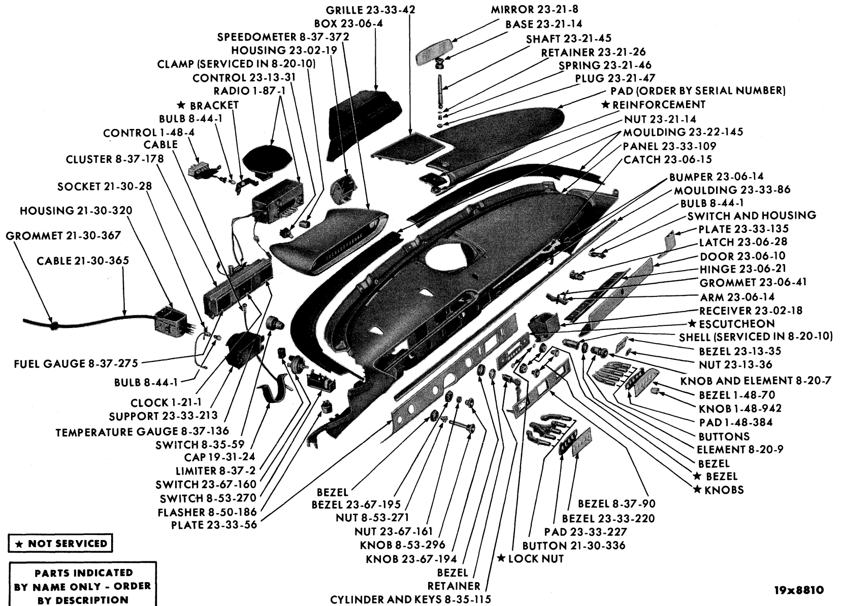
INSTRUMENT PANEL - PLYMOUTH PP1-2
