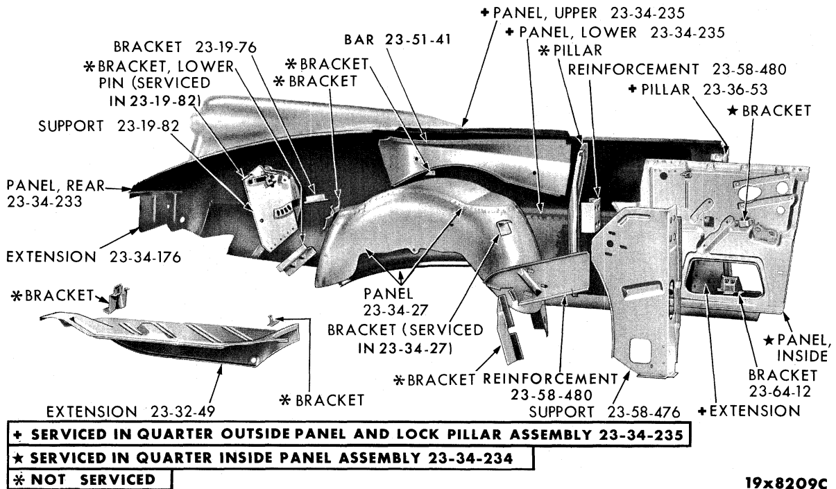
REAR QUARTER PANEL - IMPERIAL PY1 CONVERTIBLE COUPE
