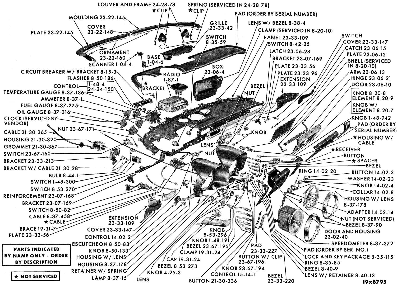
INSTRUMENT PANEL - IMPERIAL PY1
