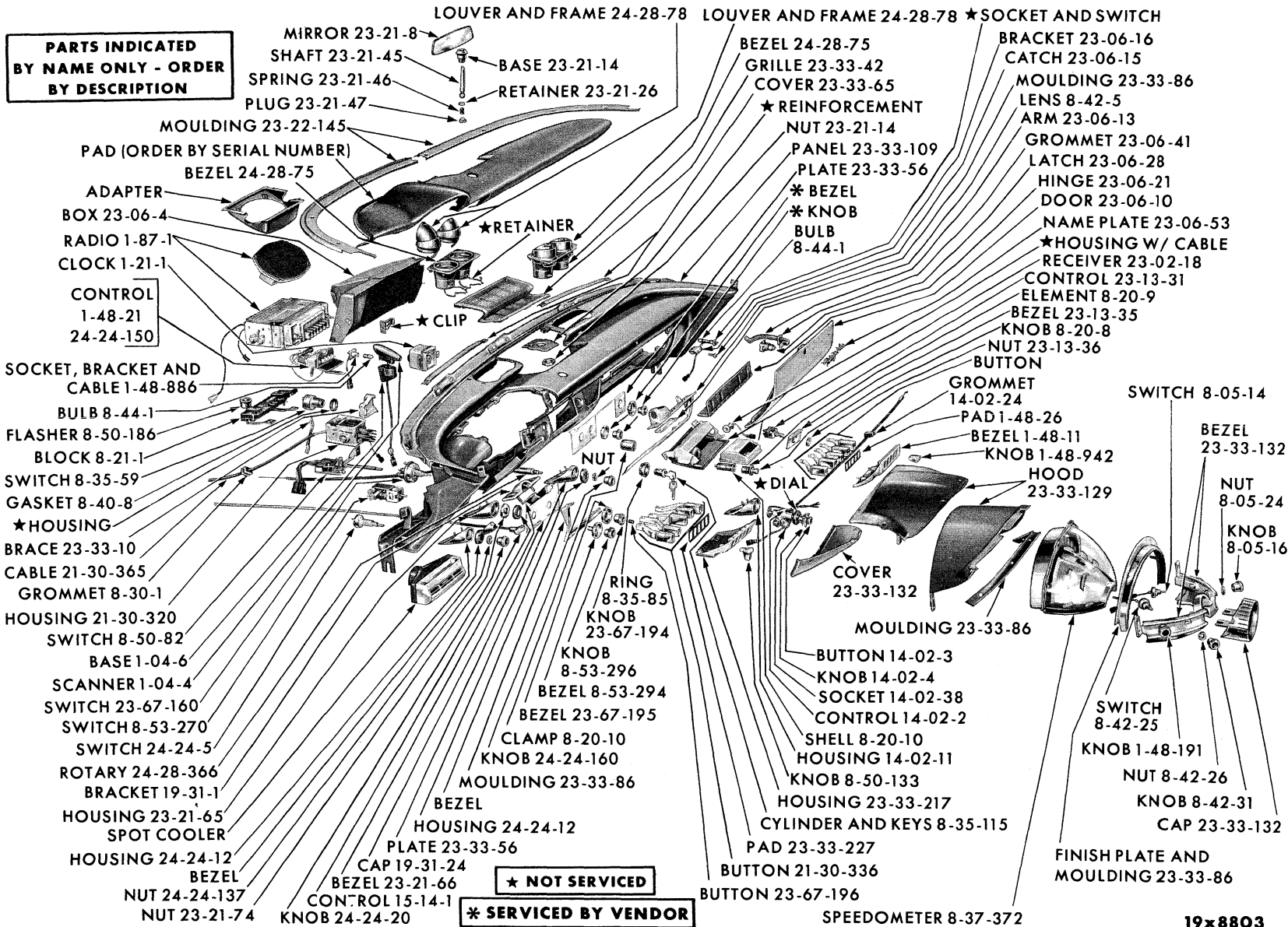
INSTRUMENT PANEL - CHRYSLER PC1-2-3
