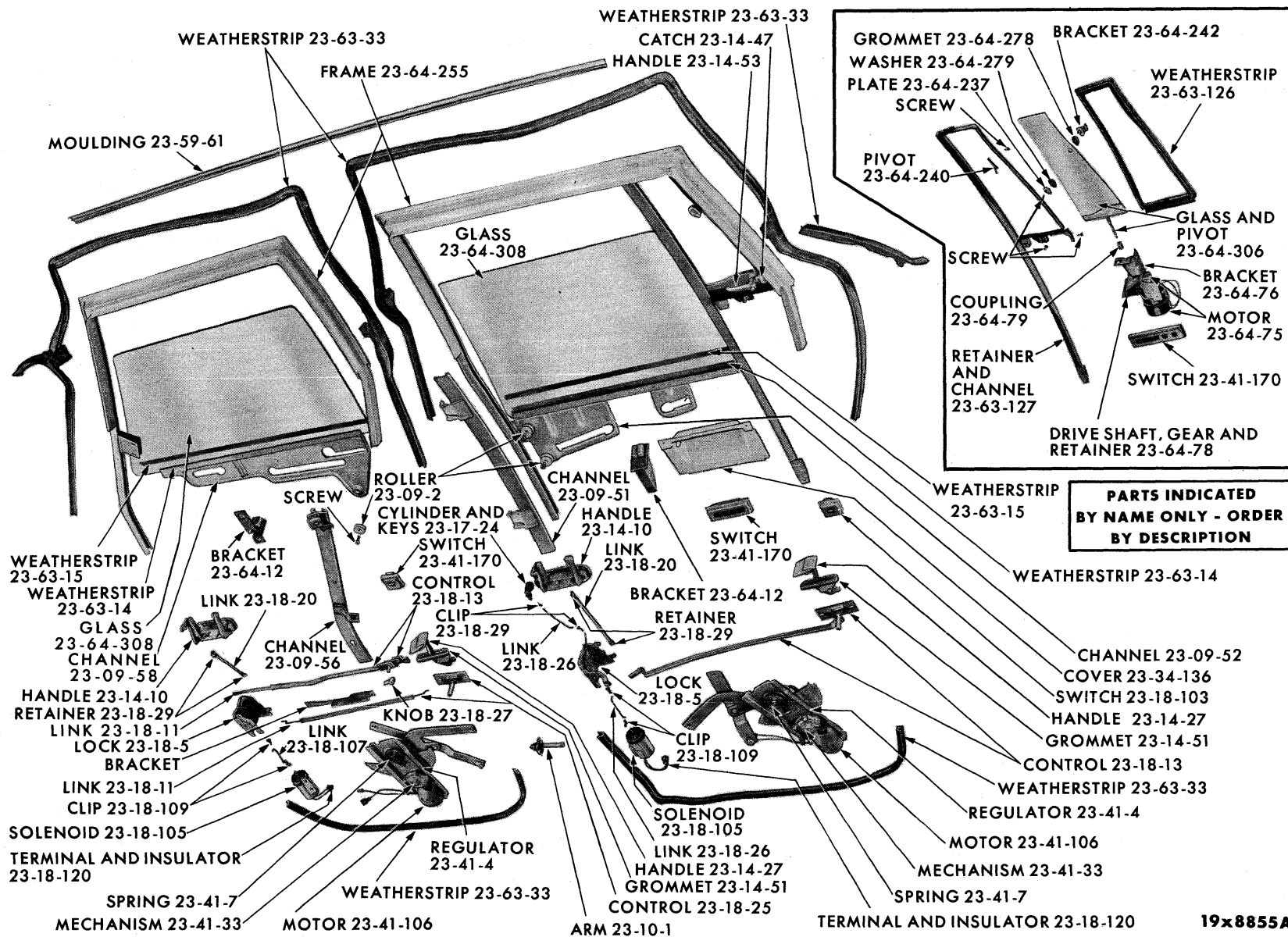
WINDOWS, REGULATORS AND RUNS - IMPERIAL PY1 4 DOOR SEDAN
