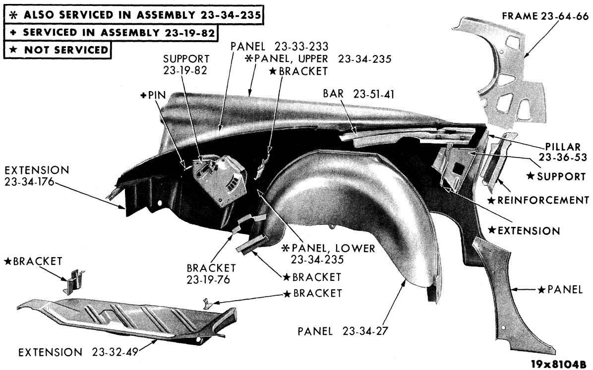
REAR QUARTER PANEL - IMPERIAL PY1 SPECIAL 4 DOOR SEDAN
