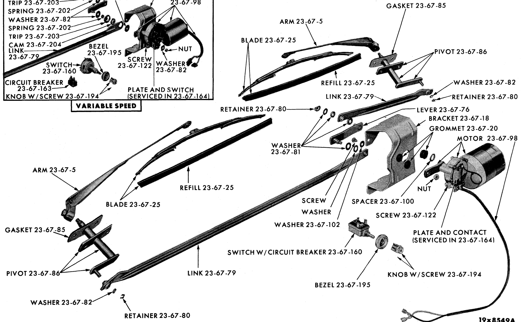
WINDSHIELD WIPER - EXCEPT IMPERIAL PY1
