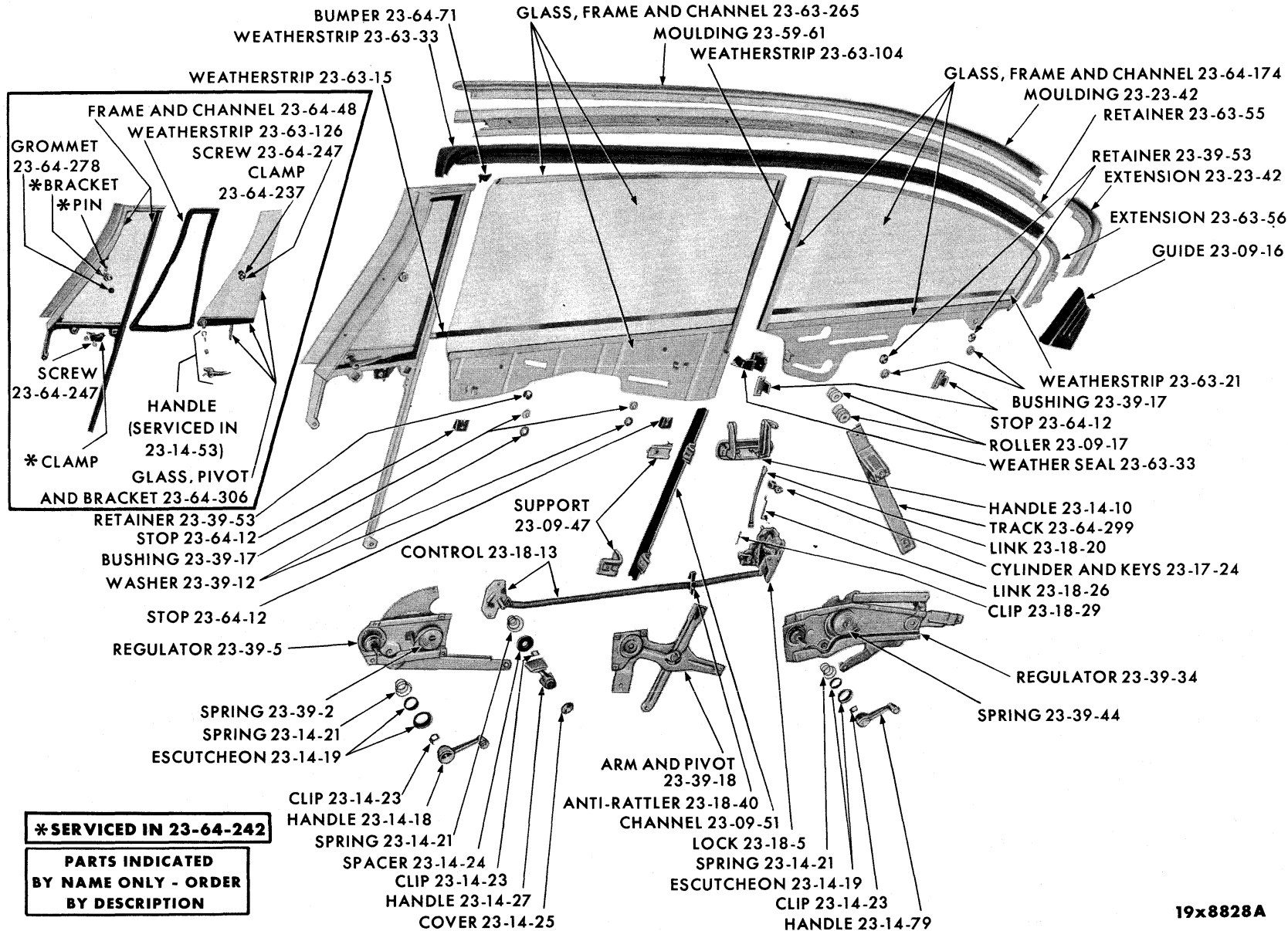
WINDOWS, REGULATORS AND RUNS - PLYMOUTH PP1-2 SPECIAL CLUB COUPE
