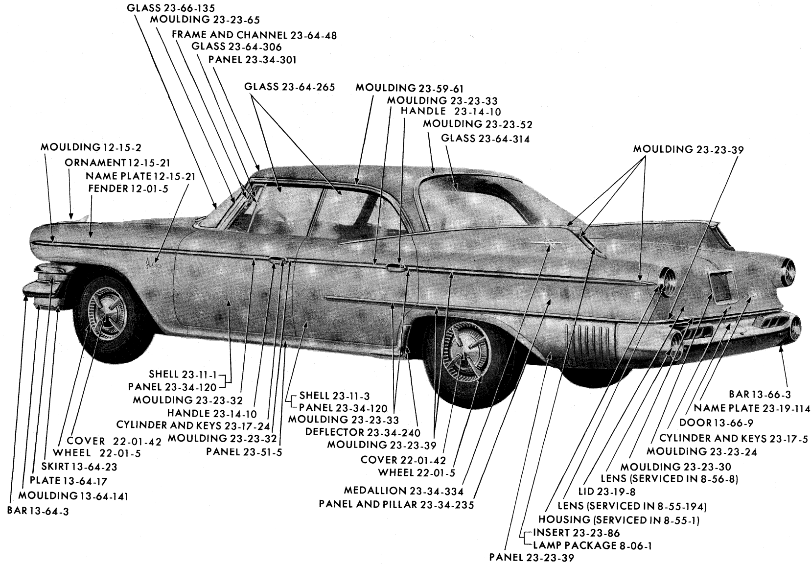
REAR EXTERIOR - DODGE PD1-2 SPECIAL 4 DOOR SEDAN
