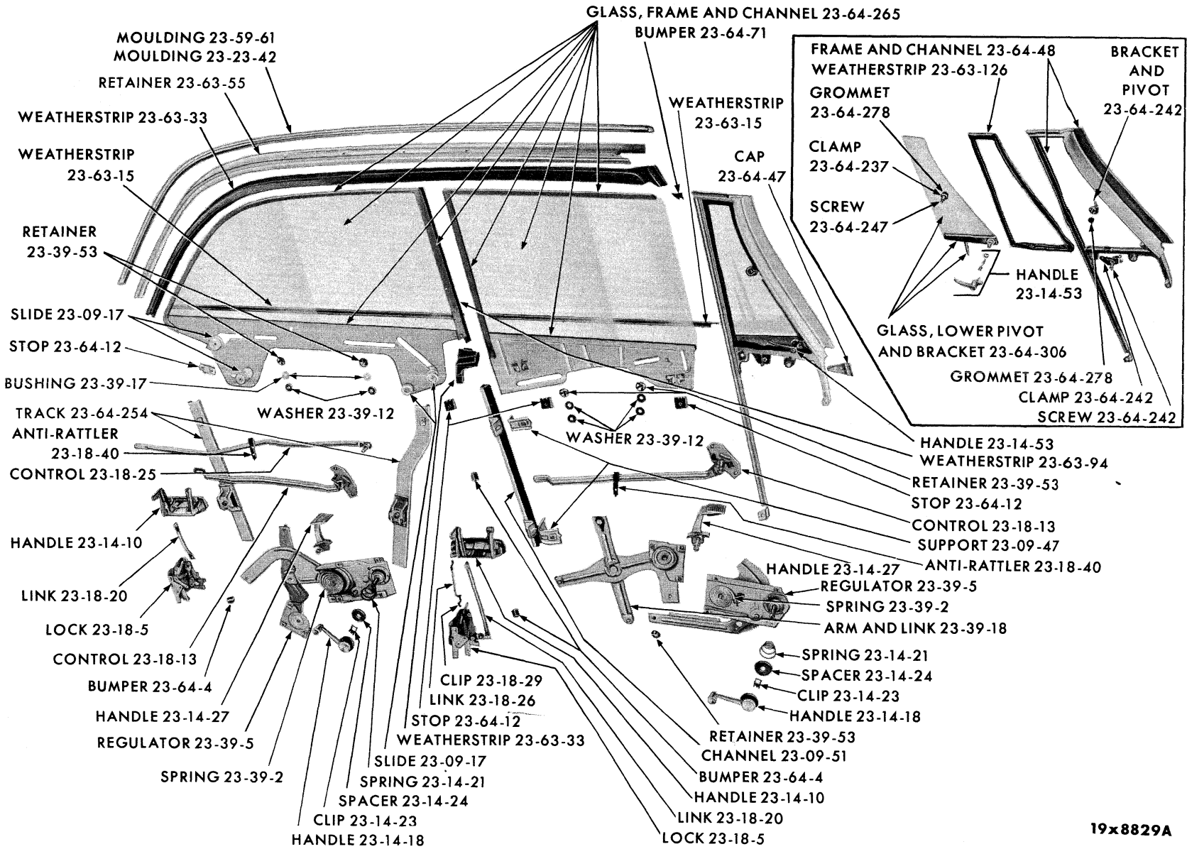
WINDOWS, REGULATORS AND RUNS - DODGE PD1-2-3-4, DESOTO PS1-3 AND CHRYSLER PC1-2-3 SPECIAL 4 DOOR SEDAN
