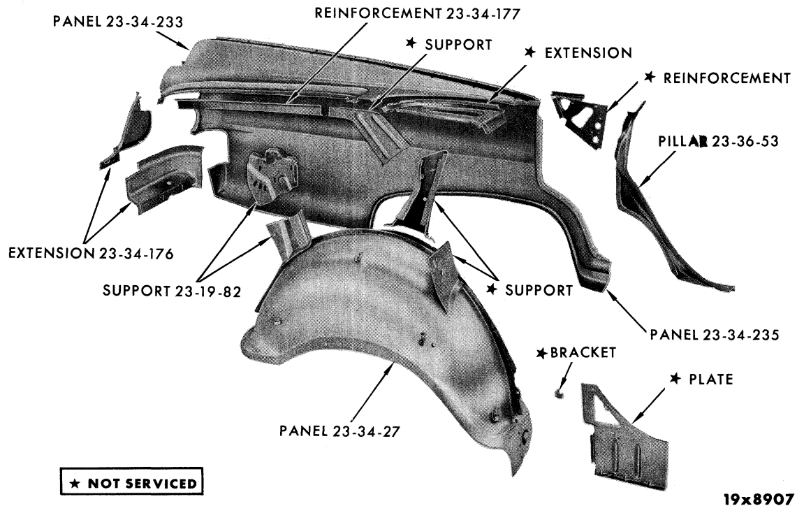
REAR QUARTER PANEL - DODGE PD3-4 4 DOOR SEDAN AND SPECIAL 4 DOOR SEDAN
