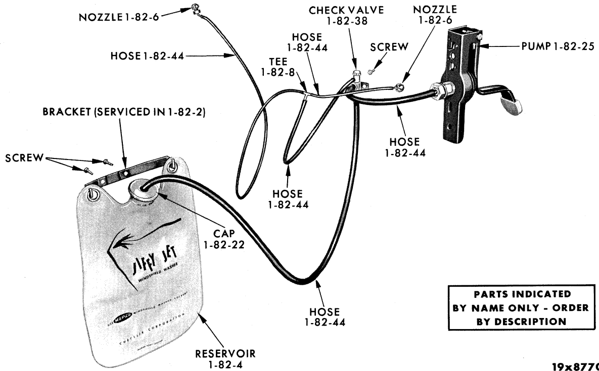
FOOT-CONTROLLED WINDSHIELD WASHER SYSTEM
