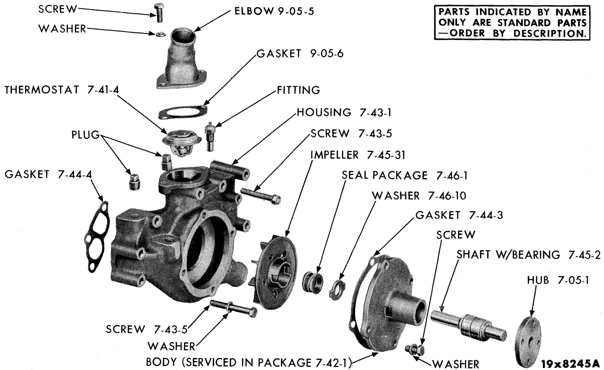
WATER PUMP - V8 CYLINDER (EXCEPT PLYMOUTH MP2) WITHOUT AIR CONDITIONING
