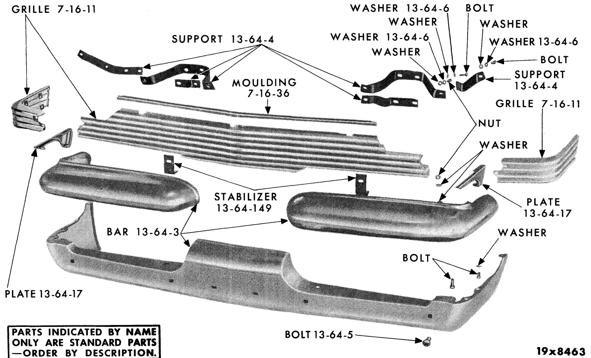
GRILLE AND FRONT BUMPER - CHRYSLER MC1-2-3
