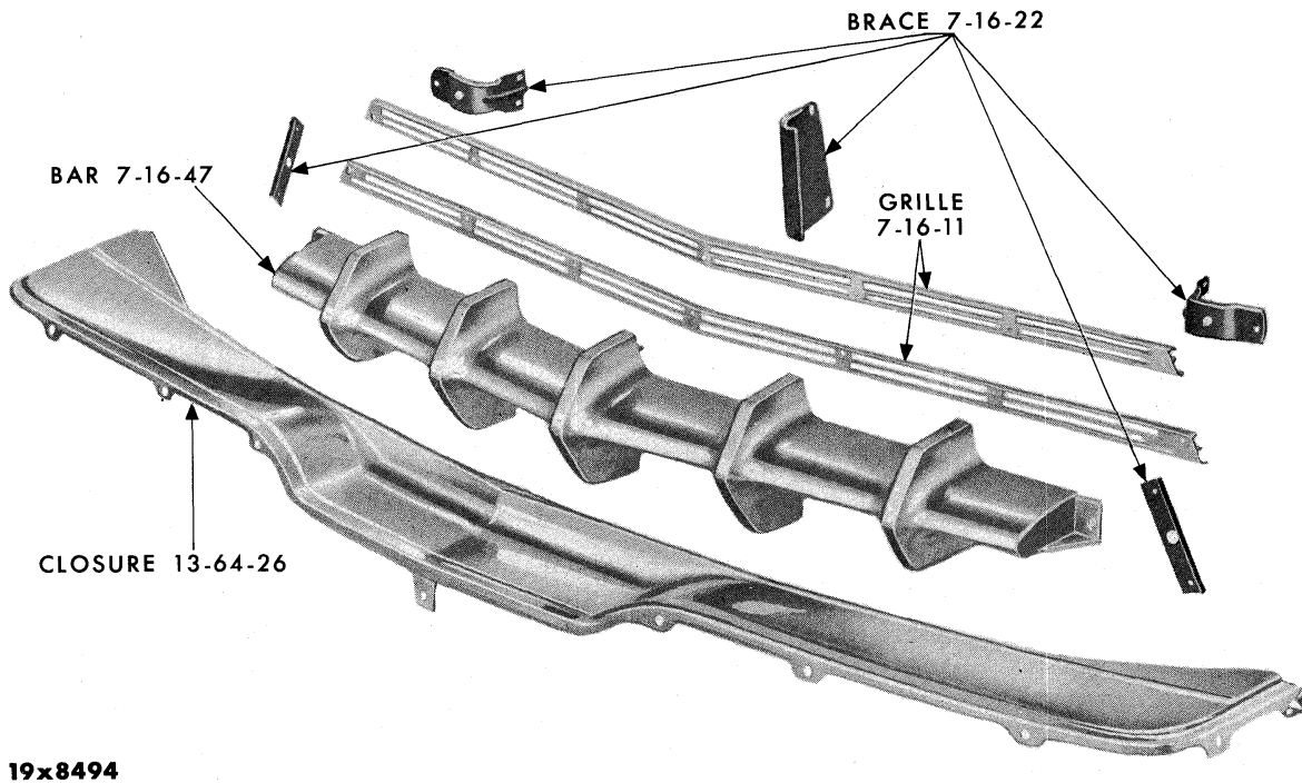
GRILLE - IMPERIAL MY1
