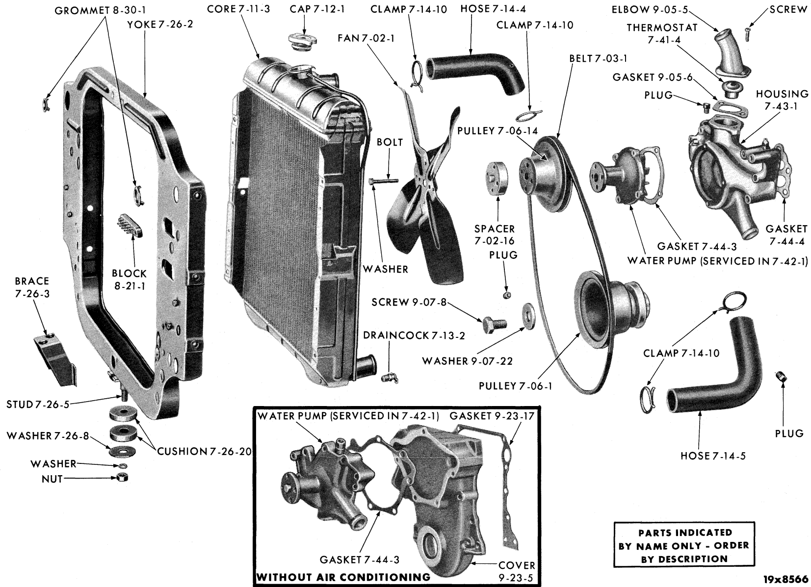
COOLING SYSTEM - DODGE MD2
