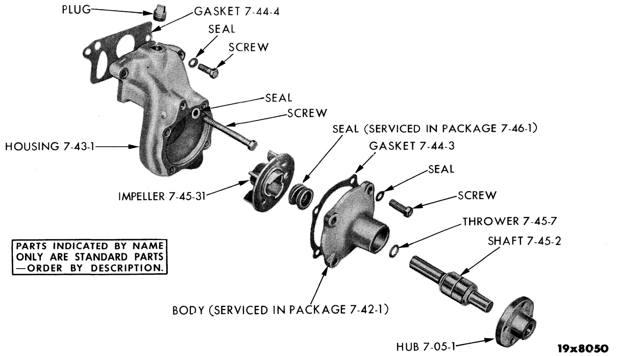
WATER PUMP - 6 CYLINDER
