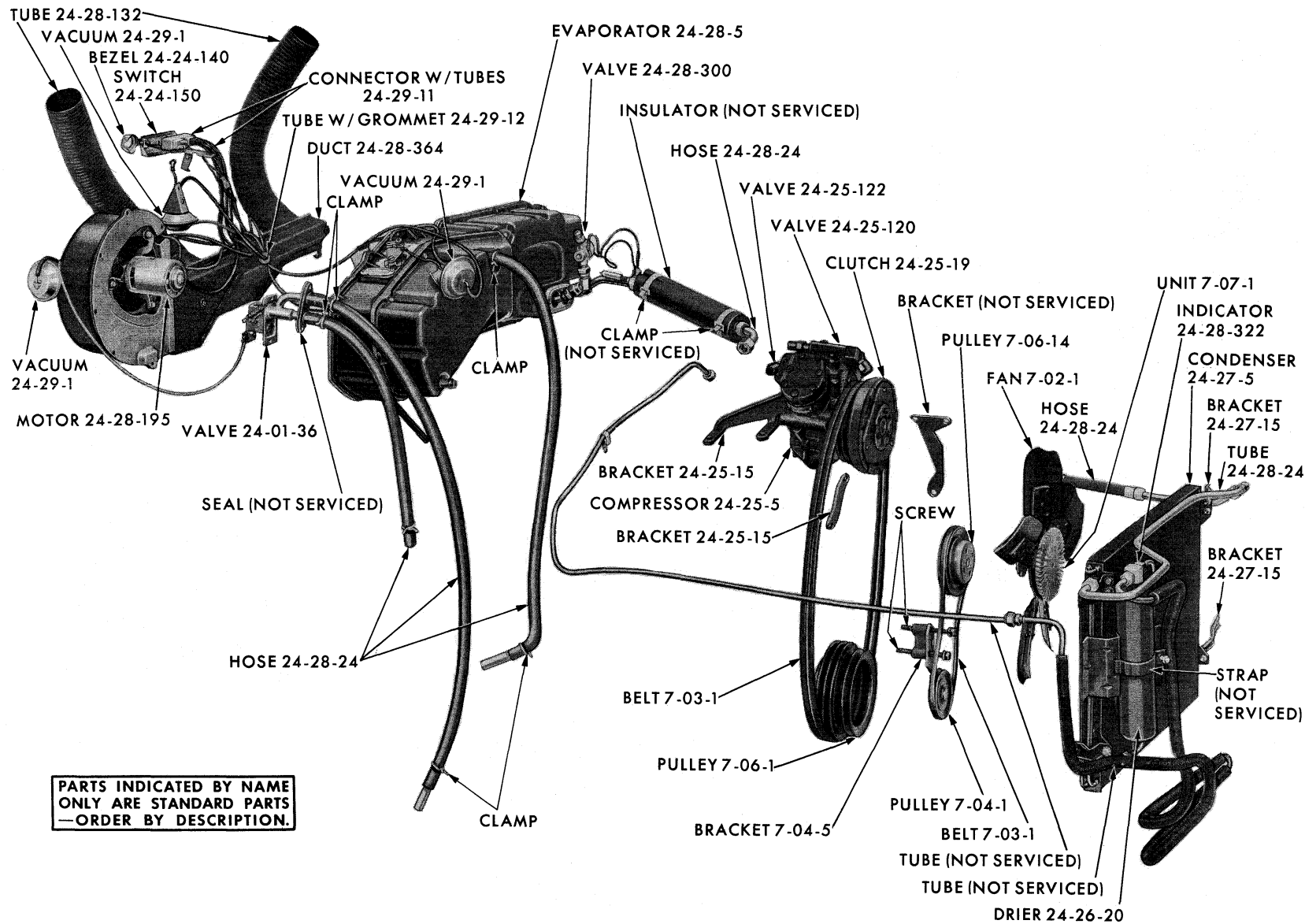
AIR CONDITIONING SYSTEM - COWL TYPE
