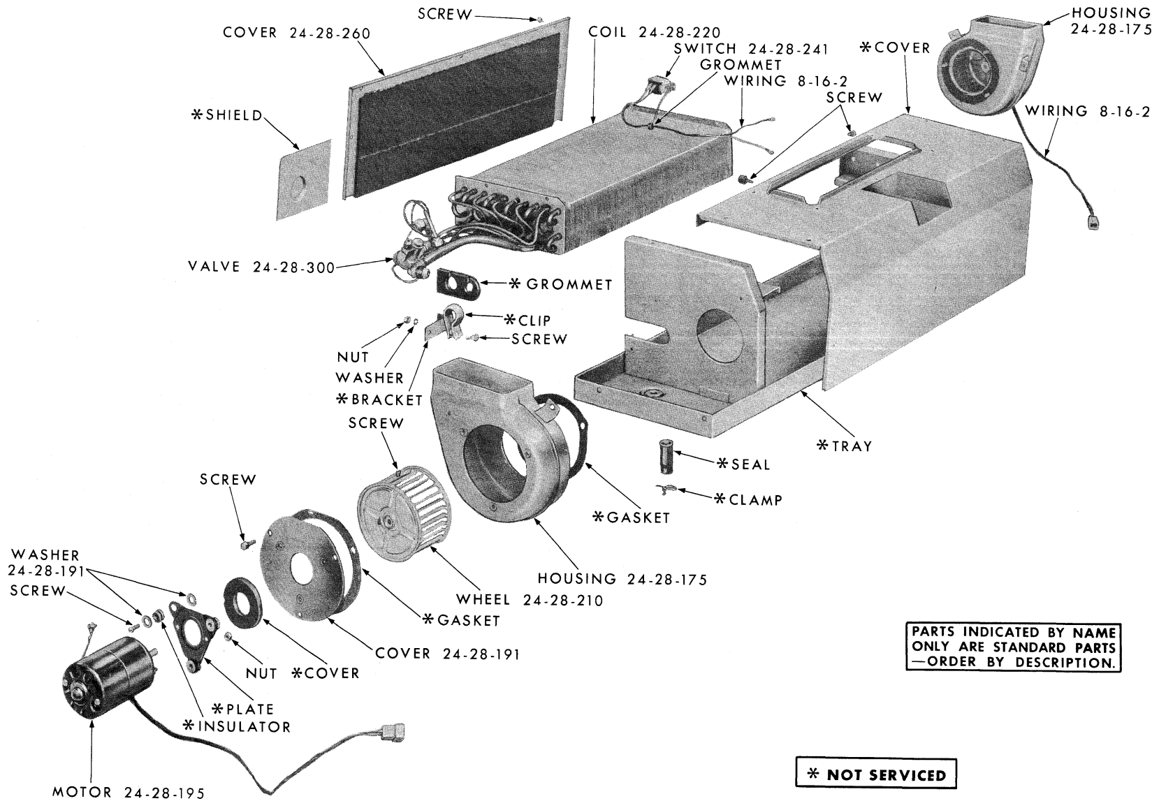
AIR CONDITIONING EVAPORATOR - TRUNK UNIT
