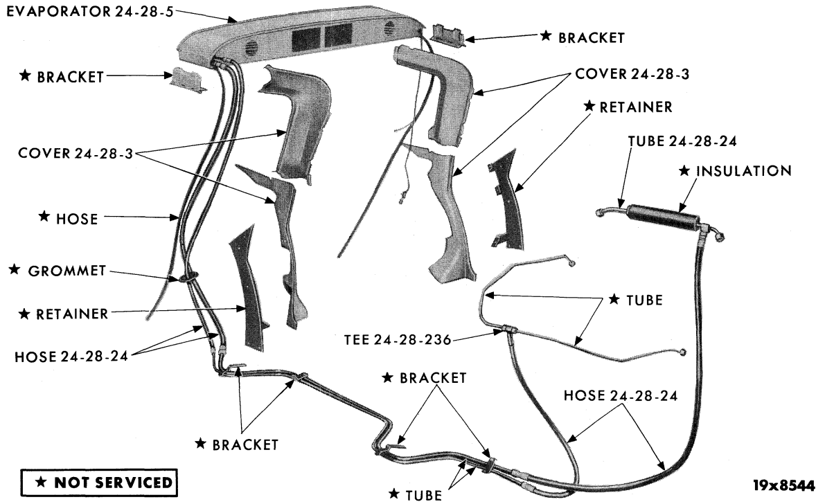
AIR CONDITIONING SYSTEM - SUBURBANS
