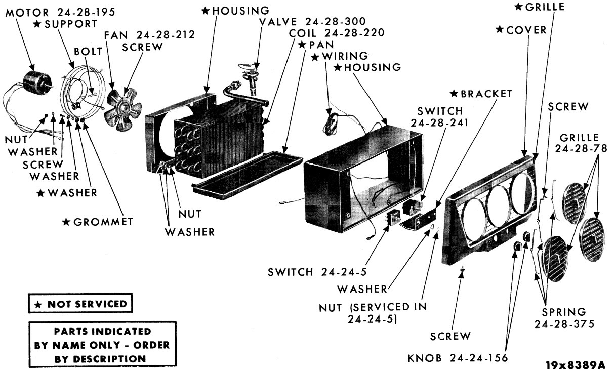
AIR CONDITIONING EVAPORATOR - MODEL "D"
