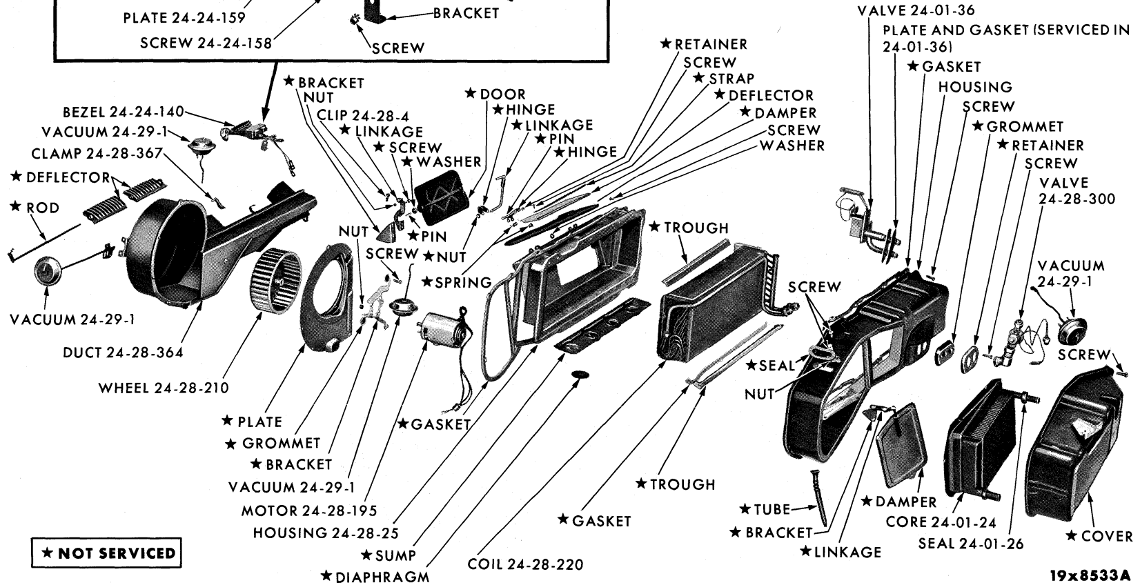
HEATER AND AIR CONDITIONING SYSTEM - MODEL 903
