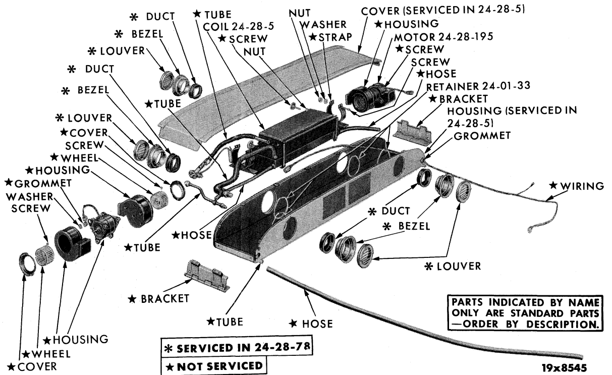
AIR CONDITIONING EVAPORATOR - SUBURBANS
