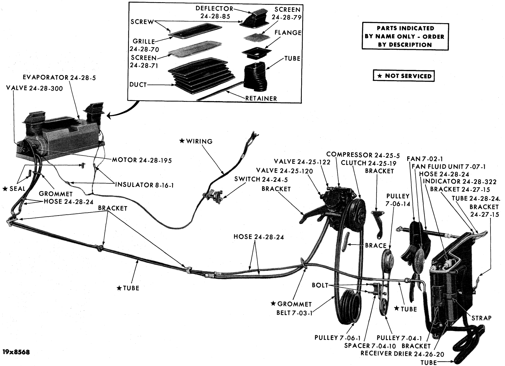
AIR CONDITIONING SYSTEM - TRUNK UNIT
