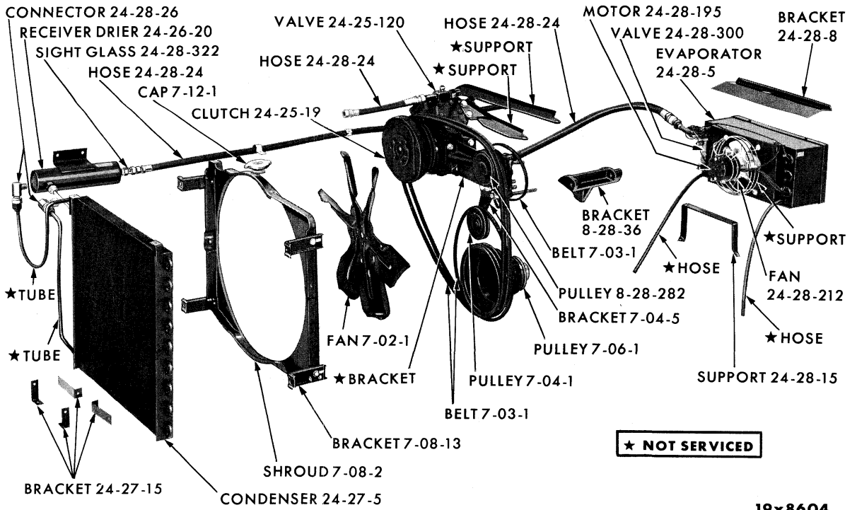
AIR CONDITIONING SYSTEM - MODEL "D"
