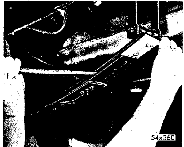
Fig. 9—Positioning New Interliners
