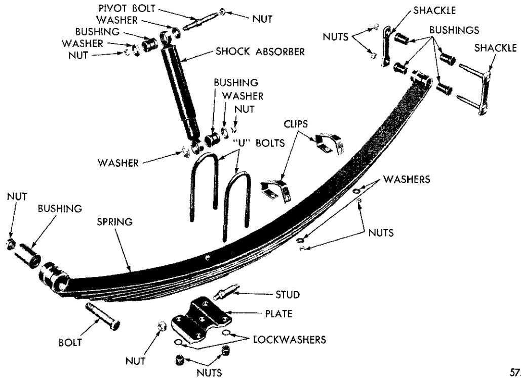
Fig. 4—Typical Rear Springs Suspension (Disassembled View)
