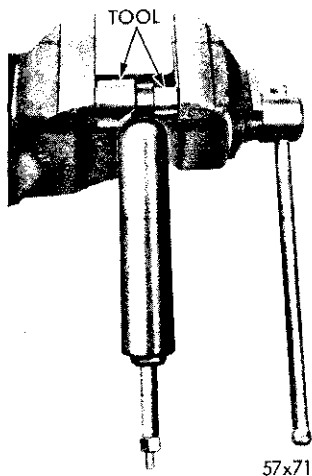
Fig. 13—Installing Shock Absorber Eye Bushing
