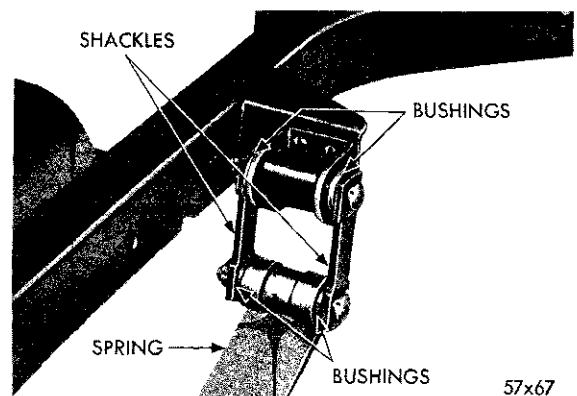
Fig. 6—Rear Spring Shackles
