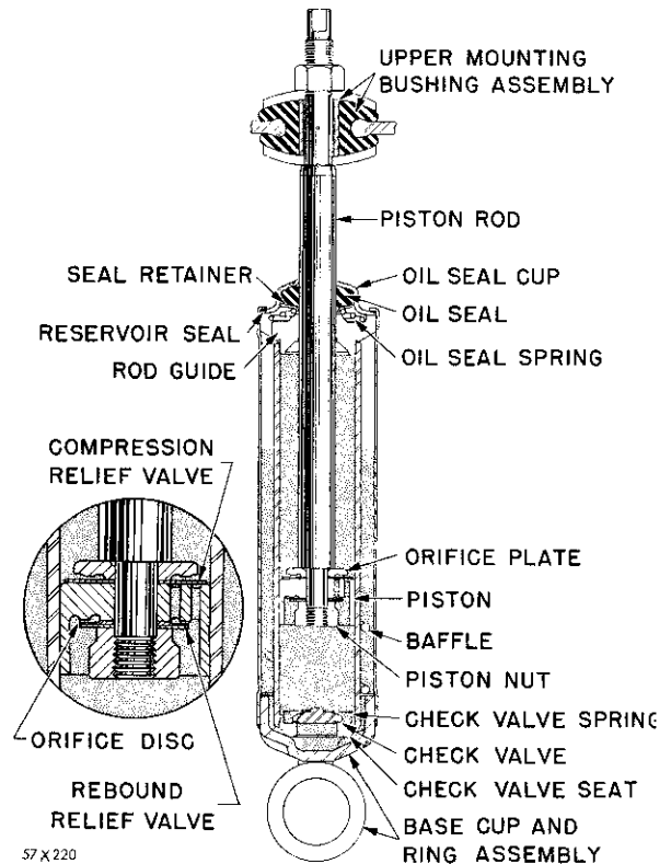
Fig. 12—Front Shock Absorber
