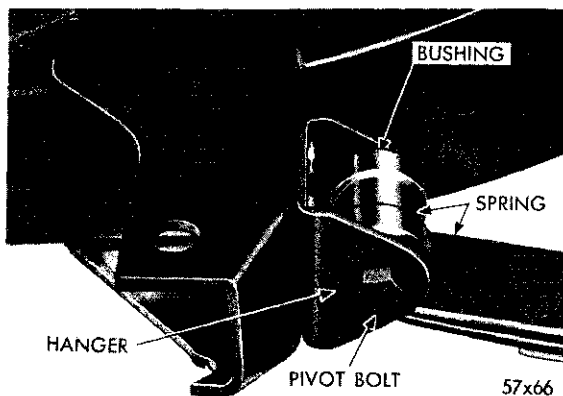
Fig. 5—Rear Springs Front Mounting
