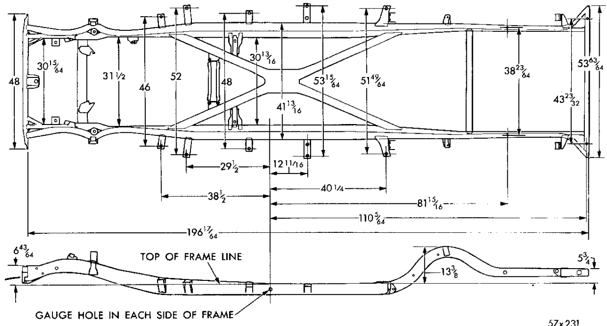
Fig. 1—Frame Dimensions, Windsor and New Yorker
