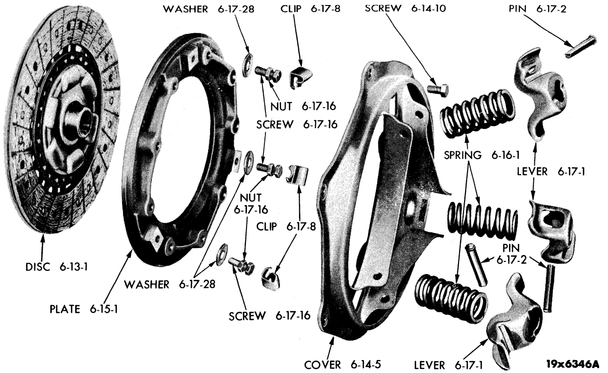
CLUTCH (TYPE 1)
