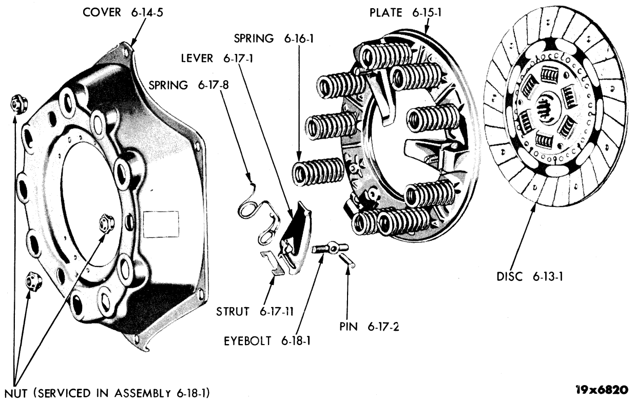
CLUTCH (TYPE 2)
