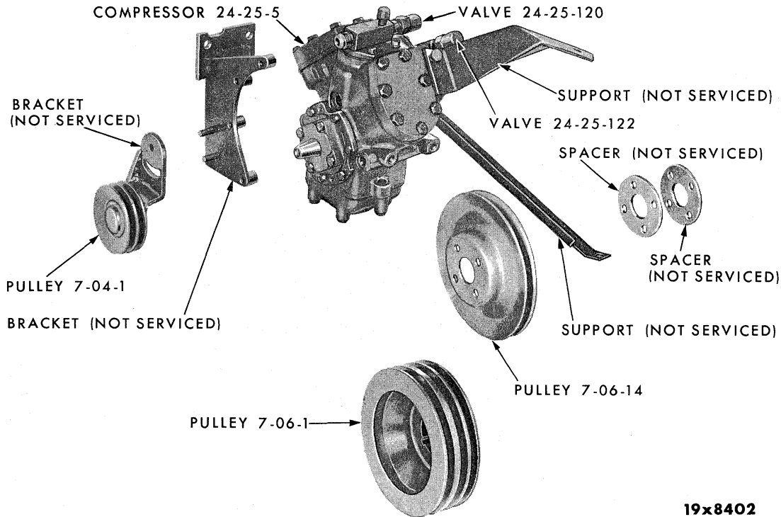
AIR CONDITIONING COMPRESSOR, PULLEY AND BRACKETS - PLYMOUTH LP1-2, DODGE LD1-2-3
