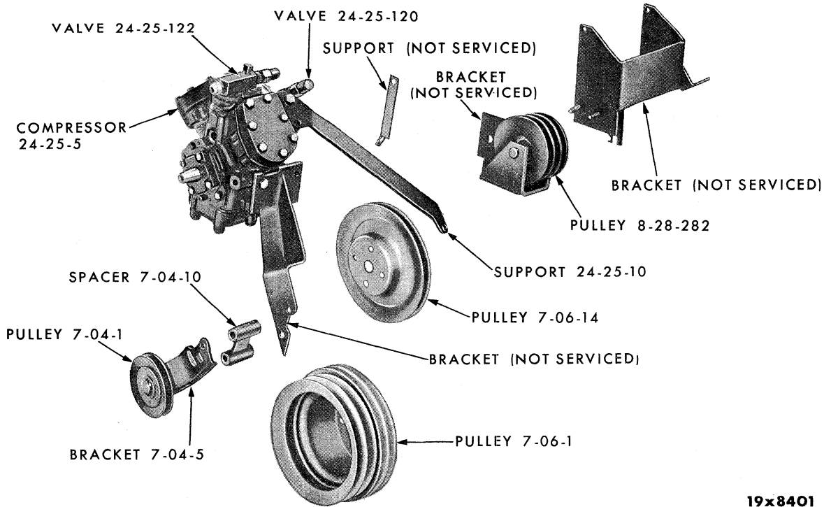
AIR CONDITIONING COMPRESSOR, PULLEY, AND BRACKETS - PLYMOUTH LP2 FURY (WITH 350 CU. IN. ENGINE), DODGE LD2-D500, DESOTO LS1-2-3
