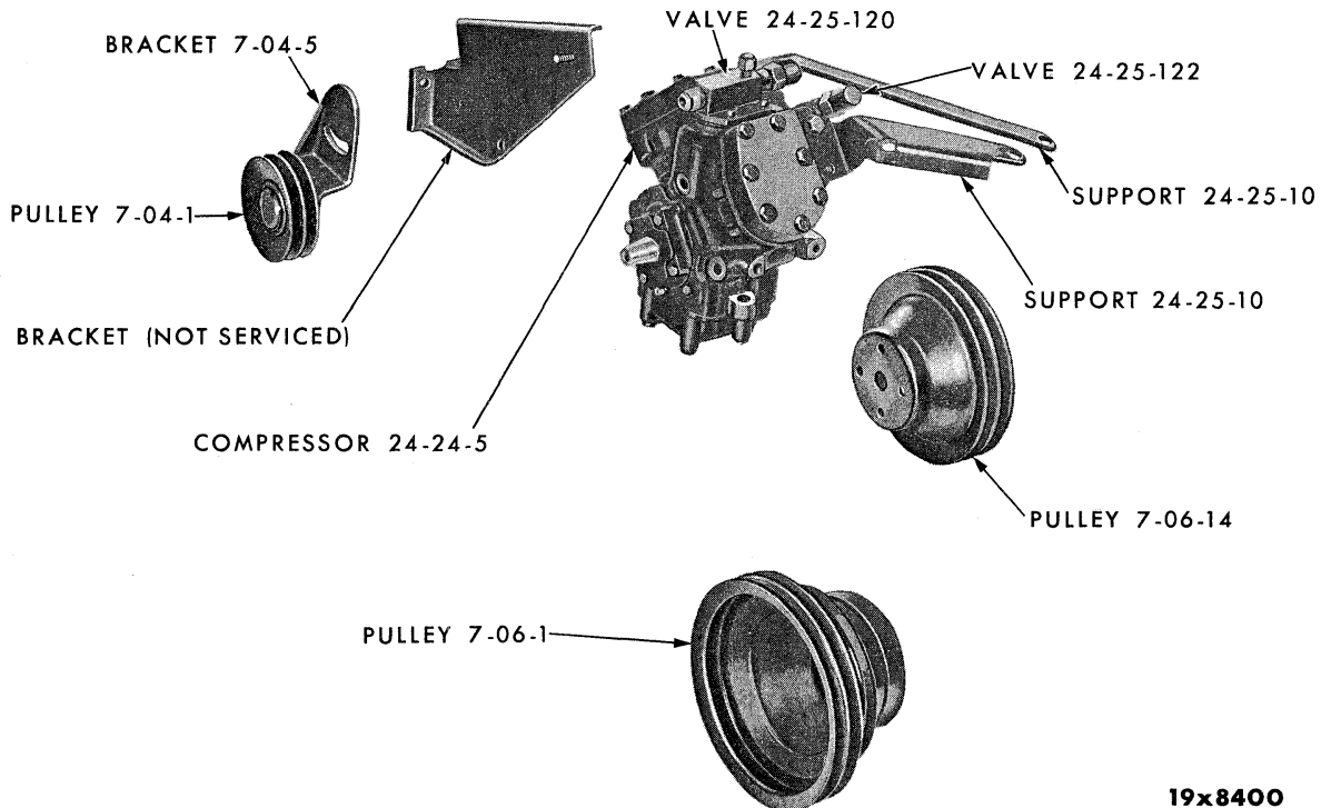
AIR CONDITIONING COMPRESSOR, PULLEY AND BRACKETS - CHRYSLER LC1-2-3, IMPERIAL LY1
